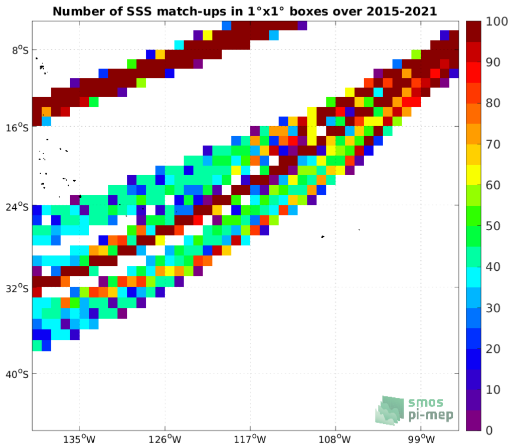
Figure 4: Number of SSS match-ups between TSG (LEGOS-DM) SSS and the SMAP SSS L3 v5.0 - Monthly (JPL) SSS product for the OTT zone Pi-MEP region over 1°×1° boxes and for the full satellite product period.
