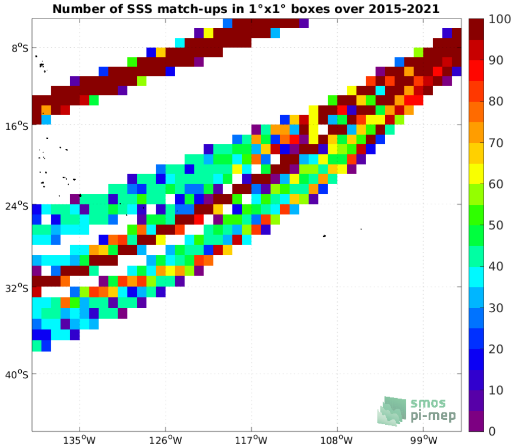
Figure 4: Number of SSS match-ups between TSG (LEGOS-DM) SSS and the SMAP SSS L3 v5.0 - Monthly (JPL) SSS product for the OTT zone Pi-MEP region over 1^\circ \times 1^\circ boxes and for the full satellite product period.
