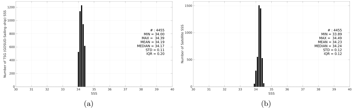
Figure 3: Histograms of SSS from TSG (GOSUD-Sailing-ship) (a) and SMAP SSS L3 v5.0 - Monthly (JPL) (b) considering all match-up pairs per bins of 0.1 over the OTT zone Pi-MEP region and for the full satellite product period.
