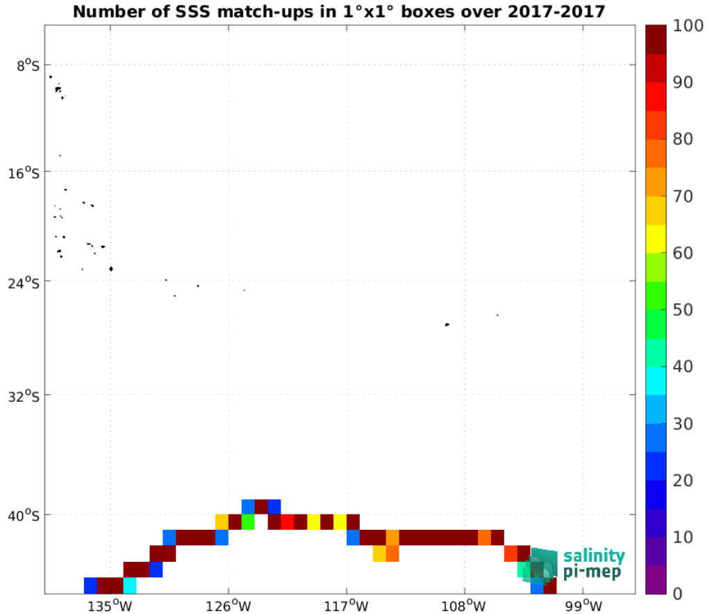
Figure 5: Number of SSS match-ups between TSG (GOSUD-Sailing-ship) SSS and the SMAP SSS L3 v5.0 - Monthly (JPL) SSS product for the OTT zone Pi-MEP region over 1^\circ \times 1^\circ boxes and for the full satellite product period.
