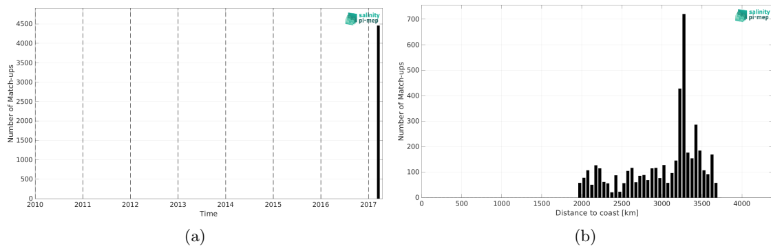
Figure 2: Number of match-ups between TSG (GOSUD-Sailing-ship) and SMAP SSS L3 v5.0 - Monthly (JPL) SSS as a function of time (a) and as function of the distance to coast (b) over the OTT zone Pi-MEP region and for the full satellite product period.
