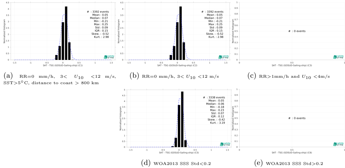
Figure 13: Normalized histogram of \Delta SSS (SMAP SSS L3 v5.0 - Monthly (JPL) - TSG (GOSUD-Sailing-ship)) for 5 different subdatasets corresponding to: RR=0 mm/h, 3 < U_{10} < 12 m/s, SST >5^{\circ}\text{C} , distance to coast > 800 km (a), RR=0 mm/h, 3 < U_{10} < 12 m/s (b), RR >1 mm/h and U_{10} < 4 m/s (c), WOA2013 SSS Std <0.2 (d), WOA2013 SSS Std >0.2 (e).
