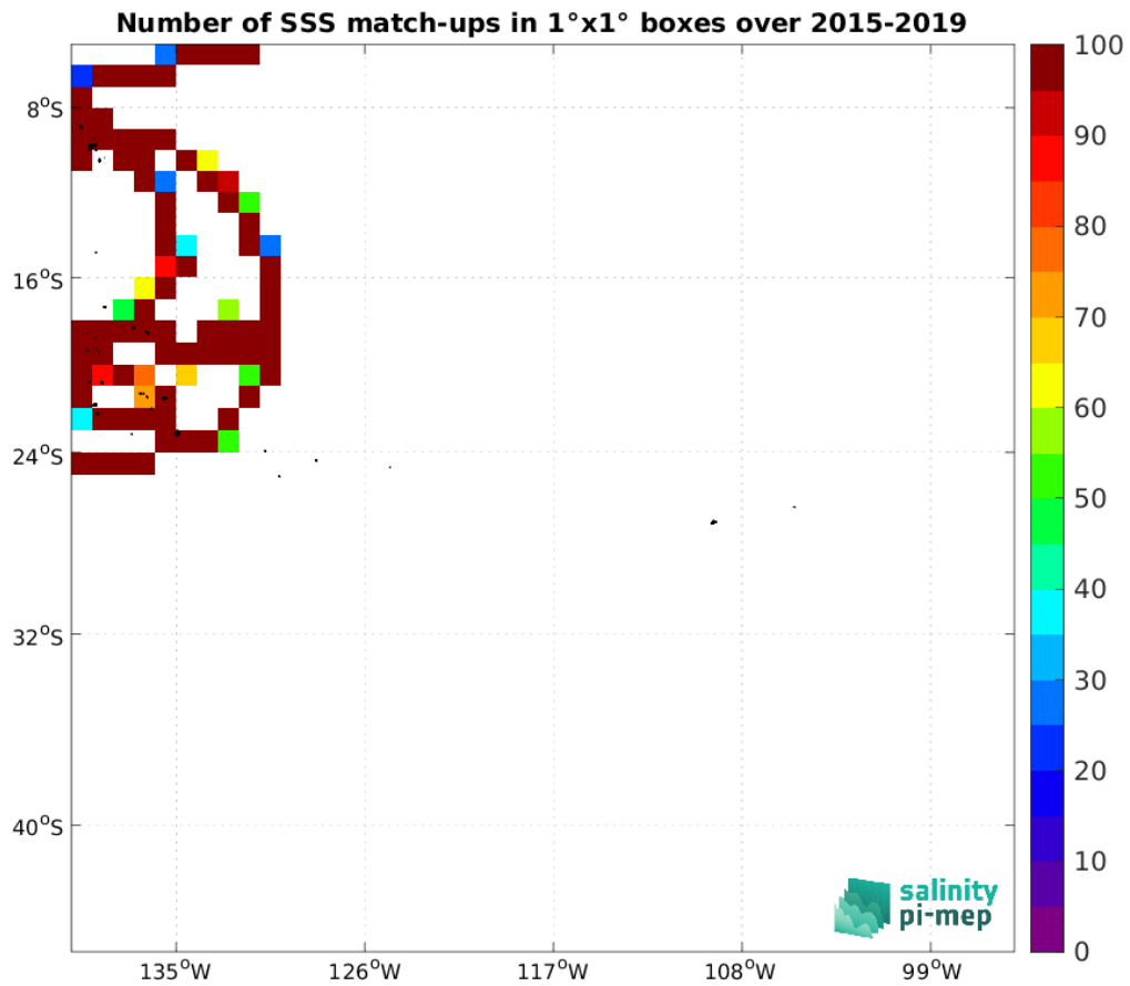
Figure 5: Number of SSS match-ups between TSG (GOSUD-Research-vessel) SSS and the SMAP SSS L3 v5.0 - Monthly (JPL) SSS product for the OTT zone Pi-MEP region over 1^\circ \times 1^\circ boxes and for the full satellite product period.
