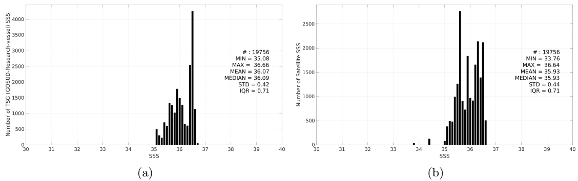
Figure 3: Histograms of SSS from TSG (GOSUD-Research-vessel) (a) and SMAP SSS L3 v5.0 - Monthly (JPL) (b) considering all match-up pairs per bins of 0.1 over the OTT zone Pi-MEP region and for the full satellite product period.
