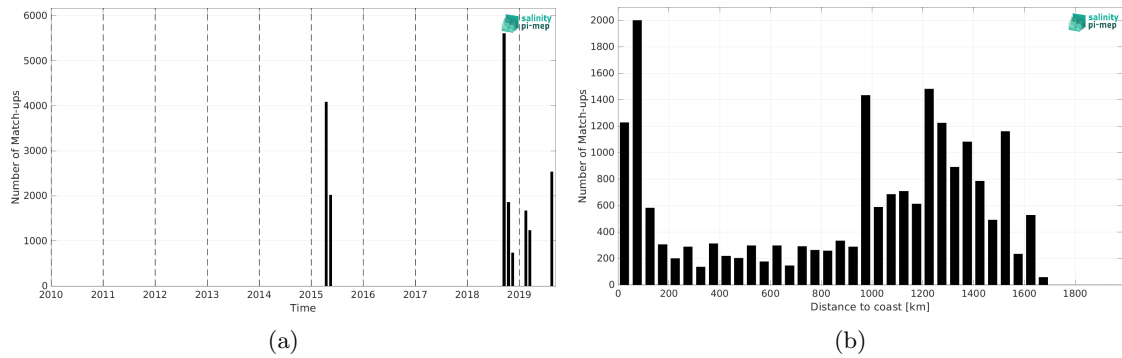
Figure 2: Number of match-ups between TSG (GOSUD-Research-vessel) and SMAP SSS L3 v5.0 - Monthly (JPL) SSS as a function of time (a) and as function of the distance to coast (b) over the OTT zone Pi-MEP region and for the full satellite product period.
