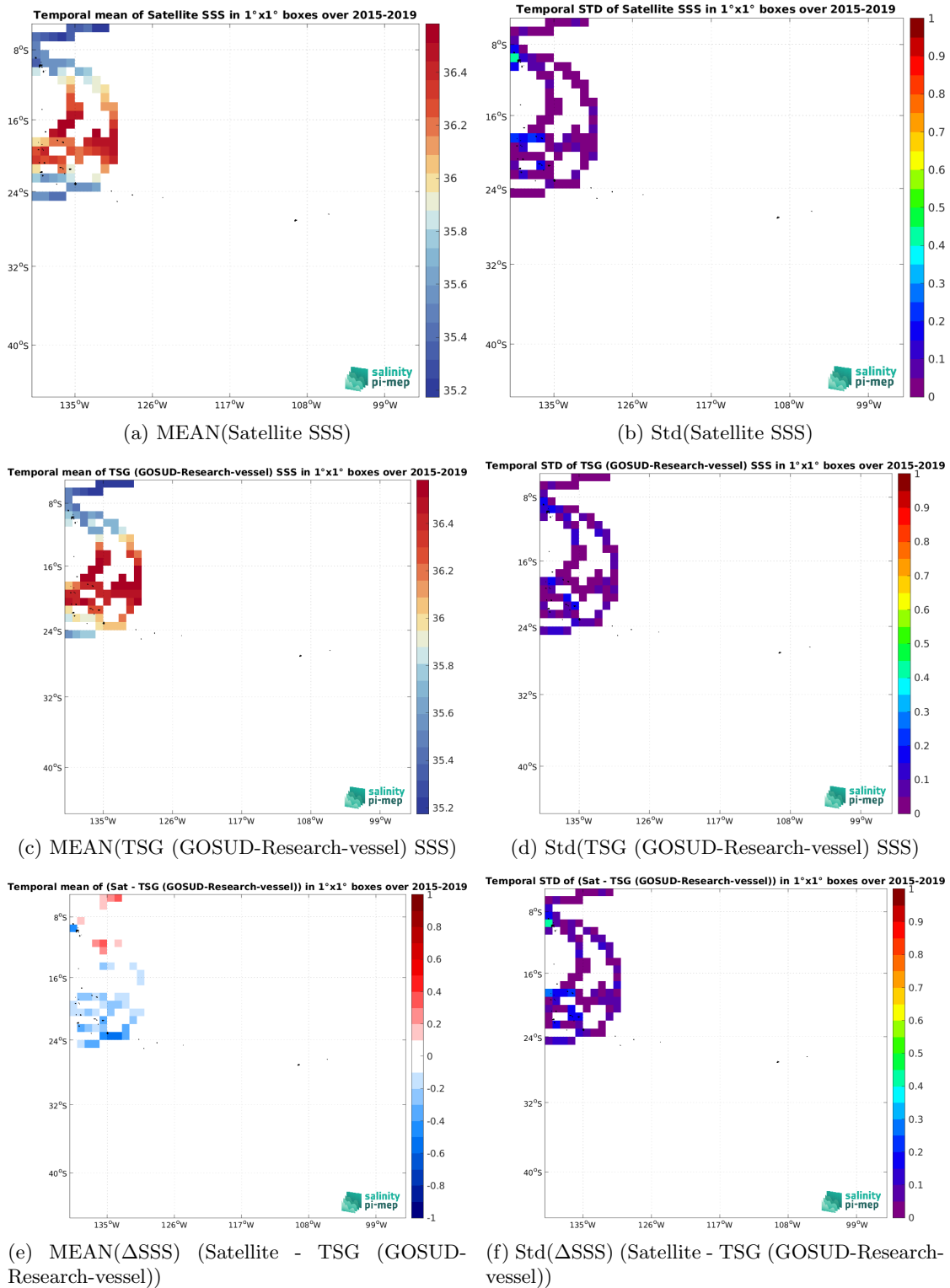
Figure 7: Temporal mean (left) and Std (right) of SSS from SMAP SSS L3 v5.0 - Monthly (JPL) (top), TSG (GOSUD-Research-vessel) (middle), and of \Delta SSS (Satellite - TSG (GOSUD-Research-vessel)). Only match-up pairs are used to generate these maps.
