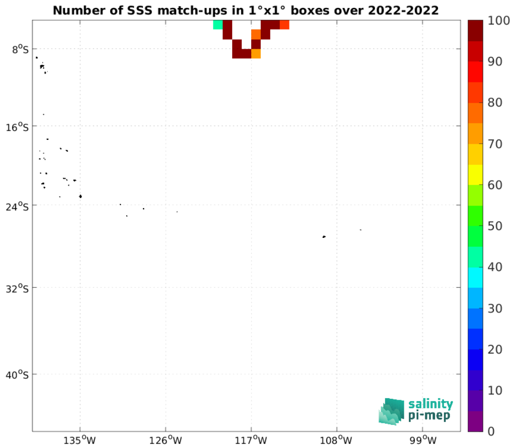
Figure 5: Number of SSS match-ups between Saildrone SSS and the SMAP SSS L3 v5.0 - Monthly (JPL) SSS product for the OTT zone Pi-MEP region over 1°x1° boxes and for the full satellite product period.
