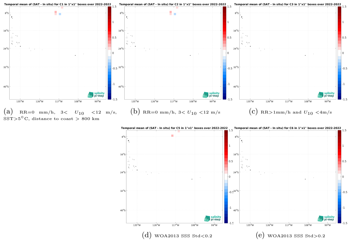
Figure 14: Temporal mean gridded over spatial boxes of size 1^\circ \times 1^\circ of \Delta SSS (SMAP SSS L3 v5.0 - Monthly (JPL) - Saildrone) for 5 different subdatasets corresponding to:RR=0 mm/h, 3 < U_{10} < 12 m/s, SST >5^\circ\text{C} , distance to coast > 800 km (a), RR=0 mm/h, 3 < U_{10} < 12 m/s (b), RR >1 mm/h and U_{10} < 4 m/s (c), WOA2013 SSS Std <0.2 (d), WOA2013 SSS Std >0.2 (e).
