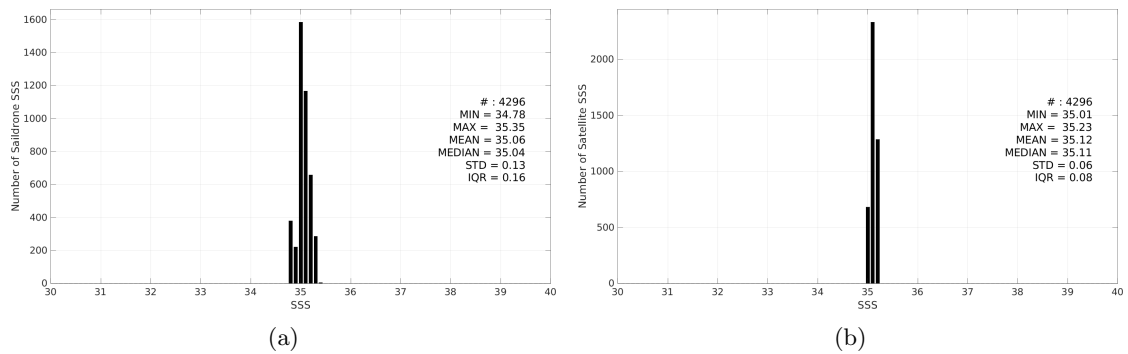
Figure 3: Histograms of SSS from Saildrone (a) and SMAP SSS L3 v5.0 - Monthly (JPL) (b) considering all match-up pairs per bins of 0.1 over the OTT zone Pi-MEP region and for the full satellite product period.
