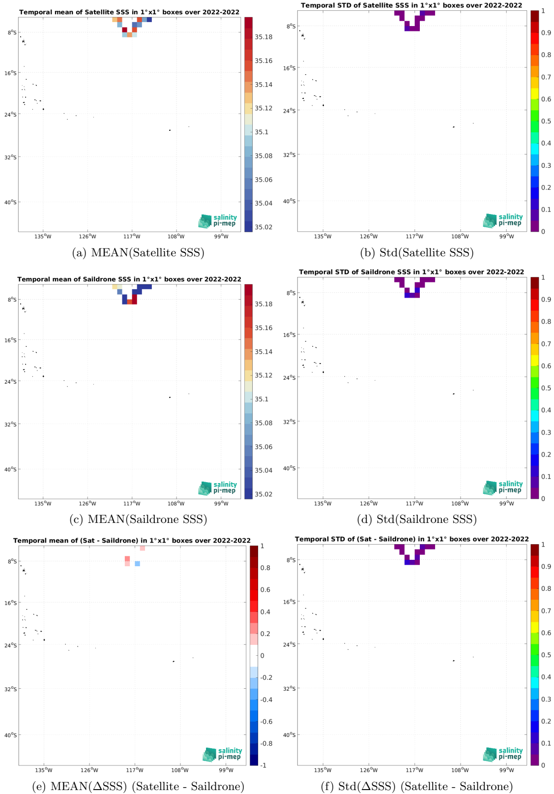
Figure 7: Temporal mean (left) and Std (right) of SSS from SMAP SSS L3 v5.0 - Monthly (JPL) (top), Saildrone (middle), and of \Delta SSS (Satellite - Saildrone). Only match-up pairs are used to generate these maps.
