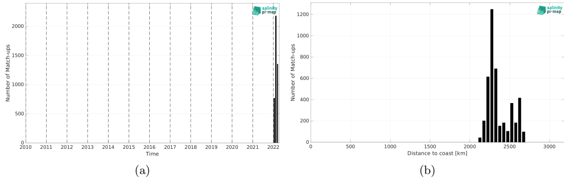
Figure 2: Number of match-ups between Saildrone and SMAP SSS L3 v5.0 - Monthly (JPL) SSS as a function of time (a) and as function of the distance to coast (b) over the OTT zone Pi-MEP region and for the full satellite product period.
