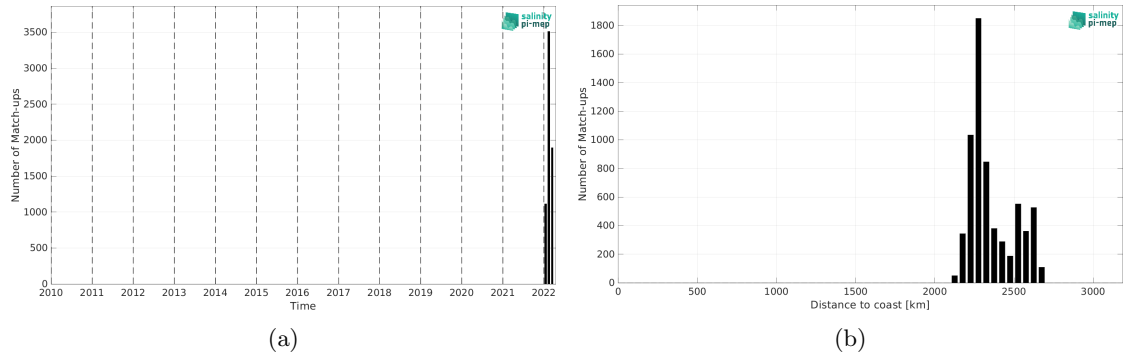
Figure 1: Number of match-ups between Saildrone and SMAP SSS L3 v5.0 - Monthly (JPL) SSS as a function of time (a) and as function of the distance to coast (b) over the OTT zone Pi-MEP region and for the full satellite product period.
