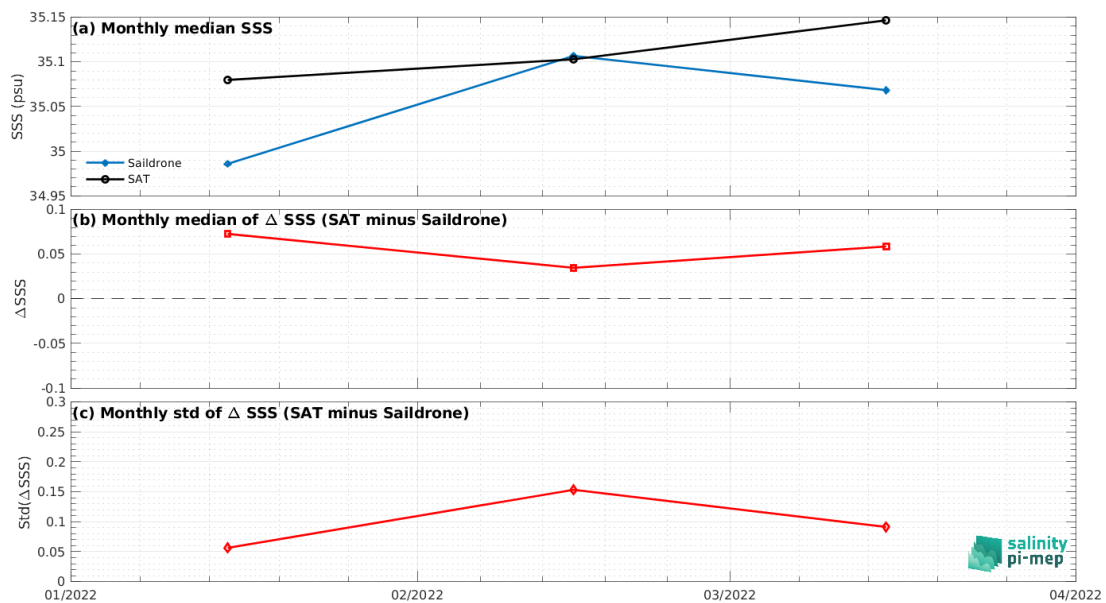
Figure 7: Time series of the monthly median SSS (top), median of \Delta SSS (Satellite - Sairdrone) and Std of \Delta SSS (Satellite - Sairdrone) over the OTT zone Pi-MEP region considering all match-ups collected by the Pi-MEP.
