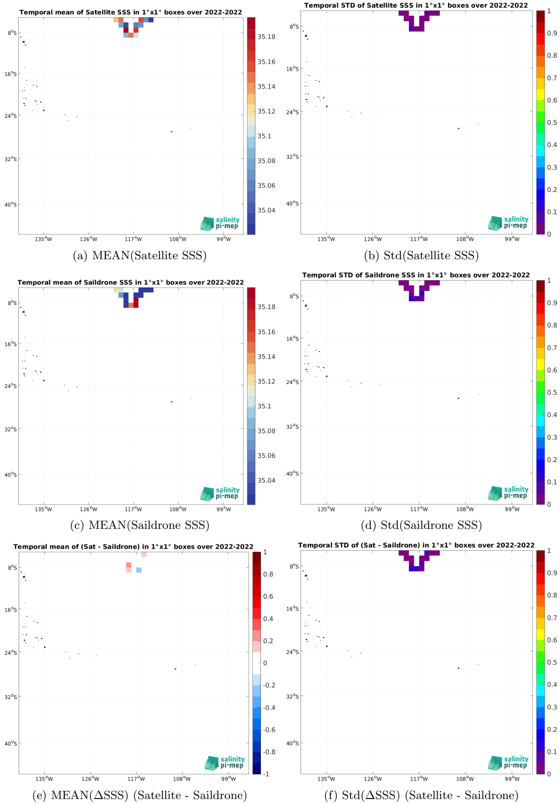
Figure 6: Temporal mean (left) and Std (right) of SSS from SMAP SSS L3 v5.0 - Monthly (JPL) (top), Saildrone (middle), and of \Delta SSS (Satellite - Saildrone). Only match-up pairs are used to generate these maps.
