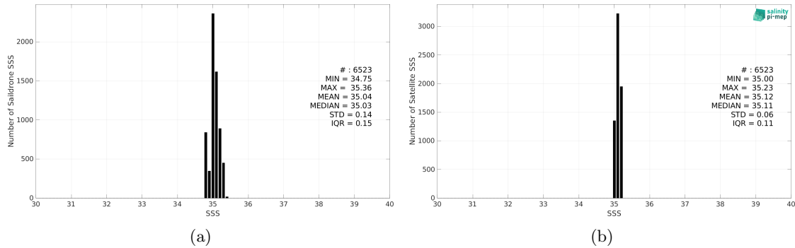
Figure 2: Histograms of SSS from Saildrone (a) and SMAP SSS L3 v5.0 - Monthly (JPL) (b) considering all match-up pairs per bins of 0.1 over the OTT zone Pi-MEP region and for the full satellite product period.
