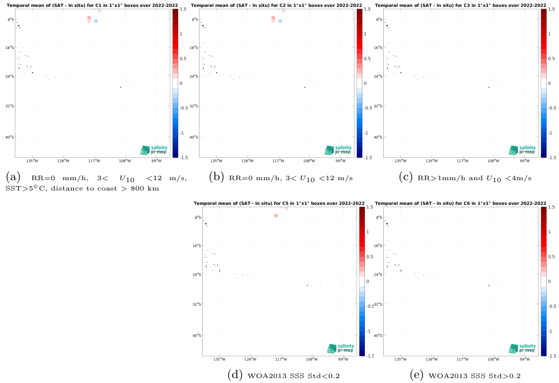
Figure 12: Temporal mean gridded over spatial boxes of size 1^\circ \times 1^\circ of \Delta SSS (SMAP SSS L3 v5.0 - Monthly (JPL) - Saildrone) for 5 different subdatasets corresponding to: RR=0 mm/h, 3 < U_{10} < 12 m/s, SST > 5^\circ\text{C} , distance to coast > 800 km (a), RR=0 mm/h, 3 < U_{10} < 12 m/s (b), RR > 1 mm/h and U_{10} < 4 m/s (c), WOA2013 SSS Std < 0.2 (d), WOA2013 SSS Std > 0.2 (e).
