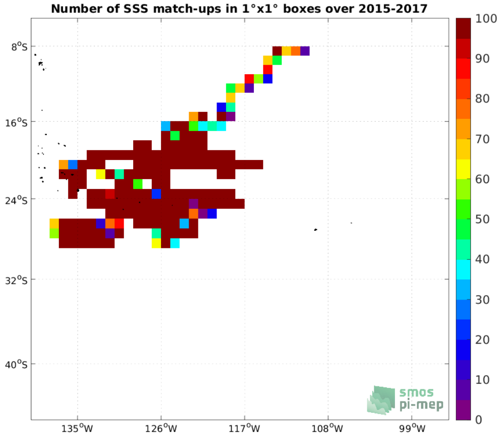
Figure 3: Number of SSS match-ups between Surface drifters SSS and the SMAP SSS L3 v5.0 - Monthly (JPL) SSS product for the OTT zone Pi-MEP region over 1^\circ \times 1^\circ boxes and for the full satellite product period.
