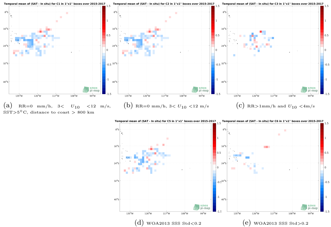
Figure 11: Temporal mean gridded over spatial boxes of size 1^\circ \times 1^\circ of \Delta SSS (SMAP SSS L3 v5.0 - Monthly (JPL) - Surface drifters) for 5 different subdatasets corresponding to:RR=0 mm/h, 3 < U_{10} < 12 m/s, SST >5^\circ\text{C} , distance to coast > 800 km (a), RR=0 mm/h, 3 < U_{10} < 12 m/s (b), RR >1 mm/h and U_{10} < 4 m/s (c), WOA2013 SSS Std <0.2 (d), WOA2013 SSS Std >0.2 (e).
