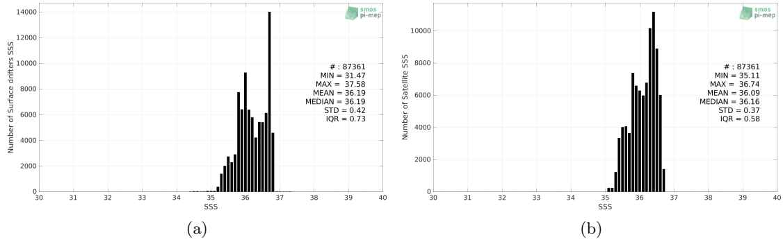
Figure 2: Histograms of SSS from Surface drifters (a) and SMAP SSS L3 v5.0 - Monthly (JPL) (b) considering all match-up pairs per bins of 0.1 over the OTT zone Pi-MEP region and for the full satellite product period.
