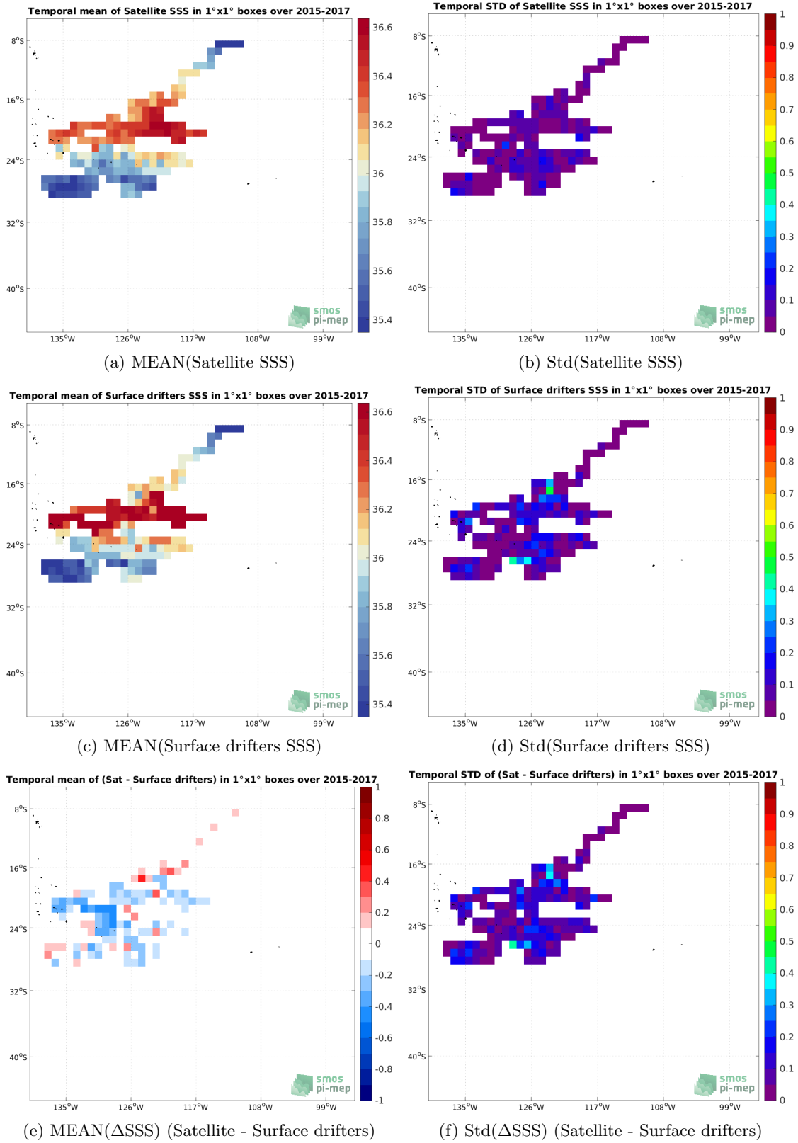
Figure 5: Temporal mean (left) and Std (right) of SSS from SMAP SSS L3 v5.0 - Monthly (JPL) (top), Surface drifters (middle), and of \Delta SSS (Satellite - Surface drifters). Only match-up pairs are used to generate these maps.
