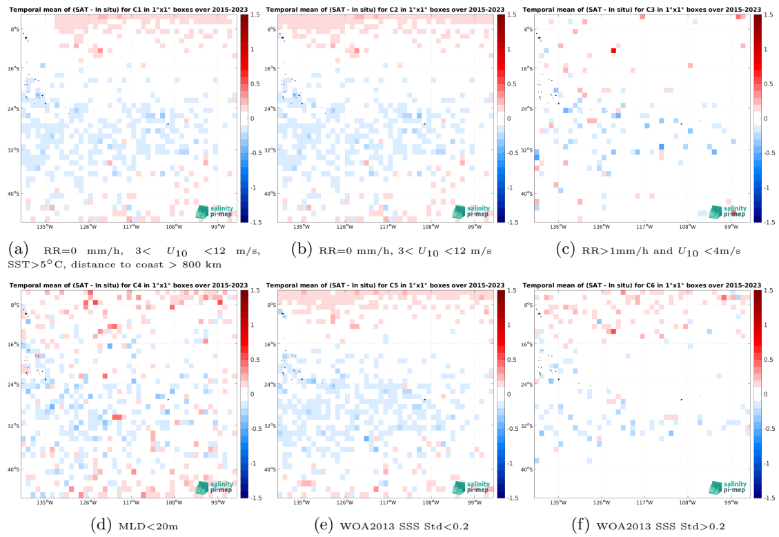
Figure 12: Temporal mean gridded over spatial boxes of size 1^\circ \times 1^\circ of \Delta SSS (SMAP SSS L3 v5.0 - Monthly (JPL) - Argo) for 6 different subdatasets corresponding to:RR=0 mm/h, 3 < U_{10} < 12 m/s, SST >5^\circ C, distance to coast > 800 km (a), RR=0 mm/h, 3 < U_{10} < 12 m/s (b), RR >1 mm/h and U_{10} < 4 m/s (c),MLD <20 m (d),WOA2013 SSS Std <0.2 (e),WOA2013 SSS Std >0.2 (f).
