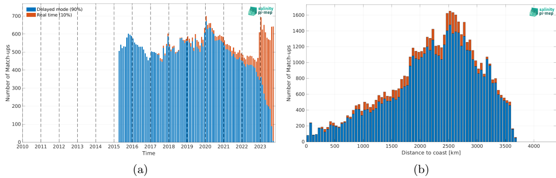
Figure 1: Number of match-ups between Argo and SMAP SSS L3 v5.0 - Monthly (JPL) SSS as a function of time (a) and as function of the distance to coast (b) over the OTT zone Pi-MEP region and for the full satellite product period.
