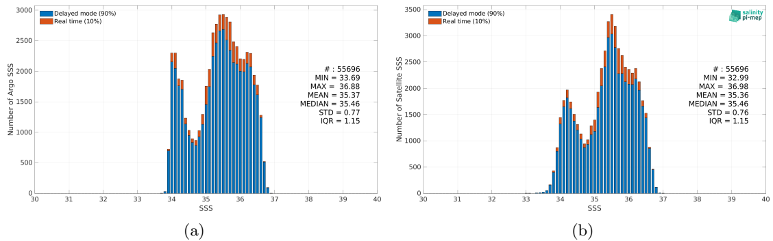
Figure 2: Histograms of SSS from Argo (a) and SMAP SSS L3 v5.0 - Monthly (JPL) (b) considering all match-up pairs per bins of 0.1 over the OTT zone Pi-MEP region and for the full satellite product period.
