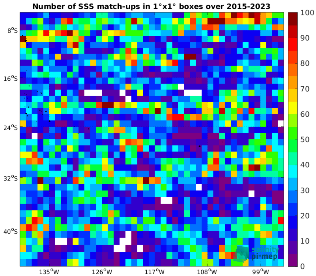
Figure 4: Number of SSS match-ups between Argo SSS and the SMAP SSS L3 v5.0 - Monthly (JPL) SSS product for the OTT zone Pi-MEP region over 1°x1° boxes and for the full satellite product period.
