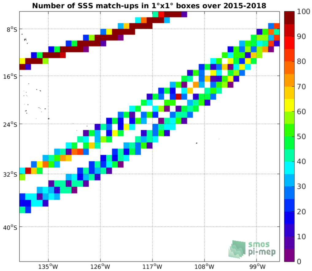
Figure 4: Number of SSS match-ups between TSG-LEGOS-DM SSS and the SMAP-L3-JPL-V4.2-8DAY-RUNNING-60KM SSS product for the OTT zone Pi-MEP region over 1°x1° boxes and for the full satellite product period.
