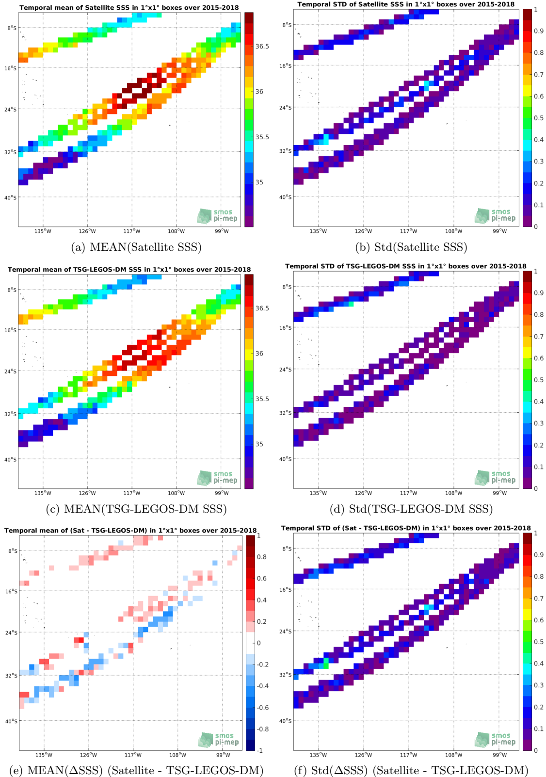
Figure 6: Temporal mean (left) and Std (right) of SSS from SMAP-L3-JPL-V4.2-8DAY-RUNNING-60KM (top), TSG-LEGOS-DM (middle), and of \Delta SSS (Satellite - TSG-LEGOS-DM). Only match-up pairs are used to generate these maps.
