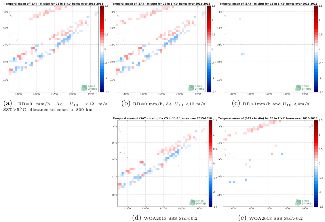
Figure 12: Temporal mean gridded over spatial boxes of size 1^\circ \times 1^\circ of \Delta SSS (SMAP-L3-JPL-V4.2-8DAY-RUNNING-60KM - TSG-LEGOS-DM) for 5 different subdatasets corresponding to:RR=0 mm/h, 3 < U_{10} < 12 m/s, SST >5^\circ\text{C} , distance to coast > 800 km (a), RR=0 mm/h, 3 < U_{10} < 12 m/s (b), RR >1 mm/h and U_{10} < 4 m/s (c), WOA2013 SSS Std <0.2 (d), WOA2013 SSS Std >0.2 (e).
