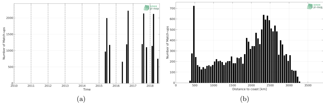
Figure 1: Number of match-ups between TSG-LEGOS-DM and SMAP-L3-JPL-V4.2-8DAY-RUNNING-60KM SSS as a function of time (a) and as function of the distance to coast (b) over the OTT zone Pi-MEP region and for the full satellite product period.
