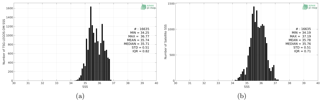
Figure 2: Histograms of SSS from TSG-LEGOS-DM (a) and SMAP-L3-JPL-V4.2-8DAY-RUNNING-60KM (b) considering all match-up pairs per bins of 0.1 over the OTT zone Pi-MEP region and for the full satellite product period.
