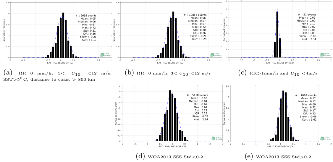
Figure 13: Normalized histogram of \Delta SSS (SMAP-L3-JPL-V4.2-8DAY-RUNNING-60KM - TSG-LEGOS-DM) for 5 different subdatasets corresponding to: RR=0 mm/h, 3 < U_{10} < 12 m/s, SST>5°C, distance to coast > 800 km (a), RR=0 mm/h, 3 < U_{10} < 12 m/s (b), RR>1mm/h and U_{10} < 4 m/s (c), WOA2013 SSS Std<0.2 (d), WOA2013 SSS Std>0.2 (e).
