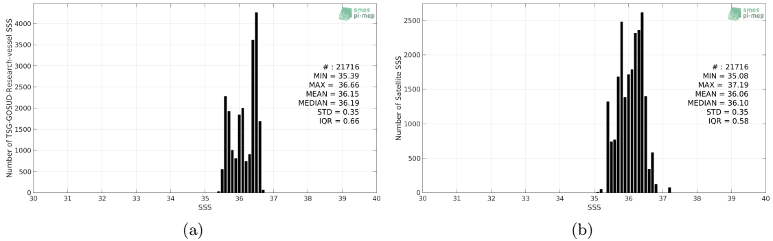
Figure 2: Histograms of SSS from TSG-GOSUD-Research-vessel (a) and SMAP-L3-JPL-V4.2-8DAY-RUNNING-60KM (b) considering all match-up pairs per bins of 0.1 over the OTT zone Pi-MEP region and for the full satellite product period.
