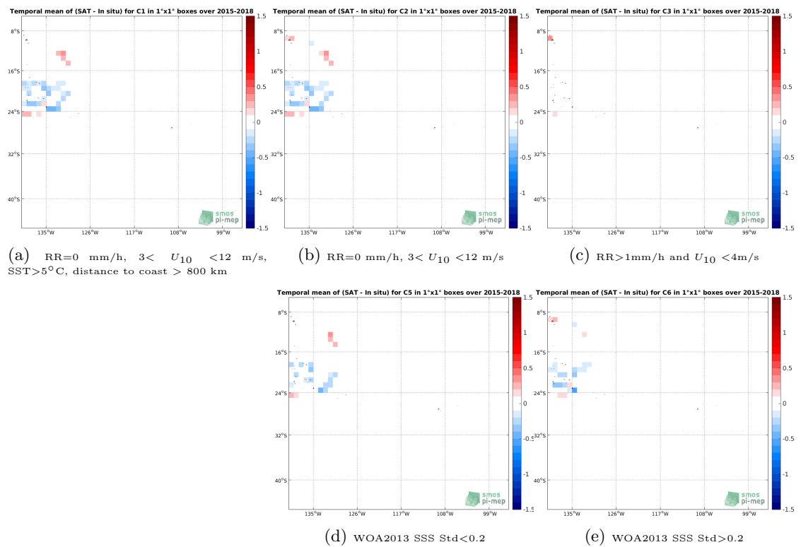
Figure 12: Temporal mean gridded over spatial boxes of size 1^\circ \times 1^\circ of \Delta SSS (SMAP-L3-JPL-V4.2-8DAY-RUNNING-60KM - TSG-GOSUD-Research-vessel) for 5 different subdatasets corresponding to:RR=0 mm/h, 3 < U_{10} < 12 m/s, SST >5^\circ C, distance to coast > 800 km (a), RR=0 mm/h, 3 < U_{10} < 12 m/s (b), RR >1 mm/h and U_{10} < 4 m/s (c), WOA2013 SSS Std <0.2 (d), WOA2013 SSS Std >0.2 (e).
