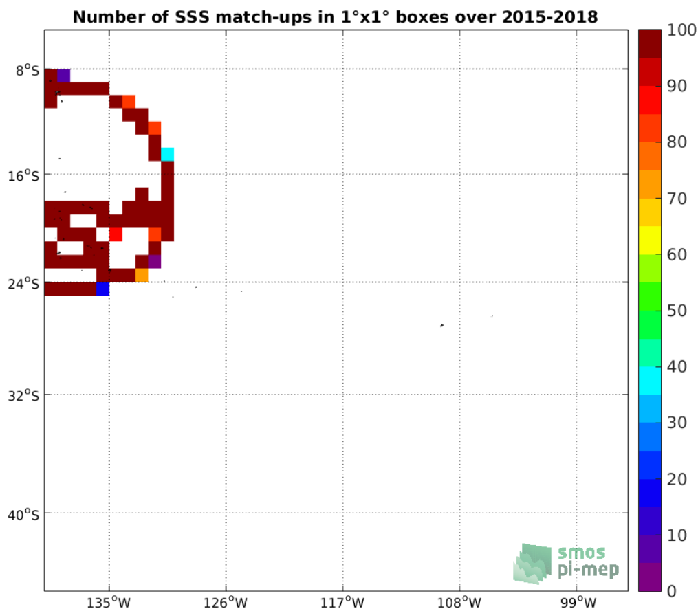
Figure 4: Number of SSS match-ups between TSG-GOSUD-Research-vessel SSS and the SMAP-L3-JPL-V4.2-8DAY-RUNNING-60KM SSS product for the OTT zone Pi-MEP region over 1°x1° boxes and for the full satellite product period.
