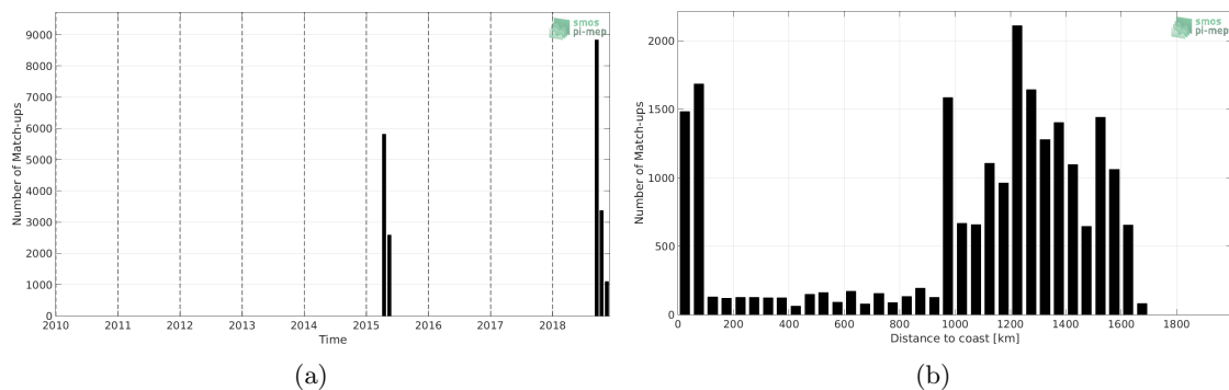
Figure 1: Number of match-ups between TSG-GOSUD-Research-vessel and SMAP-L3-JPL-V4.2-8DAY-RUNNING-60KM SSS as a function of time (a) and as function of the distance to coast (b) over the OTT zone Pi-MEP region and for the full satellite product period.
