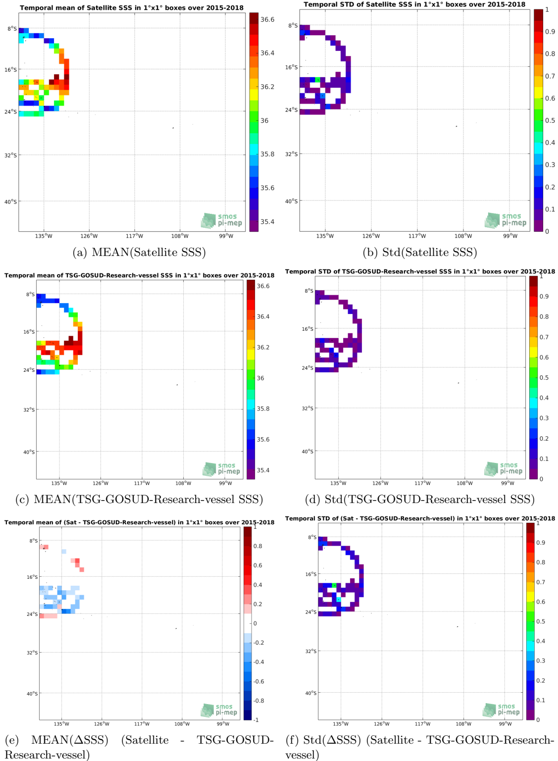
Figure 6: Temporal mean (left) and Std (right) of SSS from SMAP-L3-JPL-V4.2-8DAY-RUNNING-60KM (top), TSG-GOSUD-Research-vessel (middle), and of \Delta SSS (Satellite - TSG-GOSUD-Research-vessel). Only match-up pairs are used to generate these maps.
