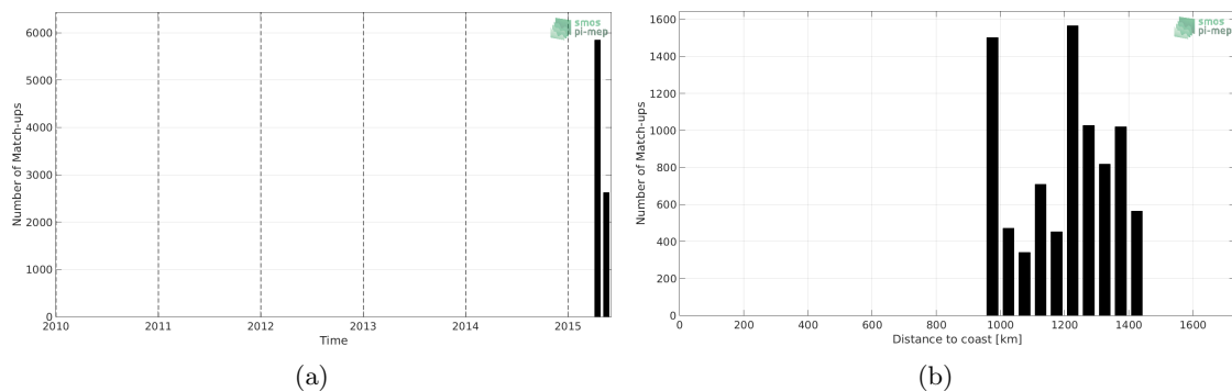
Figure 1: Number of match-ups between TSG-GOSUD-Research-vessel and SMAP-L3-JPL-V4.2-MONTHLY-60KM SSS as a function of time (a) and as function of the distance to coast (b) over the OTT zone Pi-MEP region and for the full satellite product period.
