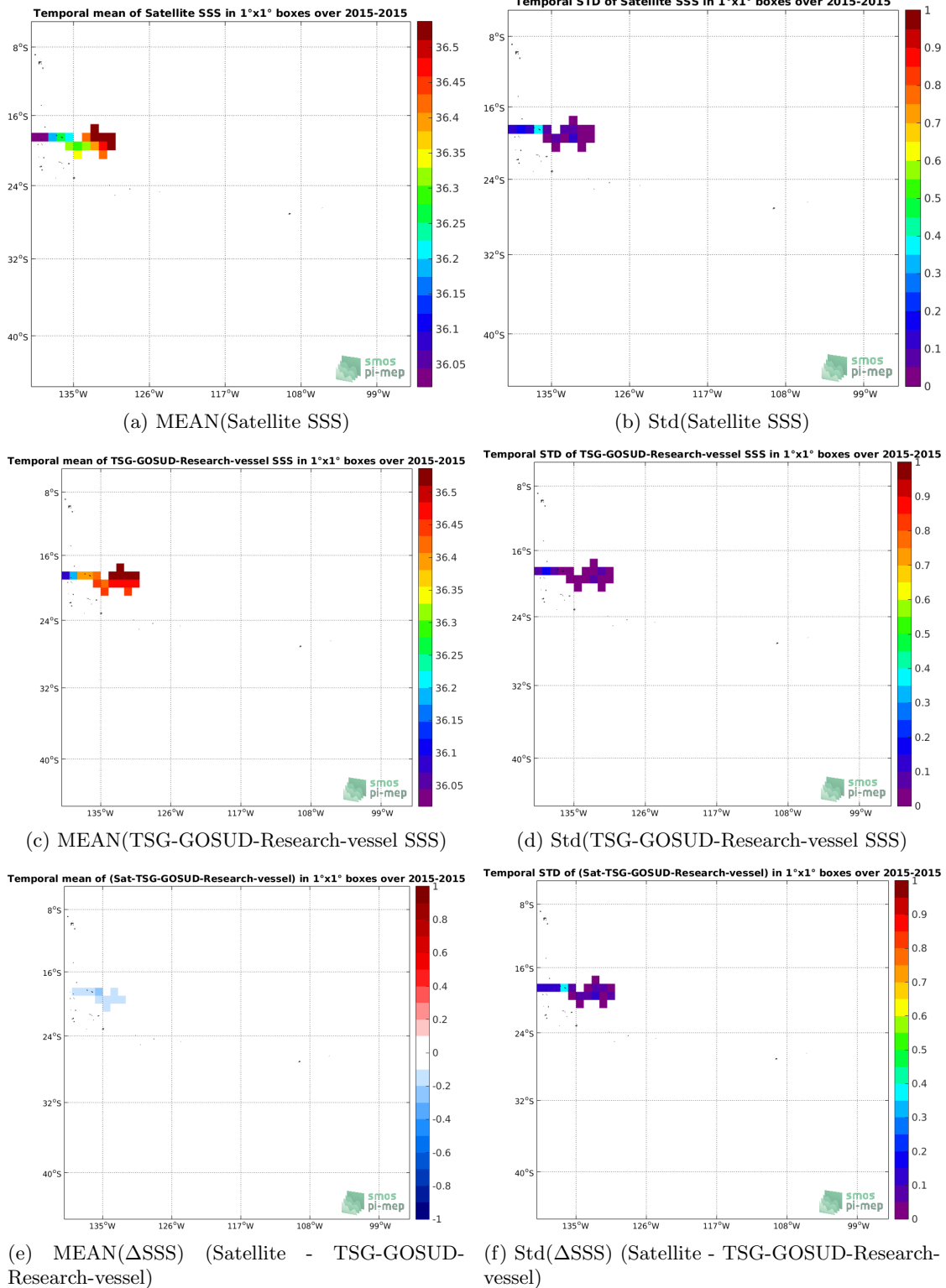
Figure 6: Temporal mean (left) and Std (right) of SSS from SMAP-L3-JPL-V4.2-MONTHLY-60KM (top), TSG-GOSUD-Research-vessel (middle), and of \Delta SSS (Satellite - TSG-GOSUD-Research-vessel). Only match-up pairs are used to generate these maps.
