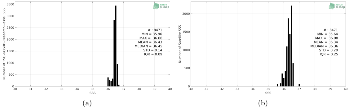
Figure 2: Histograms of SSS from TSG-GOSUD-Research-vessel (a) and SMAP-L3-JPL-V4.2-MONTHLY-60KM (b) considering all match-up pairs per bins of 0.1 over the OTT zone Pi-MEP region and for the full satellite product period.
