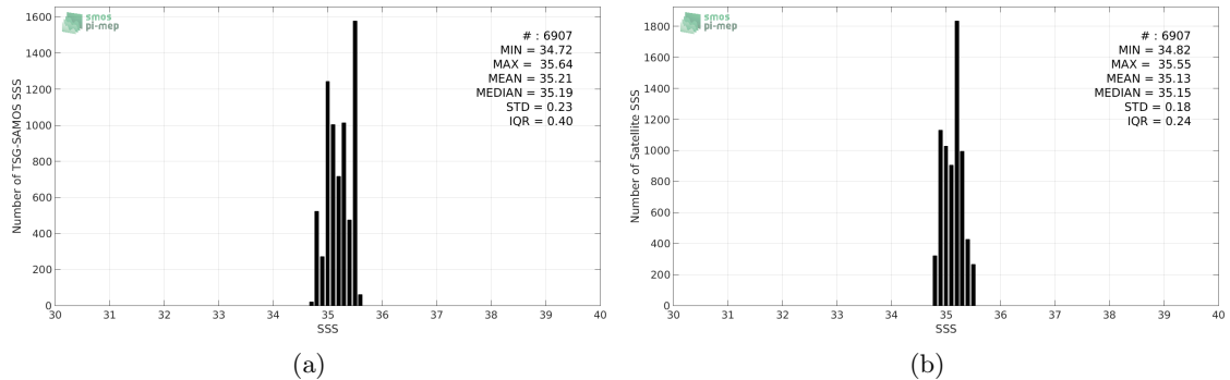
Figure 2: Histograms of SSS from TSG-SAMOS (a) and SMAP-L3-JPL-V4-8DAY-RUNNING-60KM (b) considering all match-up pairs per bins of 0.1 over the OTT zone Pi-MEP region and for the full satellite product period.
