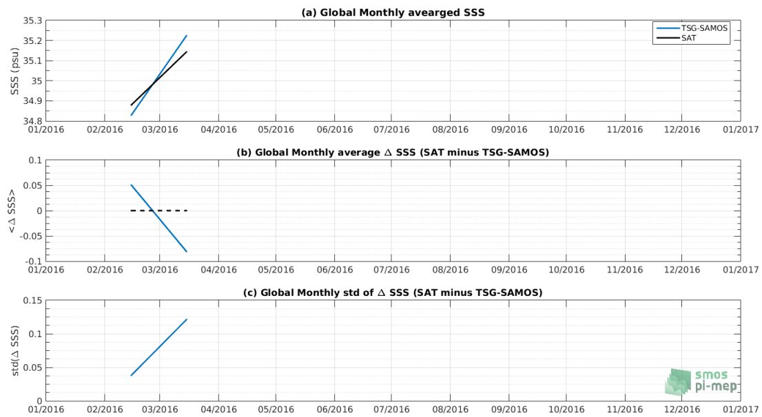
Figure 7: Time series of the monthly averaged mean SSS (top), mean \Delta SSS (Satellite - TSG-SAMOS) and STD of \Delta SSS (Satellite - TSG-SAMOS) over the OTT zone Pi-MEP region considering all match-ups collected by the Pi-MEP platform.
