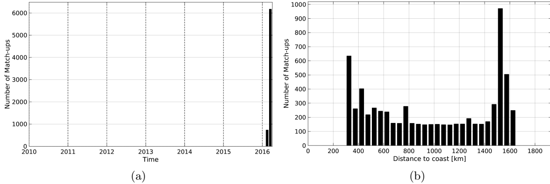
Figure 1: Number of match-ups between TSG-SAMOS and SMAP-L3-JPL-V4-8DAY-RUNNING-60KM SSS as a function of time (a) and as function of the distance to coast (b) over the OTT zone Pi-MEP region and for the full satellite product period.
