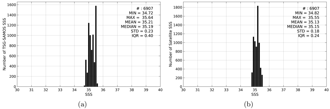
Figure 2: Histograms of SSS from TSG-SAMOS (a) and SMAP-L3-JPL-V4-8DAY-RUNNING-60KM (b) considering all match-up pairs per bins of 0.1 over the OTT zone Pi-MEP region and for the full satellite product period.
