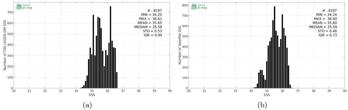
Figure 2: Histograms of SSS from TSG-LEGOS-DM (a) and SMAP-L3-JPL-V4-8DAY-RUNNING-60KM (b) considering all match-up pairs per bins of 0.1 over the OTT zone Pi-MEP region and for the full satellite product period.
