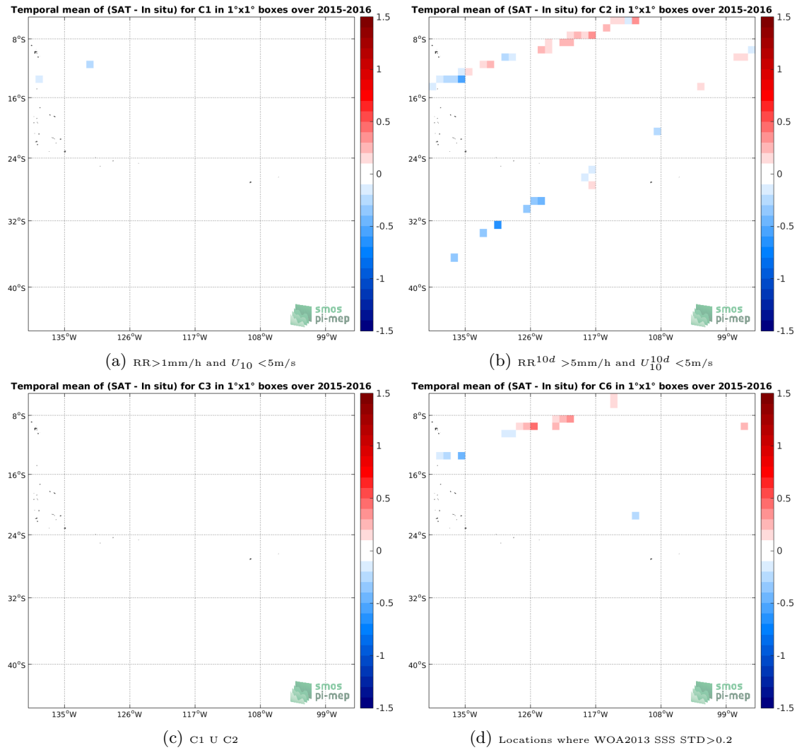
Figure 12: Temporal mean gridded over spatial boxes of size 1^\circ \times 1^\circ of \Delta SSS (SMAP-L3-JPL-V4-8DAY-RUNNING-60KM - TSG-LEGOS-DM) for 4 different subdatasets corresponding to: RR > 1mm/h and U_{10} < 5\text{m/s} (a), RR^{10d} > 5\text{mm/h} and U_{10}^{10d} < 5\text{m/s} (b), C1 U C2 (c), Locations where WOA2013 SSS STD > 0.2 (d).
