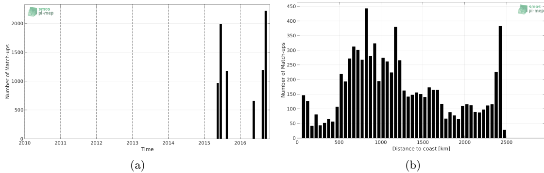
Figure 1: Number of match-ups between TSG-LEGOS-DM and SMAP-L3-JPL-V4-8DAY-RUNNING-60KM SSS as a function of time (a) and as function of the distance to coast (b) over the OTT zone Pi-MEP region and for the full satellite product period.
