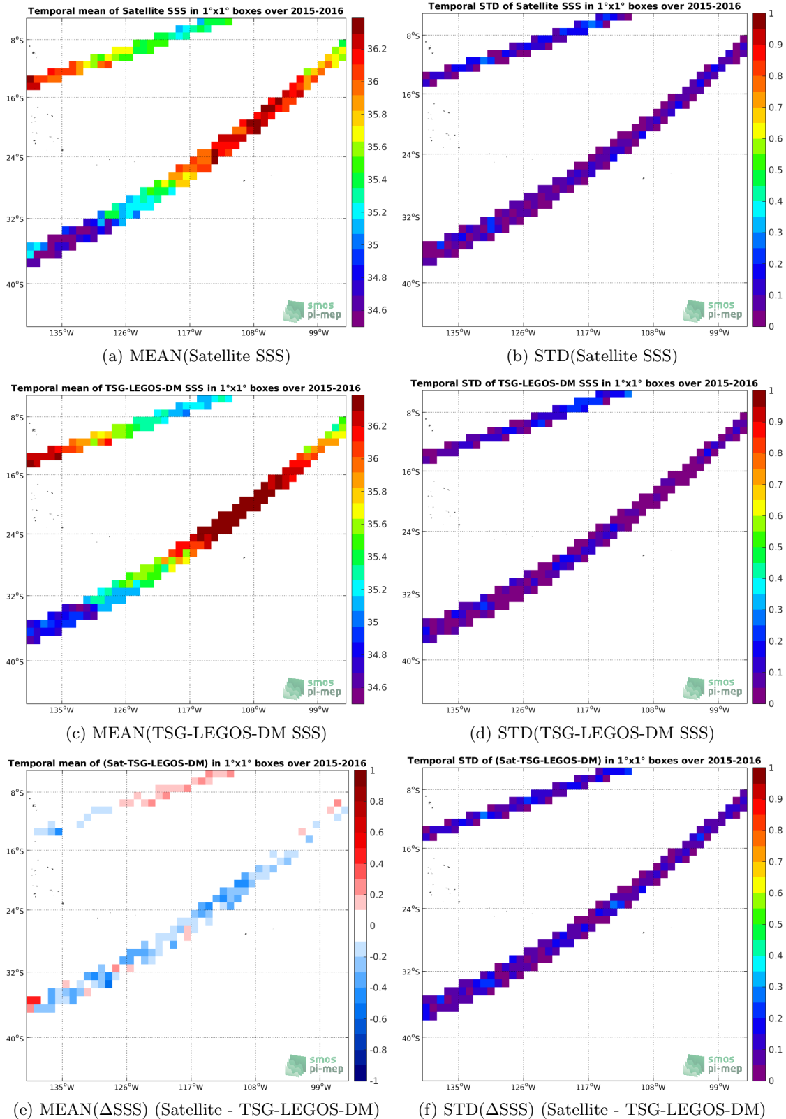
Figure 6: Temporal mean (left) and STD (right) of SSS from SMAP-L3-JPL-V4-8DAY-RUNNING-60KM (top), TSG-LEGOS-DM (middle), and of \Delta SSS (Satellite - TSG-LEGOS-DM). Only match-up pairs are used to generate these maps.
