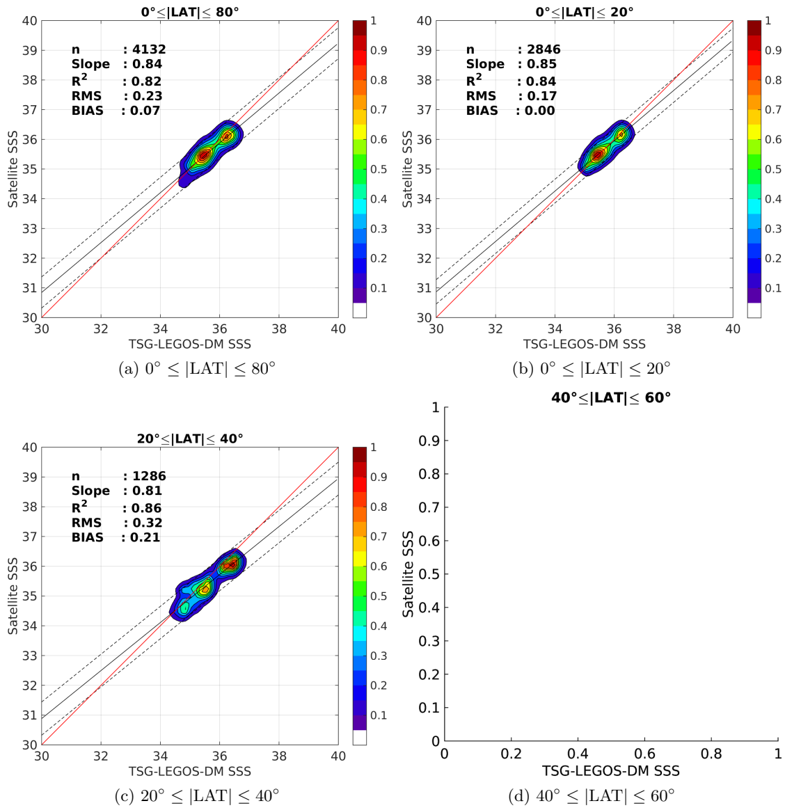
Figure 9: Contour maps of the concentration of SMAP-L3-JPL-V4-8DAY-RUNNING-60KM SSS (y-axis) versus TSG-LEGOS-DM SSS (x-axis) at match-up pairs for different latitude bands. For each plot, the red line shows x=y . The black thin and dashed lines indicate a linear fit through the data cloud and the \pm 95\% confidence levels, respectively. The number match-up pairs n , the slope and R^2 coefficient of the linear fit, the root mean square (RMS) and the mean bias between satellite and in situ data are indicated for each latitude band in each plots.
