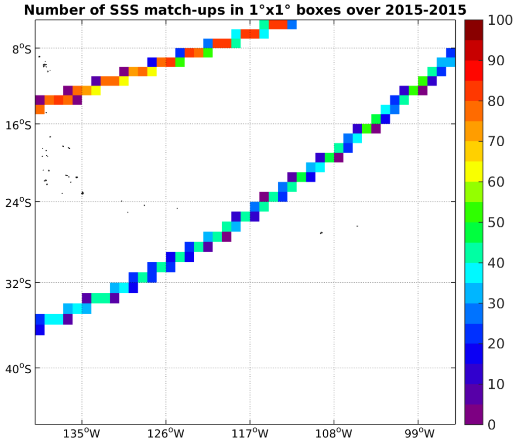
Figure 4: Number of SSS match-ups between TSG-LEGOS-DM SSS and the SMAP-L3-JPL-V4-8DAY-RUNNING-60KM SSS product for the OTT zone Pi-MEP region over 1°x1° boxes and for the full satellite product period.
