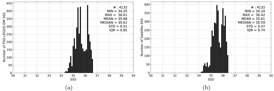
Figure 2: Histograms of SSS from TSG-LEGOS-DM (a) and SMAP-L3-JPL-V4-8DAY-RUNNING-60KM (b) considering all match-up pairs per bins of 0.1 over the OTT zone Pi-MEP region and for the full satellite product period.
