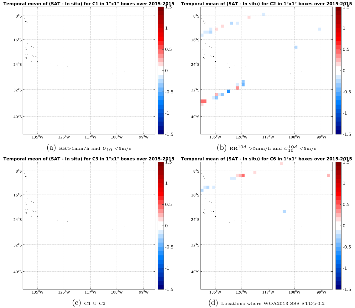
Figure 12: Temporal mean gridded over spatial boxes of size 1^\circ \times 1^\circ of \Delta SSS (SMAP-L3-JPL-V4-8DAY-RUNNING-60KM - TSG-LEGOS-DM) for 4 different subdatasets corresponding to: RR > 1\text{mm/h} and U_{10} < 5\text{m/s} (a), RR^{10d} > 5\text{mm/h} and U_{10}^{10d} < 5\text{m/s} (b), C1 U C2 (c), Locations where WOA2013 SSS STD > 0.2 (d).
