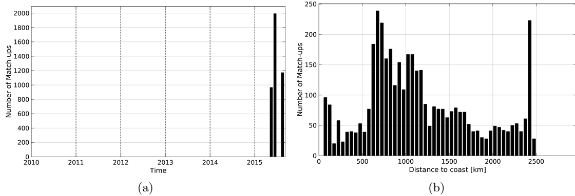
Figure 1: Number of match-ups between TSG-LEGOS-DM and SMAP-L3-JPL-V4-8DAY-RUNNING-60KM SSS as a function of time (a) and as function of the distance to coast (b) over the OTT zone Pi-MEP region and for the full satellite product period.
