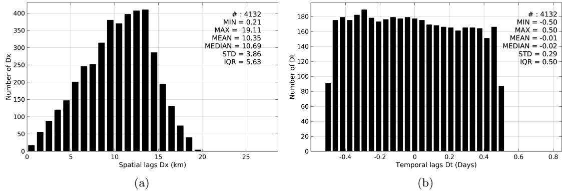
Figure 5: Histograms of the spatial (a) and temporal (b) lags between the time of the TSG-LEGOS-DM measurements and the date of the corresponding SMAP-L3-JPL-V4-8DAY-RUNNING-60KM SSS product.
