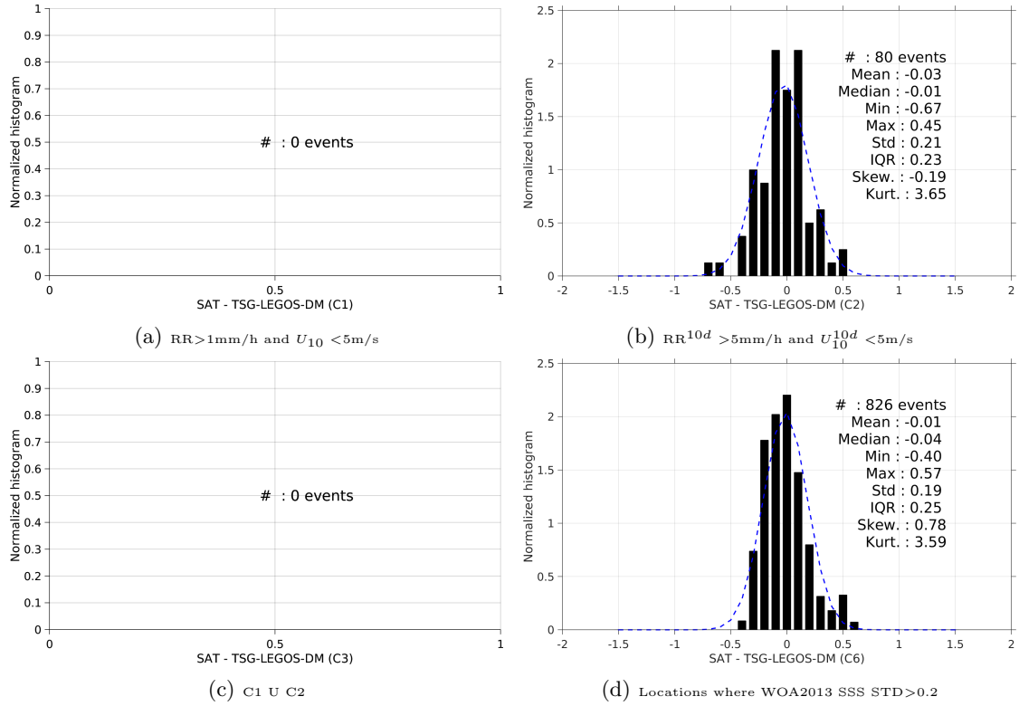
Figure 13: Normalized histogram of \Delta\text{SSS} (SMAP-L3-JPL-V4-8DAY-RUNNING-60KM - TSG-LEGOS-DM) for 6 different subdatasets corresponding to: RR > 1\text{mm/h} and U_{10} < 5\text{m/s} (a), RR^{10d} > 5\text{mm/h} and U_{10}^{10d} < 5\text{m/s} (b), C1 \cup C2 (c), Locations where WOA2013 SSS STD > 0.2 (d).
