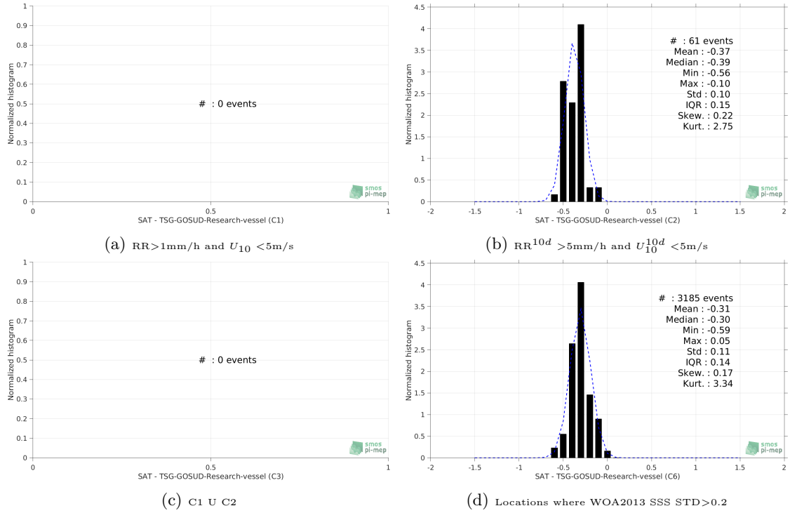
Figure 13: Normalized histogram of \Delta\text{SSS} (SMAP-L3-JPL-V4-8DAY-RUNNING-60KM - TSG-GOSUD-Research-vessel) for 6 different subdatasets corresponding to: RR > 1\text{mm/h} and U_{10} < 5\text{m/s} (a), RR^{10d} > 5\text{mm/h} and U_{10}^{10d} < 5\text{m/s} (b), C1 \cup C2 (c), Locations where WOA2013 SSS STD > 0.2 (d).
