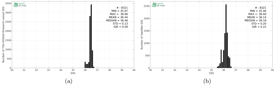
Figure 2: Histograms of SSS from TSG-GOSUD-Research-vessel (a) and SMAP-L3-JPL-V4-8DAY-RUNNING-60KM (b) considering all match-up pairs per bins of 0.1 over the OTT zone Pi-MEP region and for the full satellite product period.
