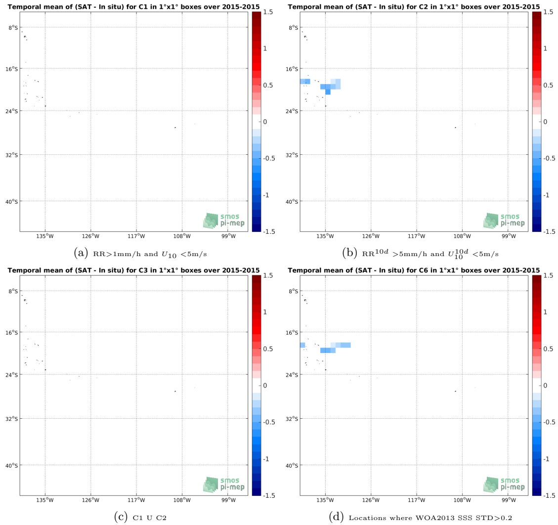
Figure 12: Temporal mean gridded over spatial boxes of size 1^\circ \times 1^\circ of \Delta SSS (SMAP-L3-JPL-V4-8DAY-RUNNING-60KM - TSG-GOSUD-Research-vessel) for 4 different subdatasets corresponding to: RR > 1\text{mm/h} and U_{10} < 5\text{m/s} (a), RR^{10d} > 5\text{mm/h} and U_{10}^{10d} < 5\text{m/s} (b), C1 U C2 (c), Locations where WOA2013 SSS STD > 0.2 (d).
