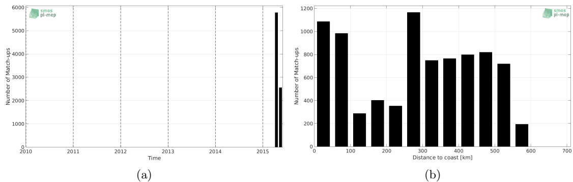
Figure 1: Number of match-ups between TSG-GOSUD-Research-vessel and SMAP-L3-JPL-V4-8DAY-RUNNING-60KM SSS as a function of time (a) and as function of the distance to coast (b) over the OTT zone Pi-MEP region and for the full satellite product period.
