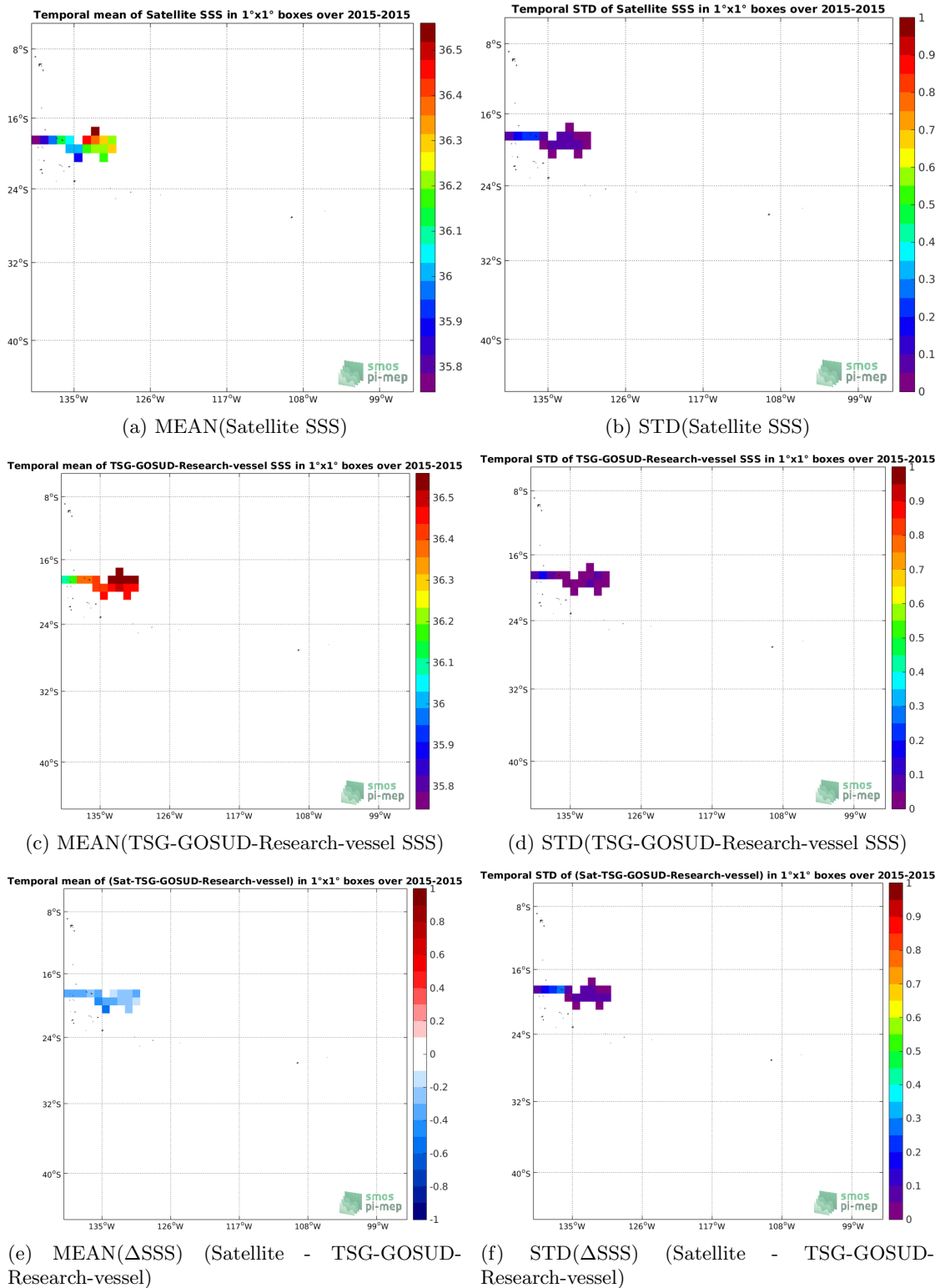
Figure 6: Temporal mean (left) and STD (right) of SSS from SMAP-L3-JPL-V4-8DAY-RUNNING-60KM (top), TSG-GOSUD-Research-vessel (middle), and of \Delta SSS (Satellite - TSG-GOSUD-Research-vessel). Only match-up pairs are used to generate these maps.
