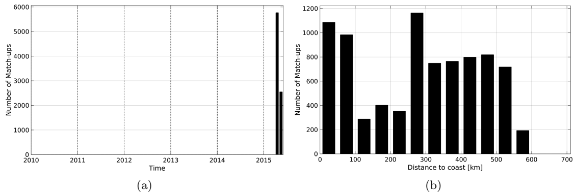
Figure 1: Number of match-ups between TSG-GOSUD-Research-vessel and SMAP-L3-JPL-V4-8DAY-RUNNING-60KM SSS as a function of time (a) and as function of the distance to coast (b) over the OTT zone Pi-MEP region and for the full satellite product period.
