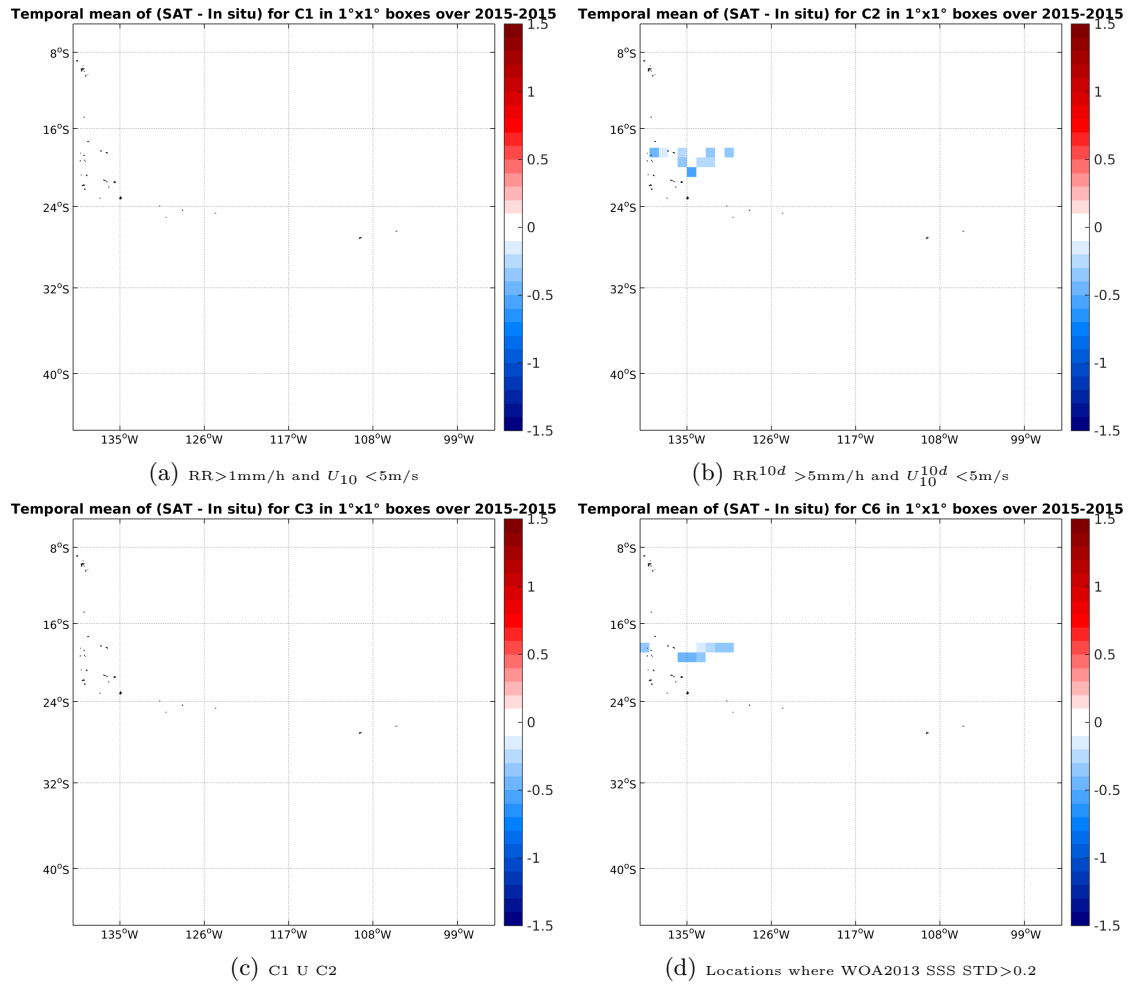
Figure 12: Temporal mean gridded over spatial boxes of size 1°x1° of \Delta SSS (SMAP-L3-JPL-V4-8DAY-RUNNING-60KM - TSG-GOSUD-Research-vessel) for 4 different subdatasets corresponding to: RR > 1\text{mm/h} and U_{10} < 5\text{m/s} (a), RR^{10d} > 5\text{mm/h} and U_{10}^{10d} < 5\text{m/s} (b), C1 U C2 (c), Locations where WOA2013 SSS STD > 0.2 (d).
