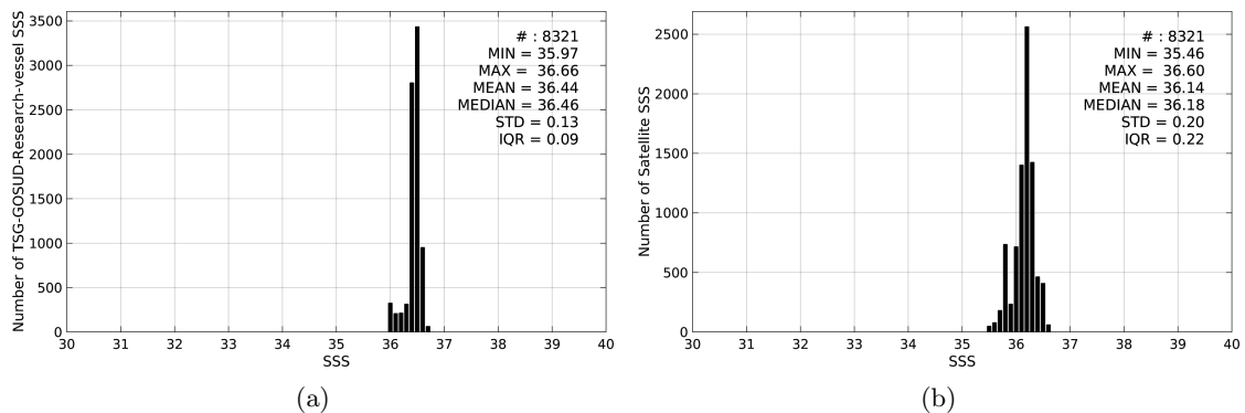
Figure 2: Histograms of SSS from TSG-GOSUD-Research-vessel (a) and SMAP-L3-JPL-V4-8DAY-RUNNING-60KM (b) considering all match-up pairs per bins of 0.1 over the OTT zone Pi-MEP region and for the full satellite product period.
