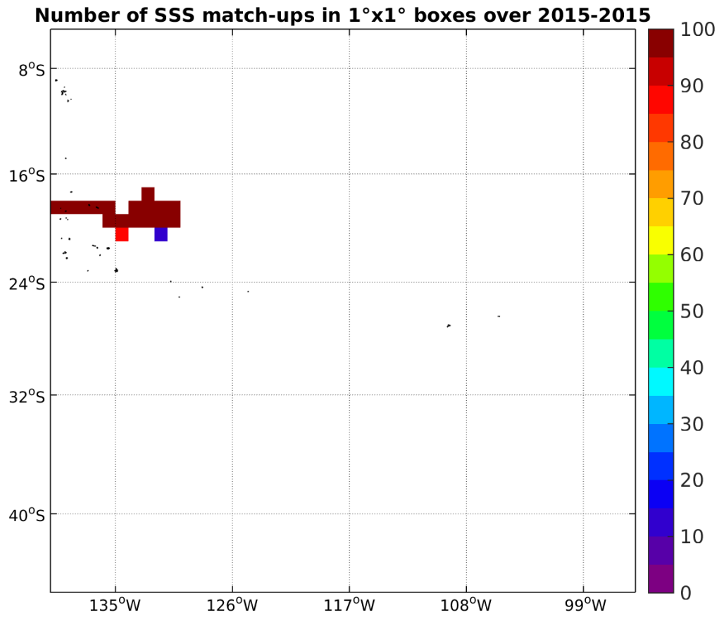
Figure 4: Number of SSS match-ups between TSG-GOSUD-Research-vessel SSS and the SMAP-L3-JPL-V4-8DAY-RUNNING-60KM SSS product for the OTT zone Pi-MEP region over 1°x1° boxes and for the full satellite product period.
