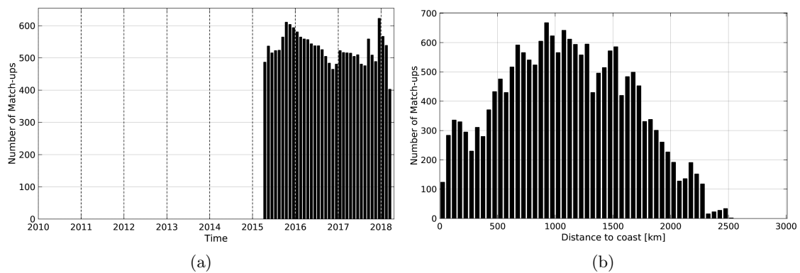
Figure 1: Number of match-ups between Argo and SMAP-L3-JPL-V4-8DAY-RUNNING-60KM SSS as a function of time (a) and as function of the distance to coast (b) over the OTT zone Pi-MEP region and for the full satellite product period.
