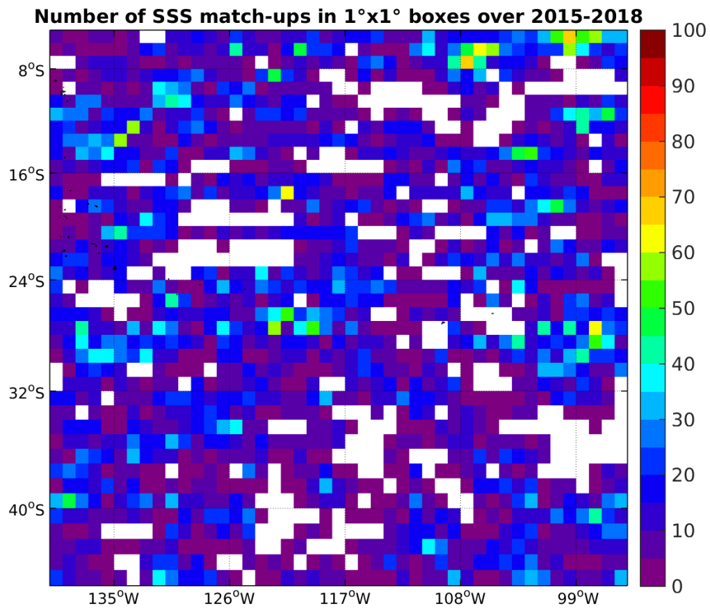
Figure 4: Number of SSS match-ups between Argo SSS and the SMAP-L3-JPL-V4-8DAY-RUNNING-60KM SSS product for the OTT zone Pi-MEP region over 1°x1° boxes and for the full satellite product period.
