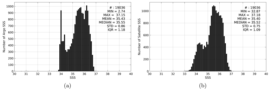
Figure 2: Histograms of SSS from Argo (a) and SMAP-L3-JPL-V4-8DAY-RUNNING-60KM (b) considering all match-up pairs per bins of 0.1 over the OTT zone Pi-MEP region and for the full satellite product period.
