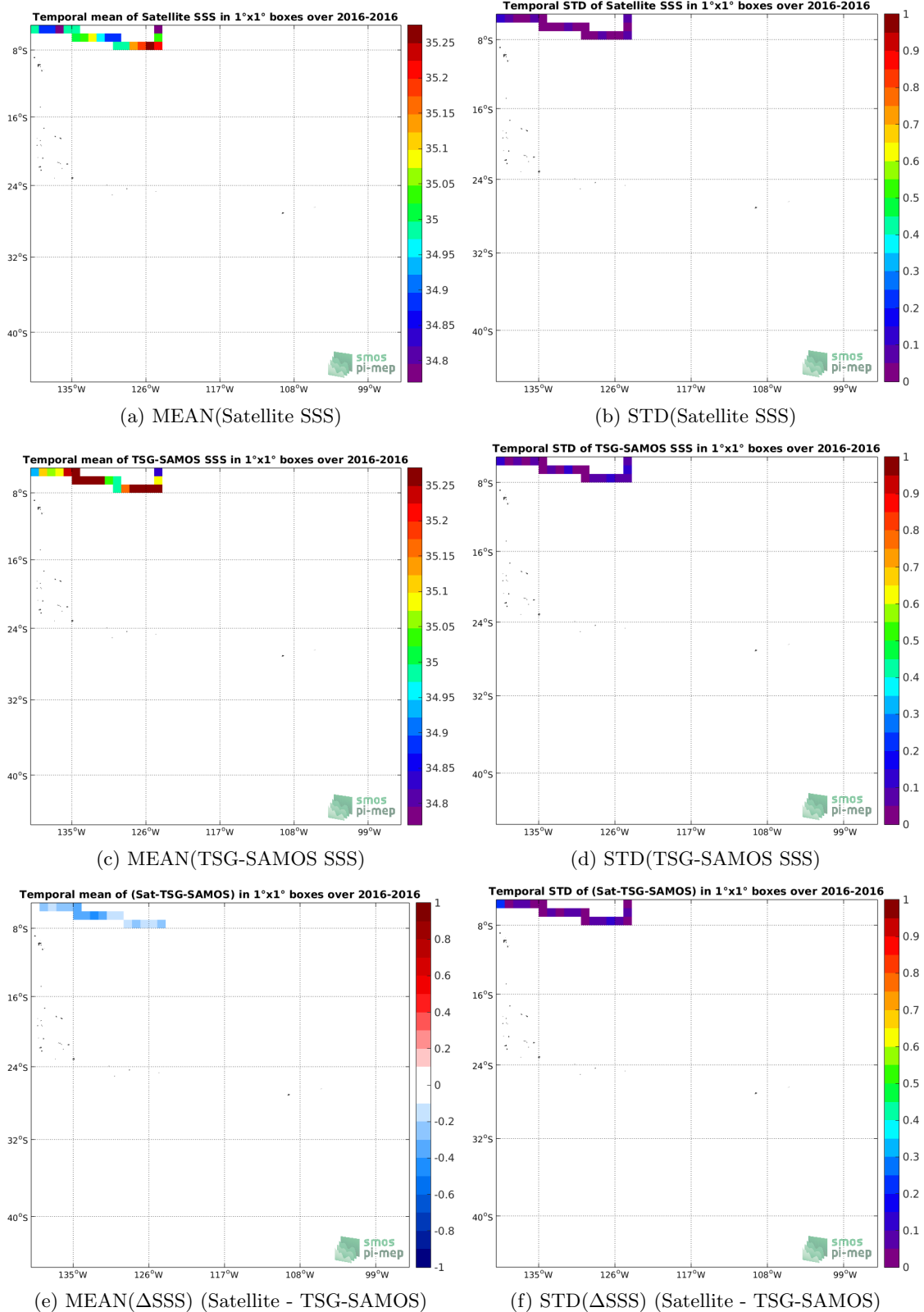
Figure 6: Temporal mean (left) and STD (right) of SSS from SMAP-L3-JPL-V4-MONTHLY-60KM (top), TSG-SAMOS (middle), and of \Delta SSS (Satellite - TSG-SAMOS). Only match-up pairs are used to generate these maps.
