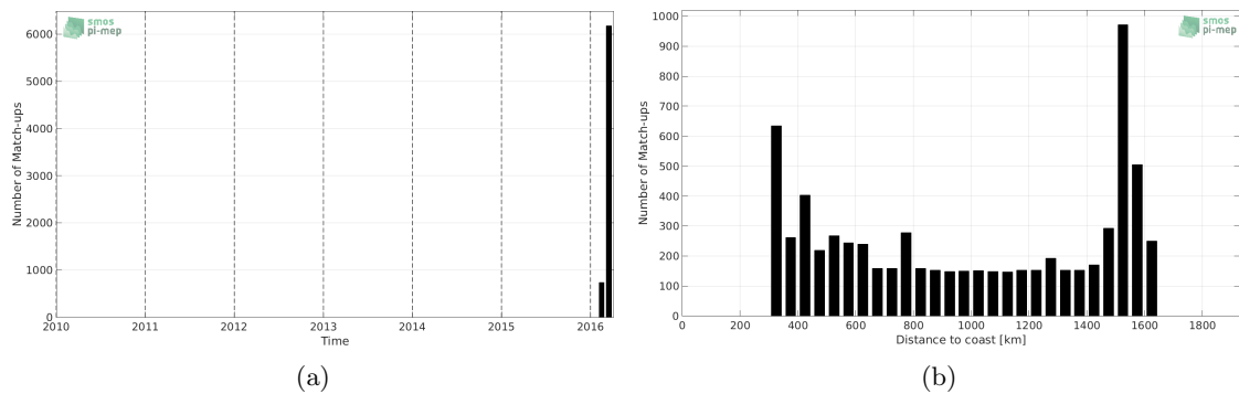
Figure 1: Number of match-ups between TSG-SAMOS and SMAP-L3-JPL-V4-MONTHLY-60KM SSS as a function of time (a) and as function of the distance to coast (b) over the OTT zone Pi-MEP region and for the full satellite product period.
