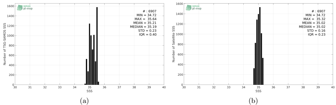
Figure 2: Histograms of SSS from TSG-SAMOS (a) and SMAP-L3-JPL-V4-MONTHLY-60KM (b) considering all match-up pairs per bins of 0.1 over the OTT zone Pi-MEP region and for the full satellite product period.
