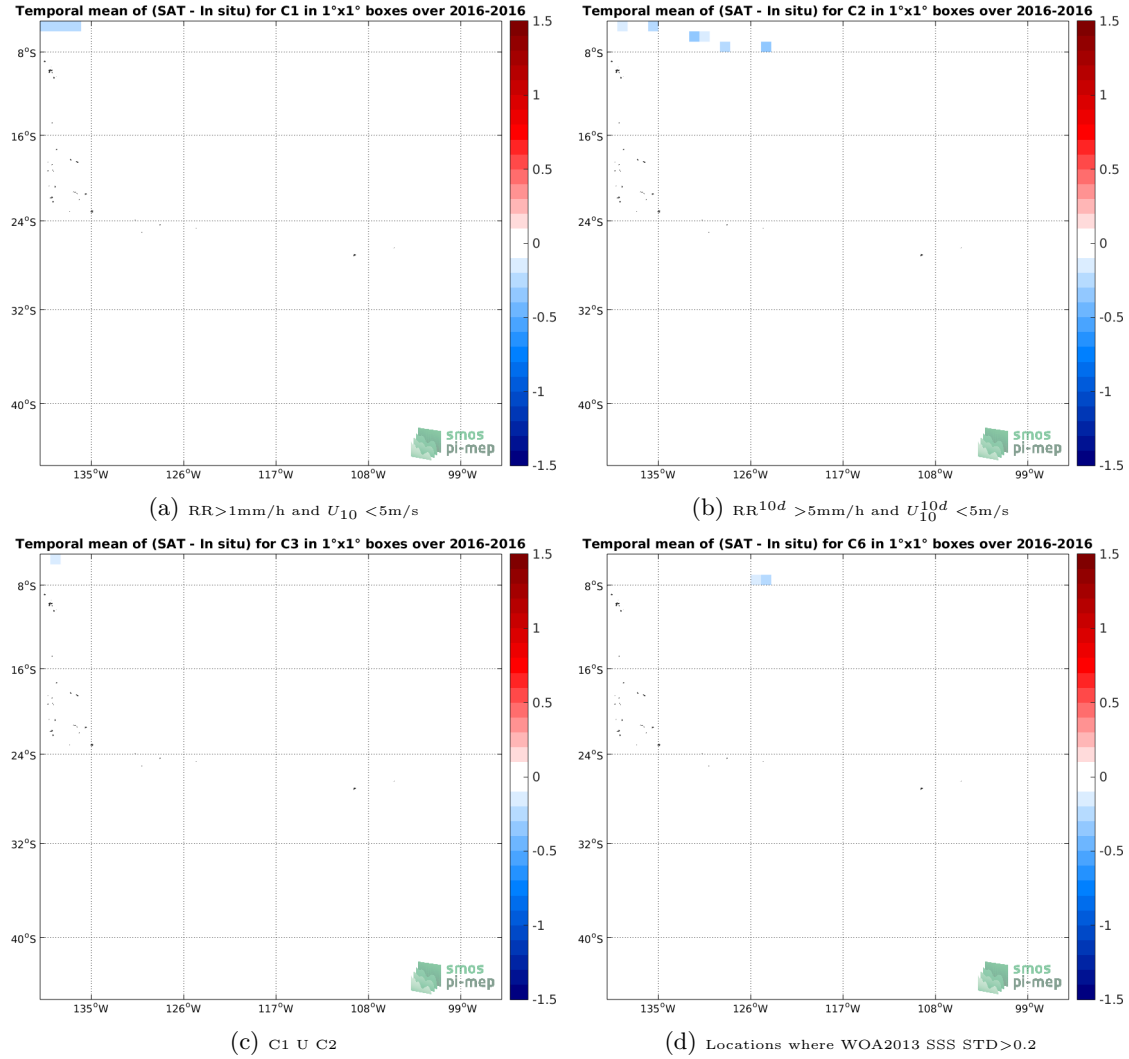
Figure 12: Temporal mean gridded over spatial boxes of size 1^\circ \times 1^\circ of \Delta SSS (SMAP-L3-JPL-V4-MONTHLY-60KM - TSG-SAMOS) for 4 different subdatasets corresponding to: RR > 1mm/h and U_{10} < 5\text{m/s} (a), RR^{10d} > 5\text{mm/h} and U_{10}^{10d} < 5\text{m/s} (b), C1 U C2 (c), Locations where WOA2013 SSS STD > 0.2 (d).
