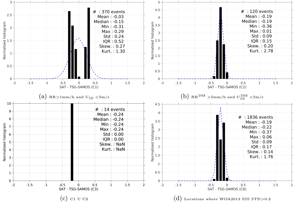
Figure 13: Normalized histogram of \Delta\text{SSS} (SMAP-L3-JPL-V4-MONTHLY-60KM - TSG-SAMOS) for 6 different subdatasets corresponding to: RR>1mm/h and U_{10} < 5\text{m/s} (a), RR^{10d} > 5\text{mm/h} and U_{10}^{10d} < 5\text{m/s} (b), C1 U C2 (c), Locations where WOA2013 SSS STD>0.2 (d).
