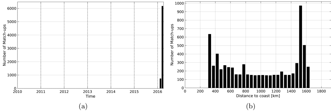
Figure 1: Number of match-ups between TSG-SAMOS and SMAP-L3-JPL-V4-MONTHLY-60KM SSS as a function of time (a) and as function of the distance to coast (b) over the OTT zone Pi-MEP region and for the full satellite product period.
