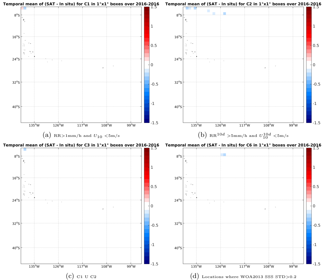
Figure 12: Temporal mean gridded over spatial boxes of size 1^\circ \times 1^\circ of \Delta SSS (SMAP-L3-JPL-V4-MONTHLY-60KM - TSG-SAMOS) for 4 different subdatasets corresponding to: RR > 1\text{mm/h} and U_{10} < 5\text{m/s} (a), RR^{10d} > 5\text{mm/h} and U_{10}^{10d} < 5\text{m/s} (b), C1 U C2 (c), Locations where WOA2013 SSS STD > 0.2 (d).
