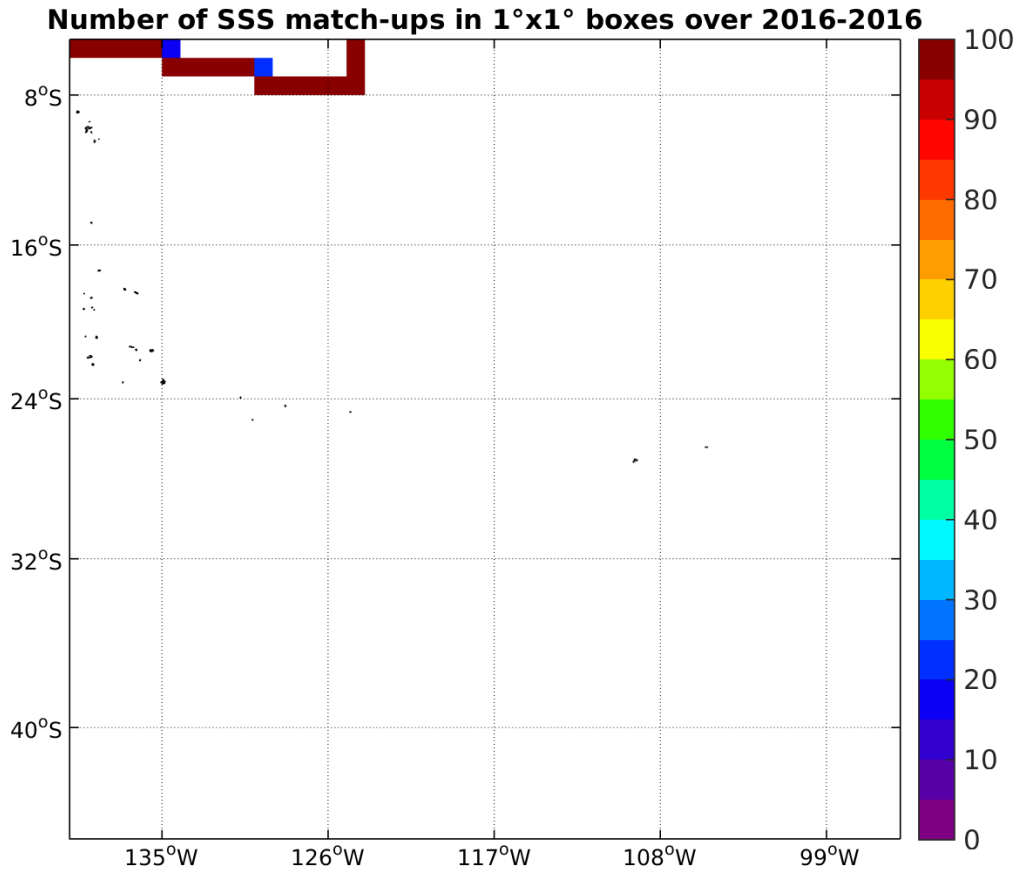
Figure 4: Number of SSS match-ups between TSG-SAMOS SSS and the SMAP-L3-JPL-V4-MONTHLY-60KM SSS product for the OTT zone Pi-MEP region over 1°x1° boxes and for the full satellite product period.
