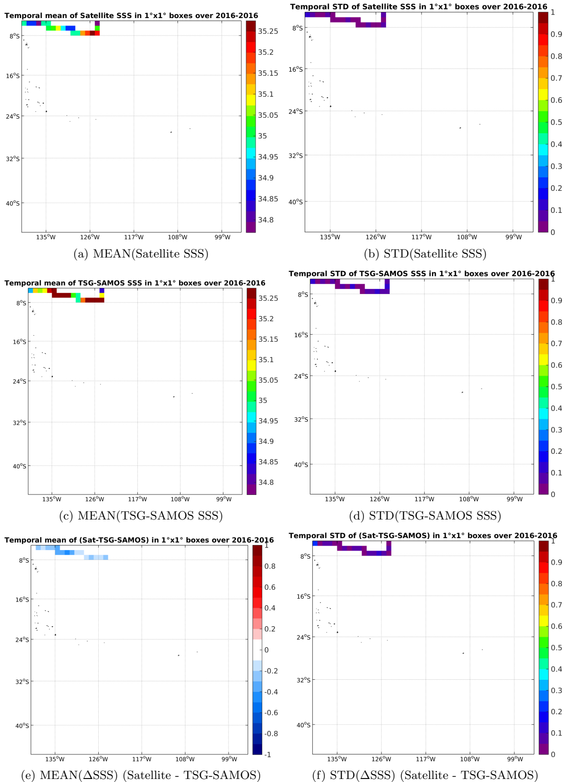
Figure 6: Temporal mean (left) and STD (right) of SSS from SMAP-L3-JPL-V4-MONTHLY-60KM (top), TSG-SAMOS (middle), and of \Delta SSS (Satellite - TSG-SAMOS). Only match-up pairs are used to generate these maps.
