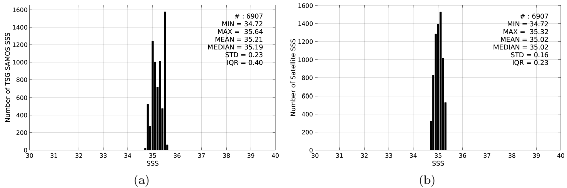
Figure 2: Histograms of SSS from TSG-SAMOS (a) and SMAP-L3-JPL-V4-MONTHLY-60KM (b) considering all match-up pairs per bins of 0.1 over the OTT zone Pi-MEP region and for the full satellite product period.
