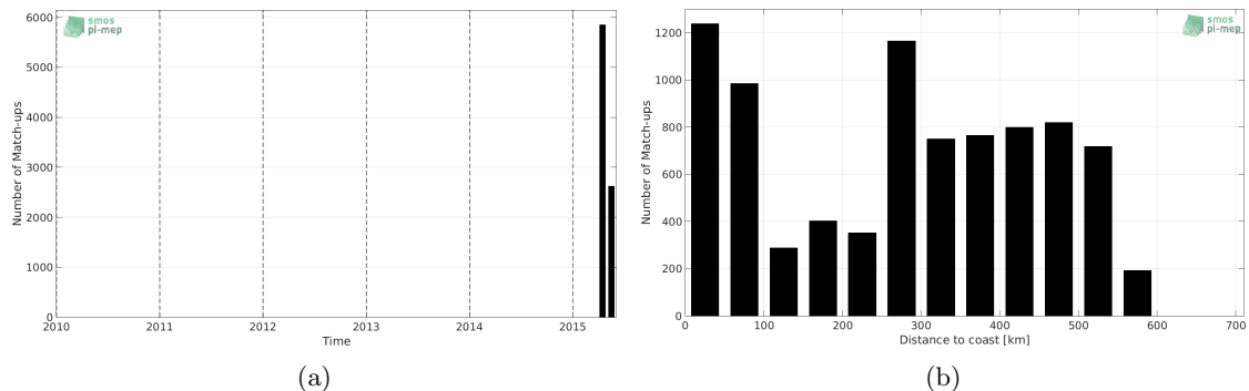
Figure 1: Number of match-ups between TSG-GOSUD-Research-vessel and SMAP-L3-JPL-V4-MONTHLY-60KM SSS as a function of time (a) and as function of the distance to coast (b) over the OTT zone Pi-MEP region and for the full satellite product period.
