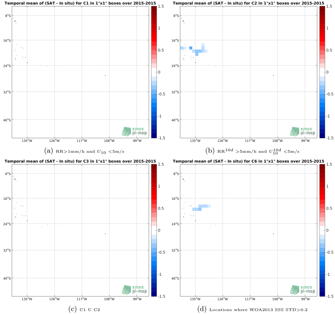
Figure 12: Temporal mean gridded over spatial boxes of size 1^\circ \times 1^\circ of \Delta SSS (SMAP-L3-JPL-V4-MONTHLY-60KM - TSG-GOSUD-Research-vessel) for 4 different subdatasets corresponding to: RR > 1\text{mm/h} and U_{10} < 5\text{m/s} (a), RR^{10d} > 5\text{mm/h} and U_{10}^{10d} < 5\text{m/s} (b), C1 U C2 (c), Locations where WOA2013 SSS STD > 0.2 (d).
