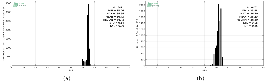
Figure 2: Histograms of SSS from TSG-GOSUD-Research-vessel (a) and SMAP-L3-JPL-V4-MONTHLY-60KM (b) considering all match-up pairs per bins of 0.1 over the OTT zone Pi-MEP region and for the full satellite product period.
