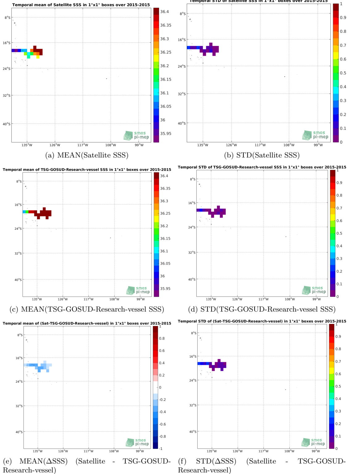
Figure 6: Temporal mean (left) and STD (right) of SSS from SMAP-L3-JPL-V4-MONTHLY-60KM (top), TSG-GOSUD-Research-vessel (middle), and of \Delta SSS (Satellite - TSG-GOSUD-Research-vessel). Only match-up pairs are used to generate these maps.
