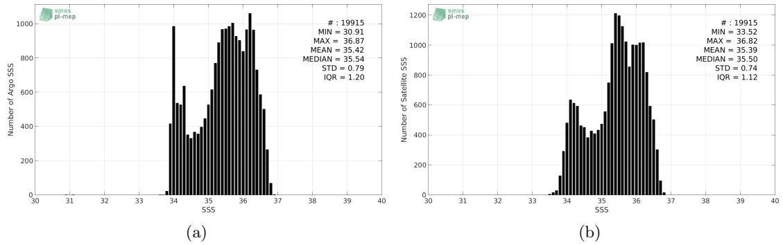
Figure 2: Histograms of SSS from Argo (a) and SMAP-L3-JPL-V4-MONTHLY-60KM (b) considering all match-up pairs per bins of 0.1 over the OTT zone Pi-MEP region and for the full satellite product period.
