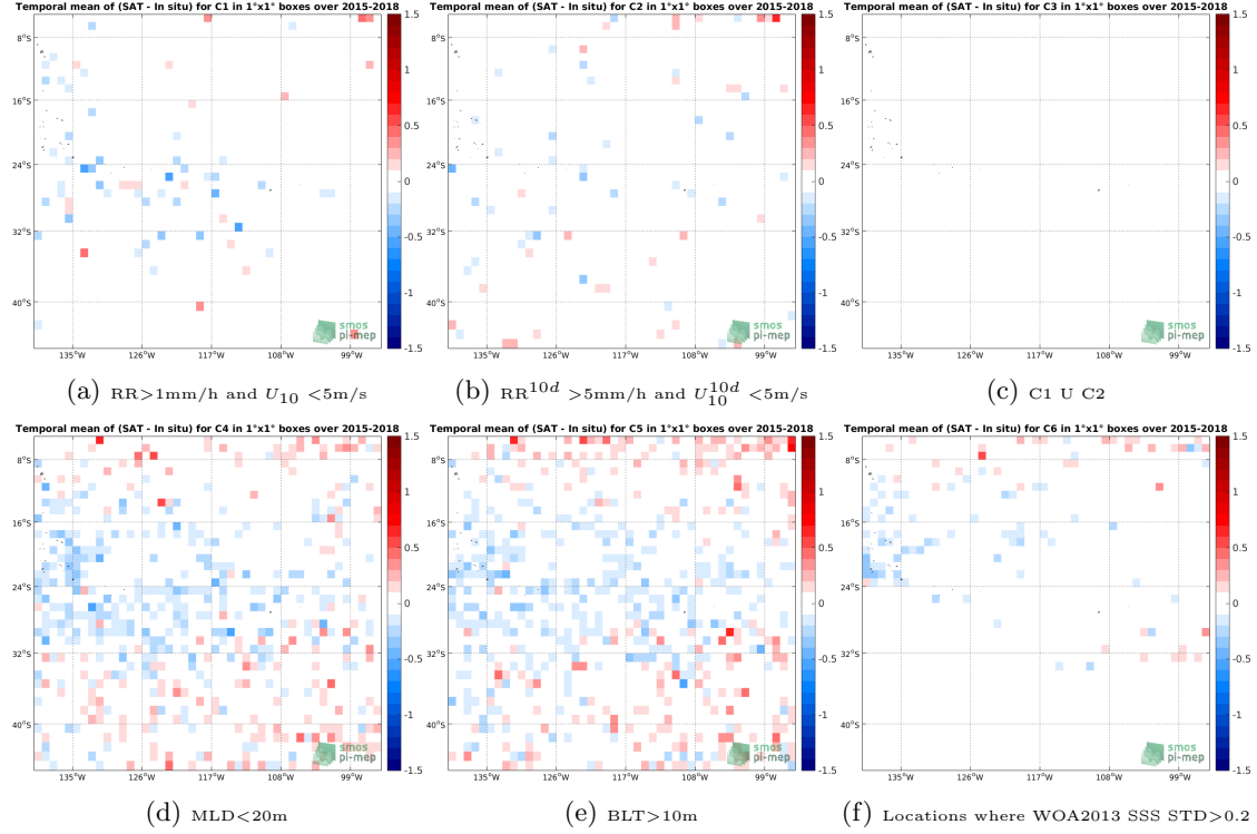
Figure 12: Temporal mean gridded over spatial boxes of size 1^\circ \times 1^\circ of \Delta\text{SSS} (SMAP-L3-JPL-V4-MONTHLY-60KM - Argo) for 6 different subdatasets corresponding to: RR > 1mm/h and U_{10} < 5\text{m/s} (a), \text{RR}^{10d} > 5\text{mm/h} and U_{10}^{10d} < 5\text{m/s} (b), C1 U C2 (c), MLD < 20m (d), BLT > 10m (e), Locations where WOA2013 SSS STD > 0.2 (f).
