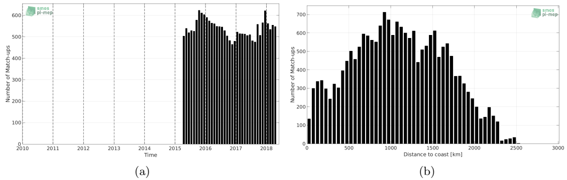
Figure 1: Number of match-ups between Argo and SMAP-L3-JPL-V4-MONTHLY-60KM SSS as a function of time (a) and as function of the distance to coast (b) over the OTT zone Pi-MEP region and for the full satellite product period.
