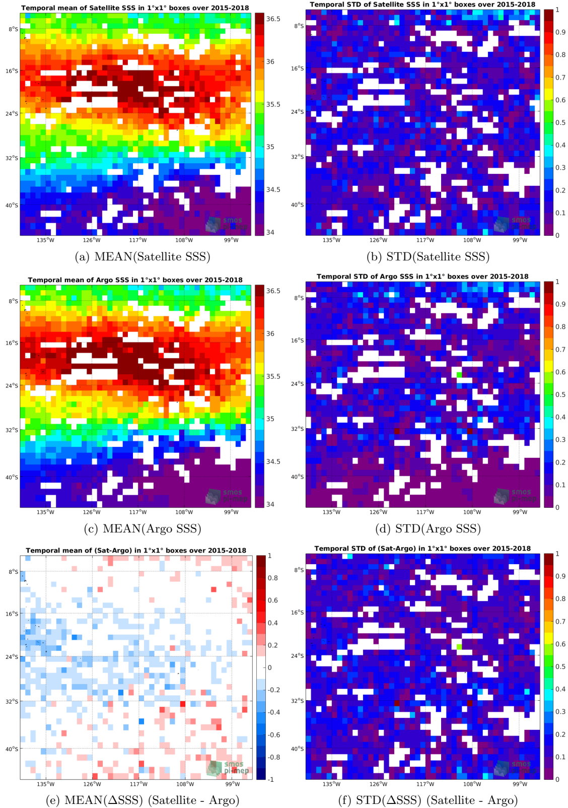
Figure 6: Temporal mean (left) and STD (right) of SSS from SMAP-L3-JPL-V4-MONTHLY-60KM (top), Argo (middle), and of ΔSSS (Satellite - Argo). Only match-up pairs are used to generate these maps.
