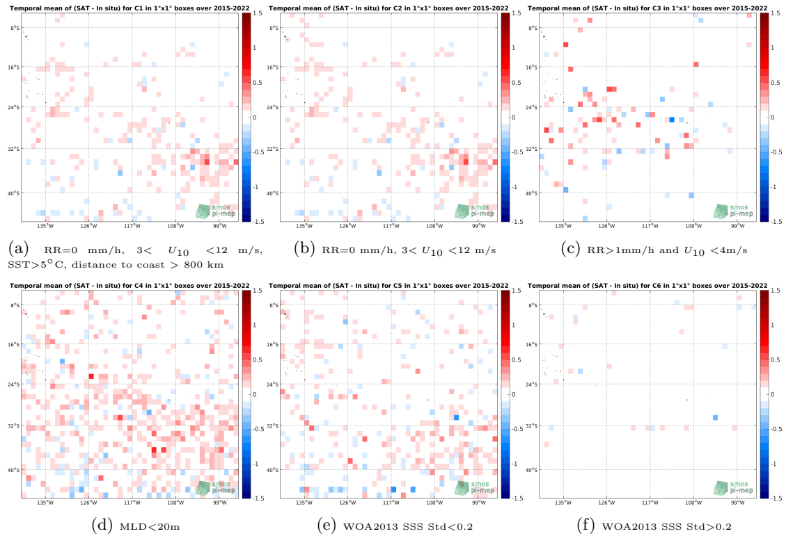
Figure 12: Temporal mean gridded over spatial boxes of size 1^\circ \times 1^\circ of \Delta SSS (SMAP SSS L2-AVERAGED v5 (RSS) - Argo) for 6 different subdatasets corresponding to:RR=0 mm/h, 3 < U_{10} < 12 m/s, SST > 5^\circ C, distance to coast > 800 km (a), RR=0 mm/h, 3 < U_{10} < 12 m/s (b), RR > 1 mm/h and U_{10} < 4 m/s (c),MLD < 20 m (d),WOA2013 SSS Std < 0.2 (e),WOA2013 SSS Std > 0.2 (f).
