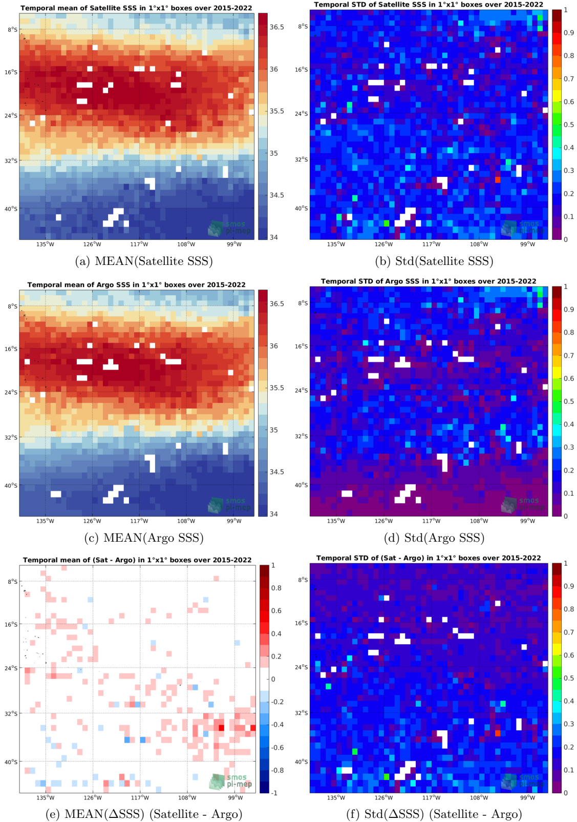
Figure 6: Temporal mean (left) and Std (right) of SSS from SMAP SSS L2-AVERAGED v5 (RSS) (top), Argo (middle), and of \Delta SSS (Satellite - Argo). Only match-up pairs are used to generate these maps.
