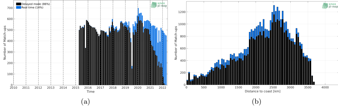
Figure 1: Number of match-ups between Argo and SMAP SSS L2-AVERAGED v5 (RSS) SSS as a function of time (a) and as function of the distance to coast (b) over the OTT zone Pi-MEP region and for the full satellite product period.
