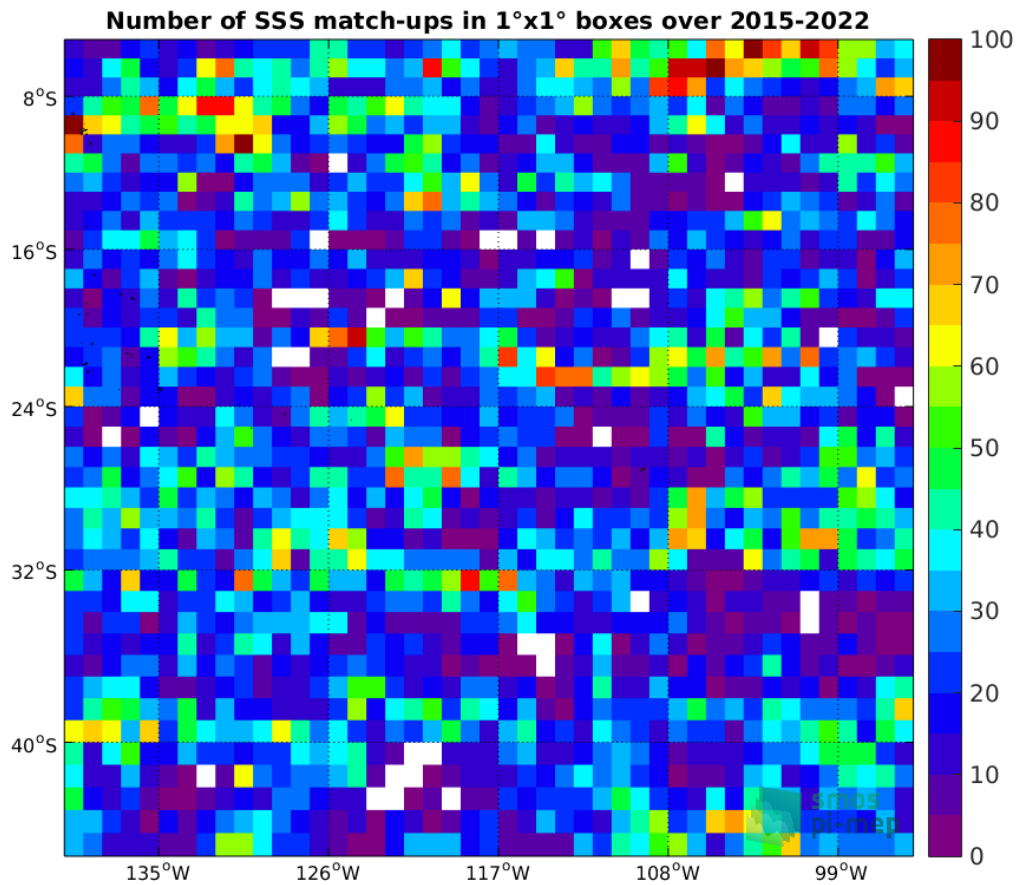
Figure 4: Number of SSS match-ups between Argo SSS and the SMAP SSS L2-AVERAGED v5 (RSS) SSS product for the OTT zone Pi-MEP region over 1^\circ \times 1^\circ boxes and for the full satellite product period.
