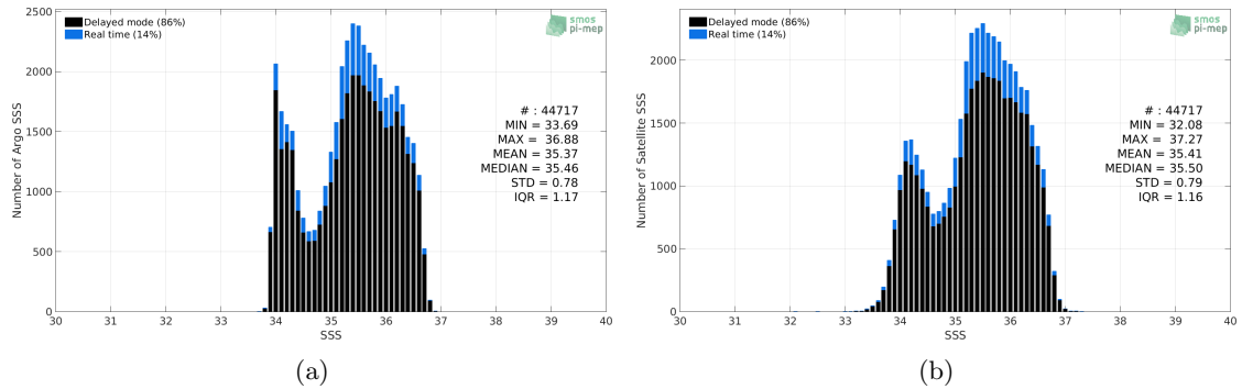
Figure 2: Histograms of SSS from Argo (a) and SMAP SSS L2-AVERAGED v5 (RSS) (b) considering all match-up pairs per bins of 0.1 over the OTT zone Pi-MEP region and for the full satellite product period.
