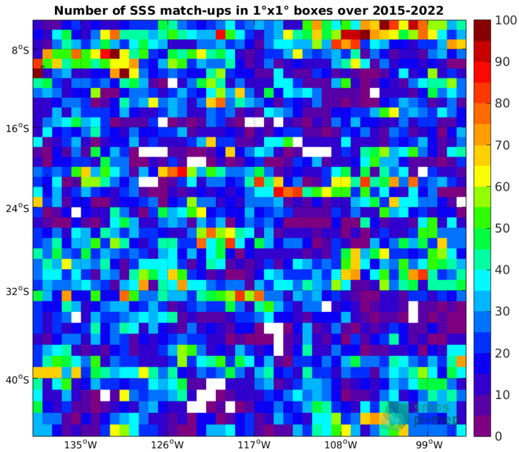
Figure 4: Number of SSS match-ups between Argo SSS and the SMAP SSS L2-AVERAGED v5.0 (JPL) SSS product for the OTT zone Pi-MEP region over 1°×1° boxes and for the full satellite product period.
