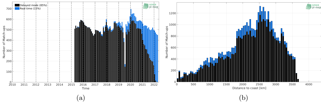
Figure 1: Number of match-ups between Argo and SMAP SSS L2-AVERAGED v5.0 (JPL) SSS as a function of time (a) and as function of the distance to coast (b) over the OTT zone Pi-MEP region and for the full satellite product period.
