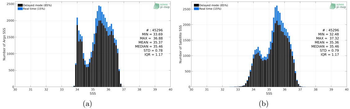
Figure 2: Histograms of SSS from Argo (a) and SMAP SSS L2-AVERAGED v5.0 (JPL) (b) considering all match-up pairs per bins of 0.1 over the OTT zone Pi-MEP region and for the full satellite product period.
