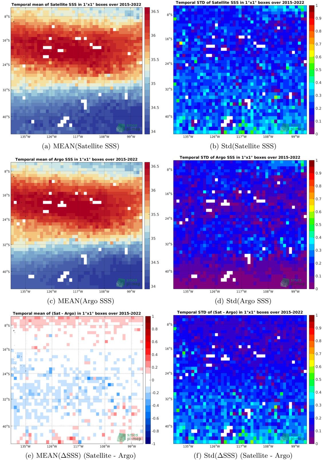
Figure 6: Temporal mean (left) and Std (right) of SSS from SMAP SSS L2-AVERAGED v5.0 (JPL) (top), Argo (middle), and of \Delta SSS (Satellite - Argo). Only match-up pairs are used to generate these maps.
