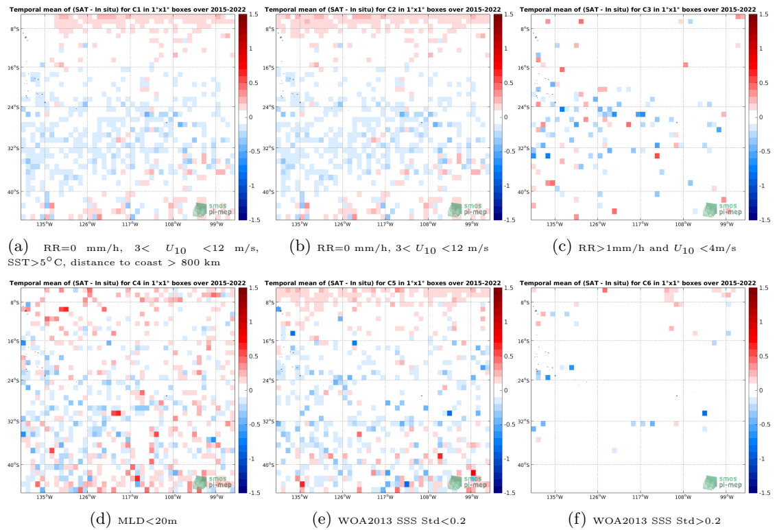
Figure 12: Temporal mean gridded over spatial boxes of size 1^\circ \times 1^\circ of \Delta SSS (SMAP SSS L2-AVERAGED v5.0 (JPL) - Argo) for 6 different subdatasets corresponding to:RR=0 mm/h, 3 < U_{10} < 12 m/s, SST > 5^\circ\text{C} , distance to coast > 800 km (a), RR=0 mm/h, 3 < U_{10} < 12 m/s (b), RR > 1 mm/h and U_{10} < 4 m/s (c),MLD < 20 m (d),WOA2013 SSS Std < 0.2 (e),WOA2013 SSS Std > 0.2 (f).
