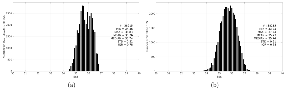
Figure 3: Histograms of SSS from TSG (LEGOS-DM) (a) and SMAP SSS L2 v6 (RSS) (b) considering all match-up pairs per bins of 0.1 over the OTT zone Pi-MEP region and for the full satellite product period.
