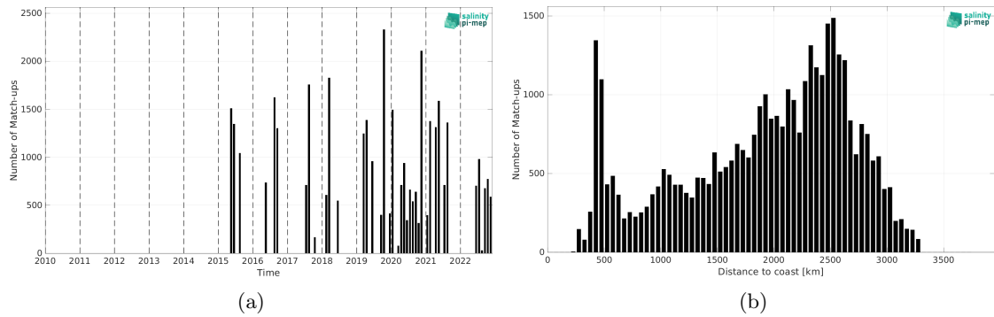
Figure 2: Number of match-ups between TSG (LEGOS-DM) and SMAP SSS L2 v6 (RSS) SSS as a function of time (a) and as function of the distance to coast (b) over the OTT zone Pi-MEP region and for the full satellite product period.
