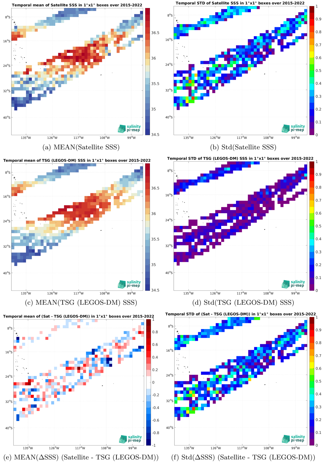
Figure 7: Temporal mean (left) and Std (right) of SSS from SMAP SSS L2 v6 (RSS) (top), TSG (LEGOS-DM) (middle), and of \Delta SSS (Satellite - TSG (LEGOS-DM)). Only match-up pairs are used to generate these maps.
