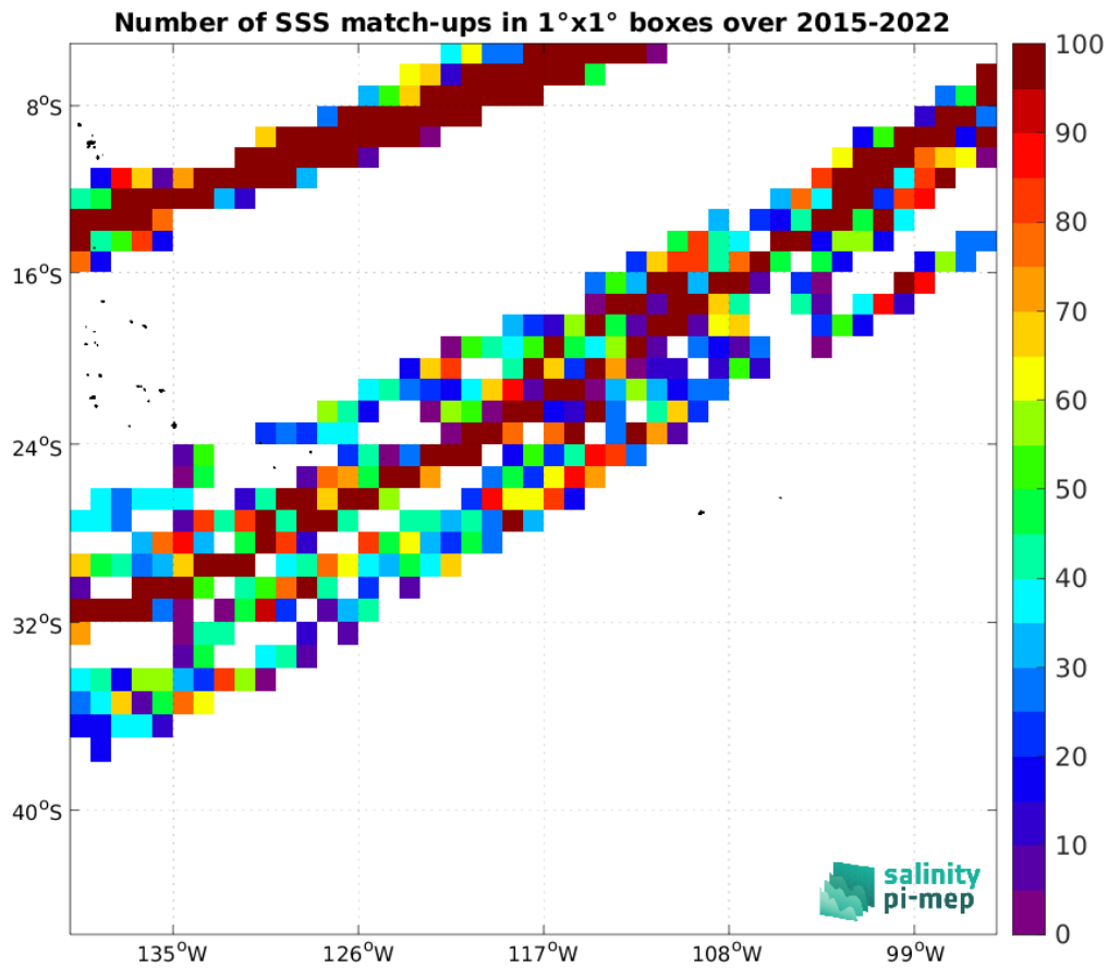
Figure 5: Number of SSS match-ups between TSG (LEGOS-DM) SSS and the SMAP SSS L2 v6 (RSS) SSS product for the OTT zone Pi-MEP region over 1^\circ \times 1^\circ boxes and for the full satellite product period.
