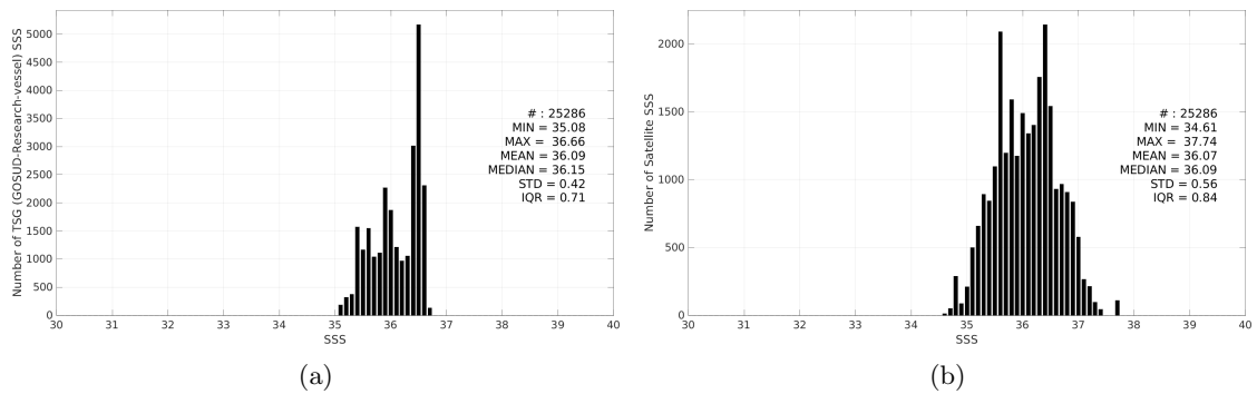
Figure 3: Histograms of SSS from TSG (GOSUD-Research-vessel) (a) and SMAP SSS L2 v6 (RSS) (b) considering all match-up pairs per bins of 0.1 over the OTT zone Pi-MEP region and for the full satellite product period.
