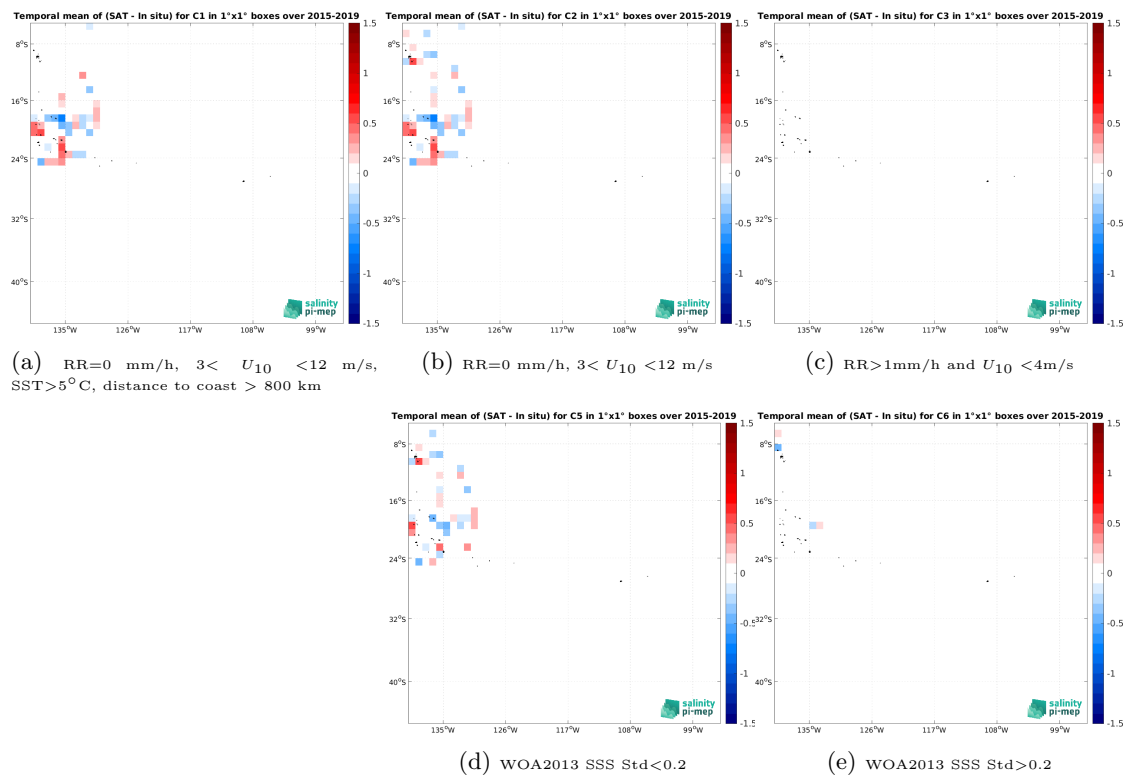
Figure 14: Temporal mean gridded over spatial boxes of size 1^\circ \times 1^\circ of \Delta SSS (SMAP SSS L2 v6 (RSS) - TSG (GOSUD-Research-vessel)) for 5 different subdatasets corresponding to: RR=0 mm/h, 3 < U_{10} < 12 m/s, SST > 5^\circ C , distance to coast > 800 km (a), RR=0 mm/h, 3 < U_{10} < 12 m/s (b), RR > 1 mm/h and U_{10} < 4 m/s (c), WOA2013 SSS Std < 0.2 (d), WOA2013 SSS Std > 0.2 (e).
