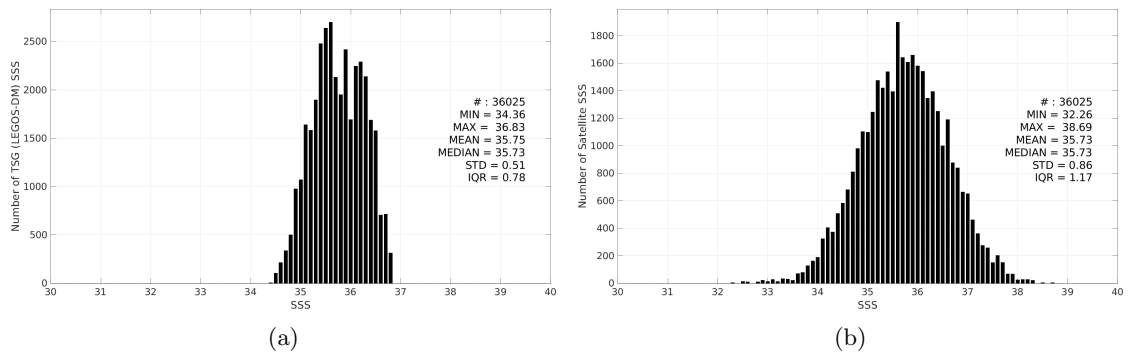
Figure 3: Histograms of SSS from TSG (LEGOS-DM) (a) and SMAP SSS L2 v6 - 40 km (RSS) (b) considering all match-up pairs per bins of 0.1 over the OTT zone Pi-MEP region and for the full satellite product period.
