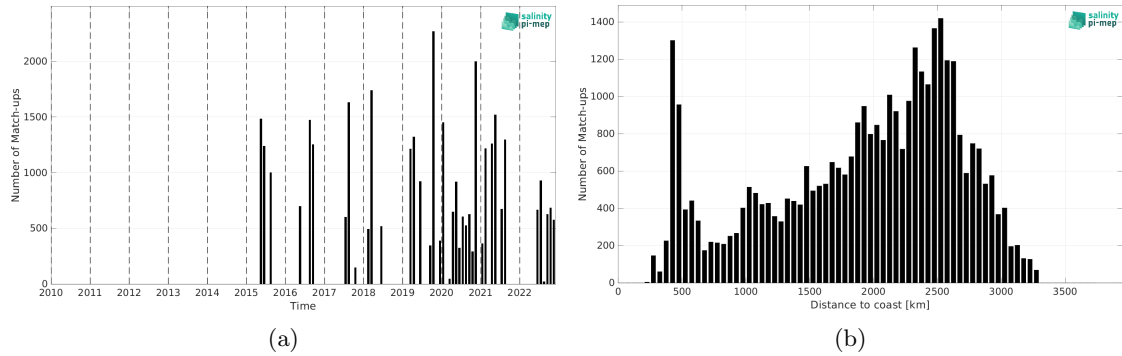
Figure 2: Number of match-ups between TSG (LEGOS-DM) and SMAP SSS L2 v6 - 40 km (RSS) SSS as a function of time (a) and as function of the distance to coast (b) over the OTT zone Pi-MEP region and for the full satellite product period.
