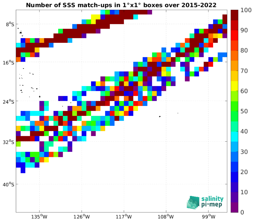
Figure 5: Number of SSS match-ups between TSG (LEGOS-DM) SSS and the SMAP SSS L2 v6 - 40 km (RSS) SSS product for the OTT zone Pi-MEP region over 1^\circ \times 1^\circ boxes and for the full satellite product period.
