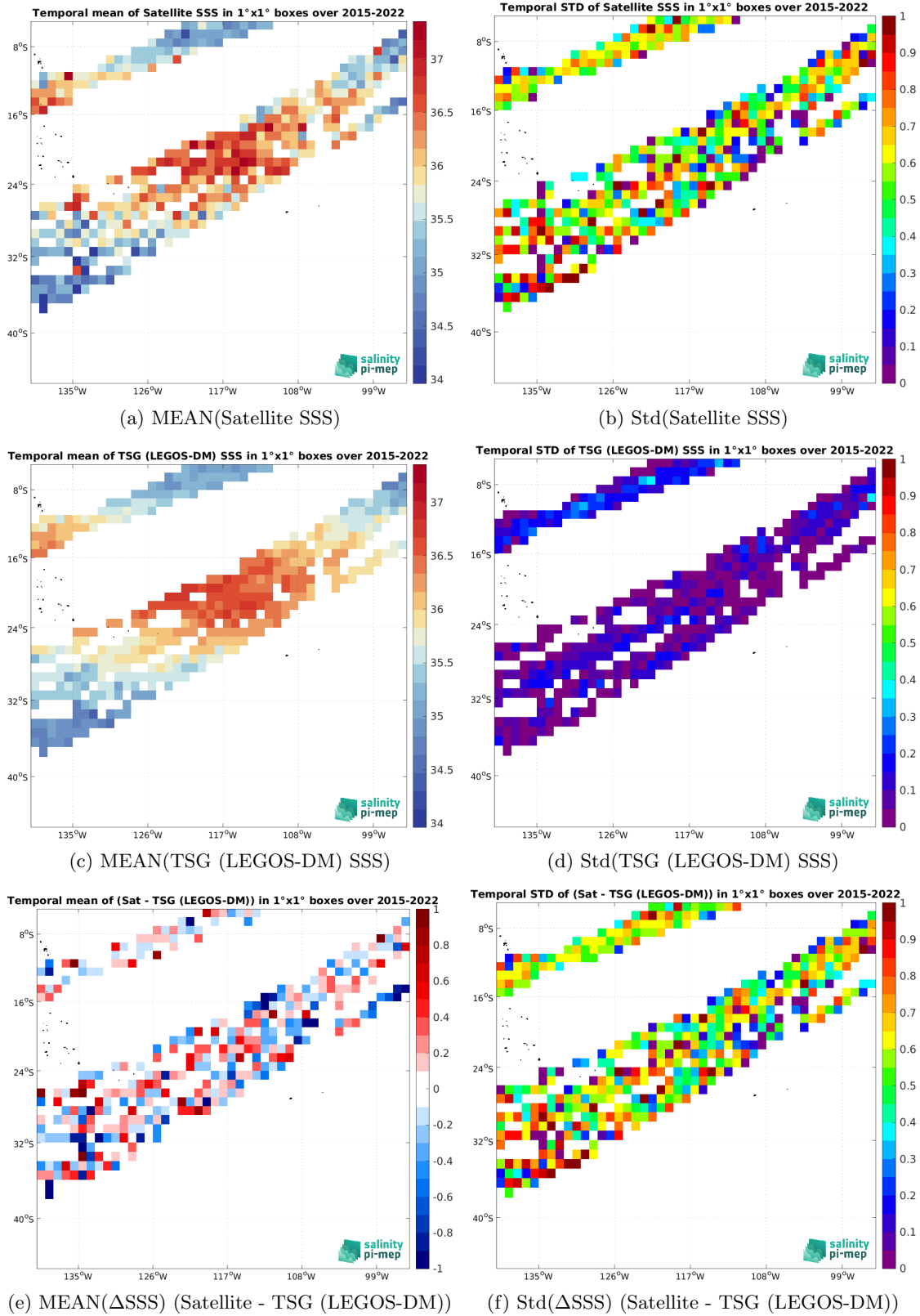
Figure 7: Temporal mean (left) and Std (right) of SSS from SMAP SSS L2 v6 - 40 km (RSS) (top), TSG (LEGOS-DM) (middle), and of \Delta SSS (Satellite - TSG (LEGOS-DM)). Only match-up pairs are used to generate these maps.
