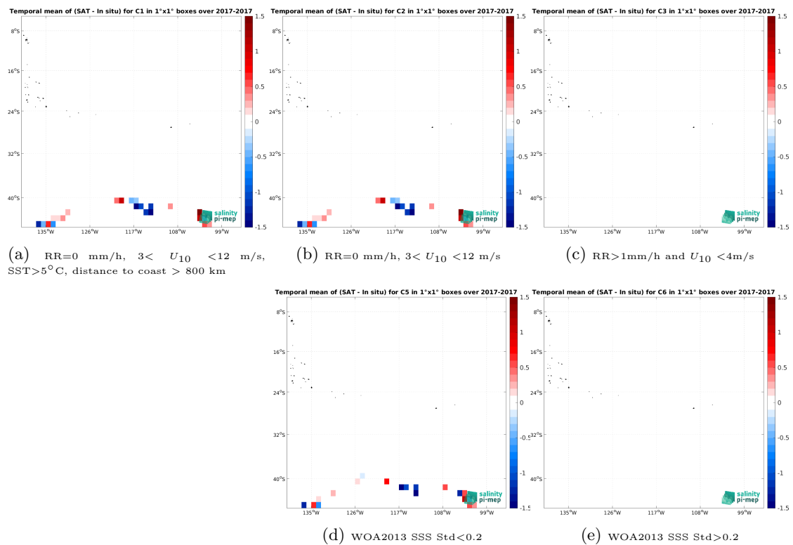
Figure 14: Temporal mean gridded over spatial boxes of size 1^\circ \times 1^\circ of \Delta SSS (SMAP SSS L2 v6 - 40 km (RSS) - TSG (GOSUD-Sailing-ship)) for 5 different subdatasets corresponding to:RR=0 mm/h, 3 < U_{10} < 12 m/s, SST >5^\circ\text{C} , distance to coast > 800 km (a), RR=0 mm/h, 3 < U_{10} < 12 m/s (b), RR >1 mm/h and U_{10} < 4 m/s (c), WOA2013 SSS Std <0.2 (d), WOA2013 SSS Std >0.2 (e).
