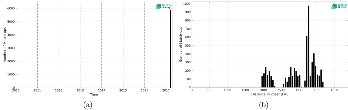
Figure 2: Number of match-ups between TSG (GOSUD-Sailing-ship) and SMAP SSS L2 v6 - 40 km (RSS) SSS as a function of time (a) and as function of the distance to coast (b) over the OTT zone Pi-MEP region and for the full satellite product period.
