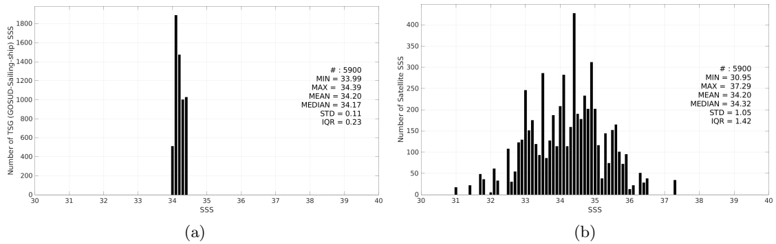
Figure 3: Histograms of SSS from TSG (GOSUD-Sailing-ship) (a) and SMAP SSS L2 v6 - 40 km (RSS) (b) considering all match-up pairs per bins of 0.1 over the OTT zone Pi-MEP region and for the full satellite product period.
