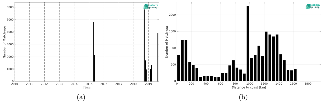
Figure 2: Number of match-ups between TSG (GOSUD-Research-vessel) and SMAP SSS L2 v6 - 40 km (RSS) SSS as a function of time (a) and as function of the distance to coast (b) over the OTT zone Pi-MEP region and for the full satellite product period.
