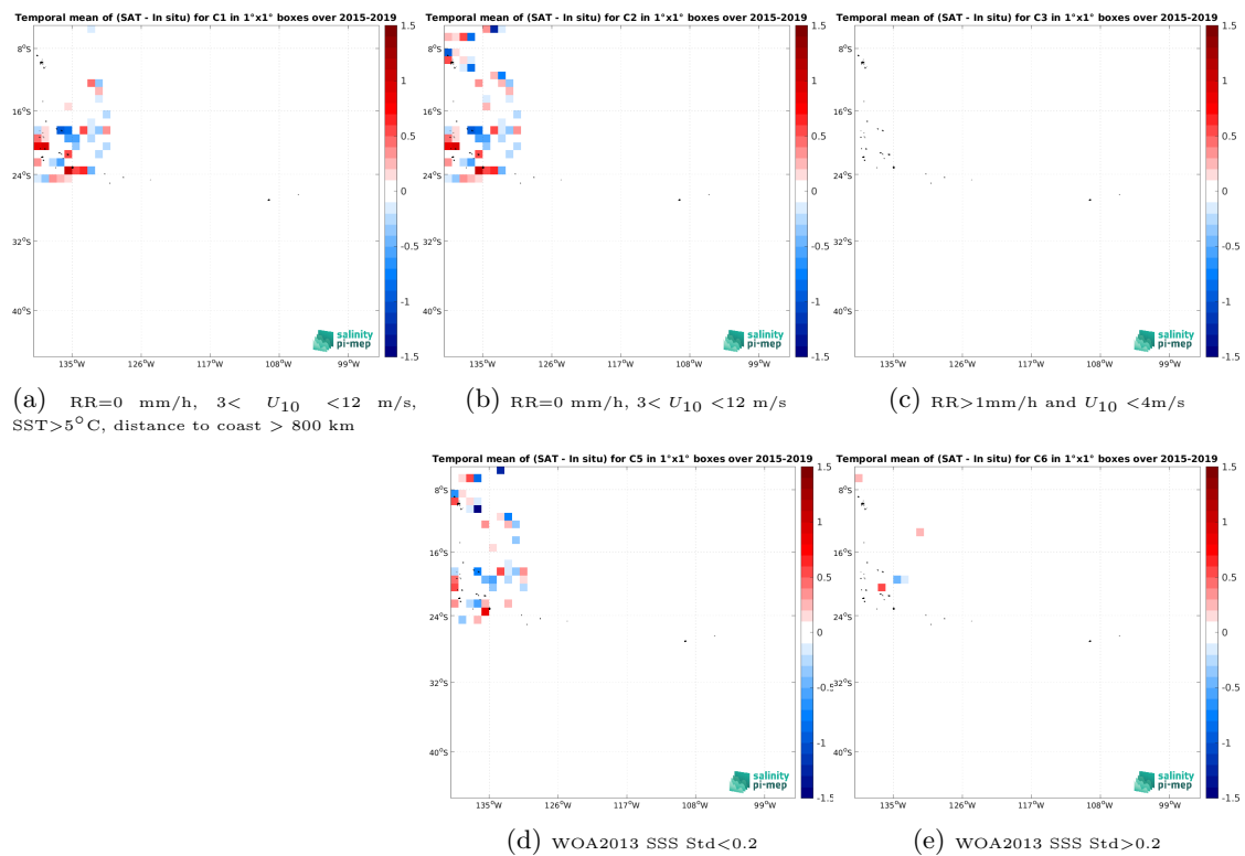
Figure 14: Temporal mean gridded over spatial boxes of size 1^\circ \times 1^\circ of \Delta SSS (SMAP SSS L2 v6 - 40 km (RSS) - TSG (GOSUD-Research-vessel)) for 5 different subdatasets corresponding to:RR=0 mm/h, 3 < U_{10} < 12 m/s, SST >5^\circ\text{C} , distance to coast > 800 km (a), RR=0 mm/h, 3 < U_{10} < 12 m/s (b), RR >1 mm/h and U_{10} < 4 m/s (c), WOA2013 SSS Std <0.2 (d), WOA2013 SSS Std >0.2 (e).
