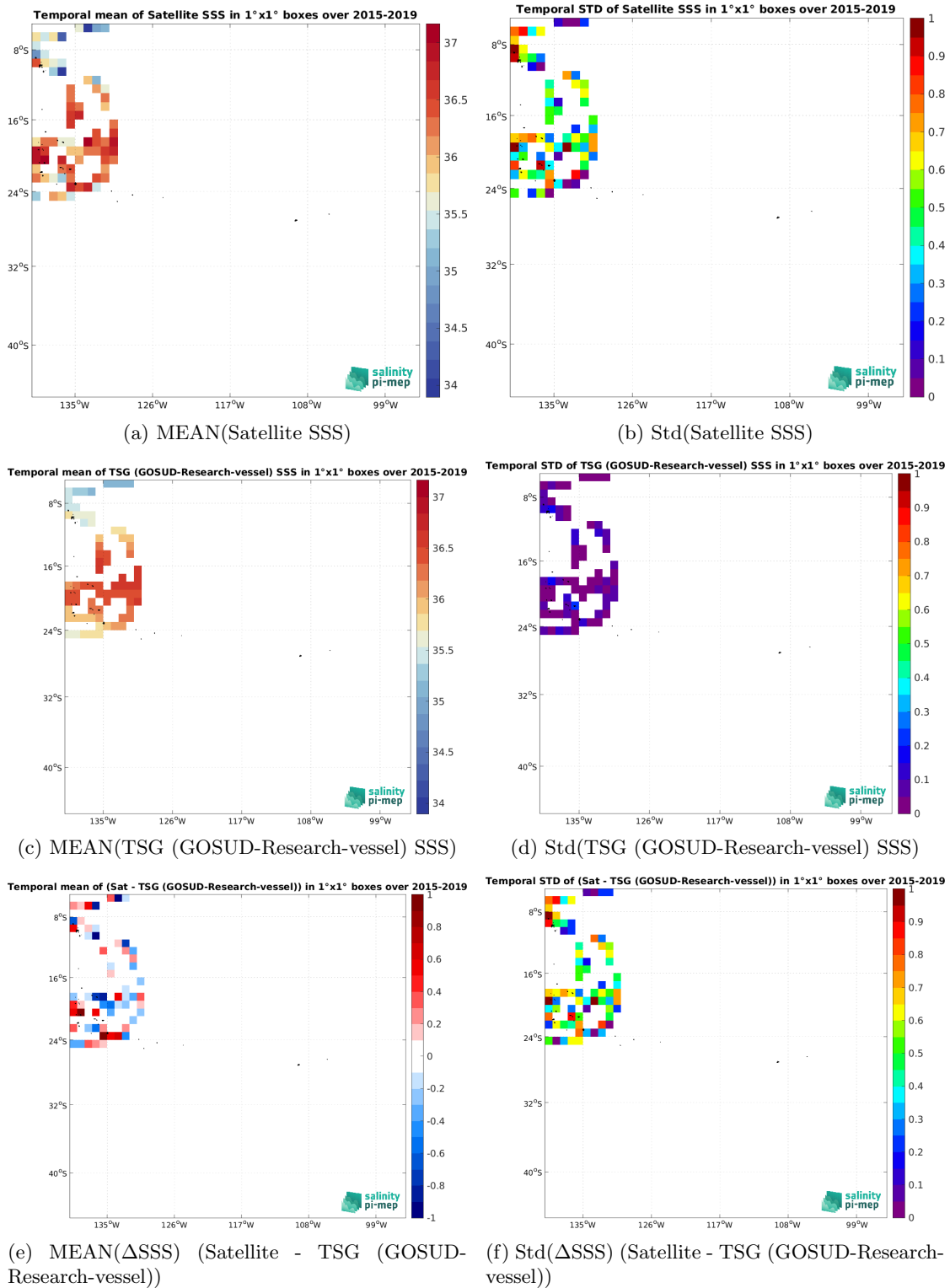
Figure 7: Temporal mean (left) and Std (right) of SSS from SMAP SSS L2 v6 - 40 km (RSS) (top), TSG (GOSUD-Research-vessel) (middle), and of \Delta SSS (Satellite - TSG (GOSUD-Research-vessel)). Only match-up pairs are used to generate these maps.
