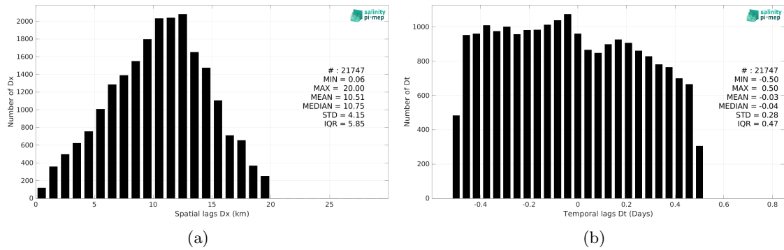
Figure 6: Histograms of the spatial (a) and temporal (b) lags between the location/time of the TSG (GOSUD-Research-vessel) measurement and the date of the corresponding SMAP SSS L2 v6 - 40 km (RSS) SSS pixel.
