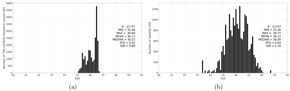
Figure 3: Histograms of SSS from TSG (GOSUD-Research-vessel) (a) and SMAP SSS L2 v6 - 40 km (RSS) (b) considering all match-up pairs per bins of 0.1 over the OTT zone Pi-MEP region and for the full satellite product period.
