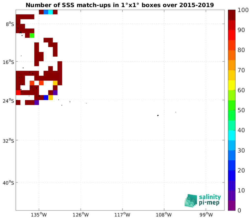
Figure 5: Number of SSS match-ups between TSG (GOSUD-Research-vessel) SSS and the SMAP SSS L2 v6 - 40 km (RSS) SSS product for the OTT zone Pi-MEP region over 1^\circ \times 1^\circ boxes and for the full satellite product period.
