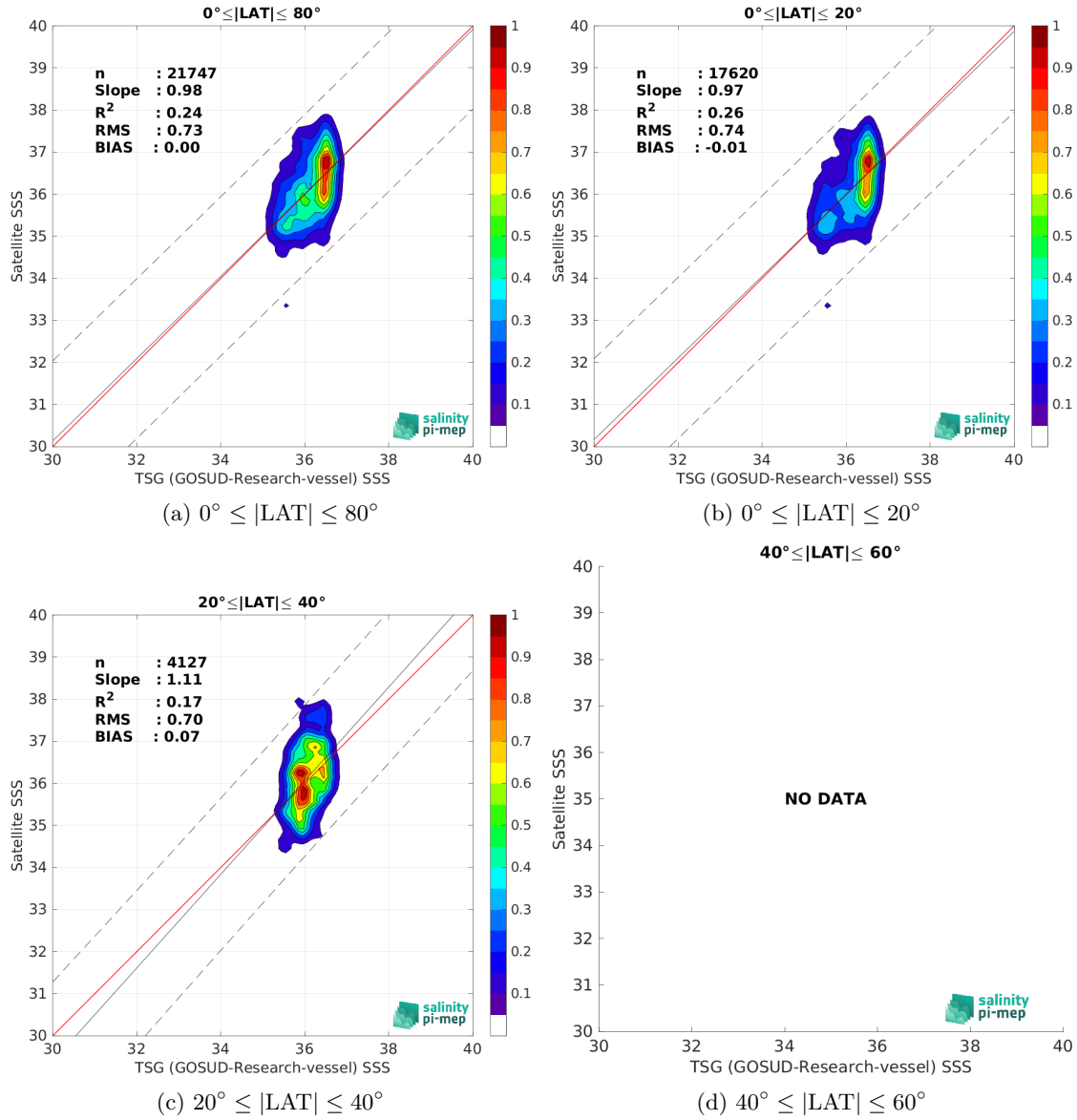
Figure 10: Contour maps of the concentration of SMAP SSS L2 v6 - 40 km (RSS) SSS (y-axis) versus TSG (GOSUD-Research-vessel) SSS (x-axis) at match-up pairs for different latitude bands. For each plot, the red line shows x=y . The black thin and dashed lines indicate a linear fit through the data cloud and the \pm 95\% confidence levels, respectively. The number match-up pairs n , the slope and R^2 coefficient of the linear fit, the root mean square (RMS) and the mean bias between satellite and in situ data are indicated for each latitude band in each plots.
