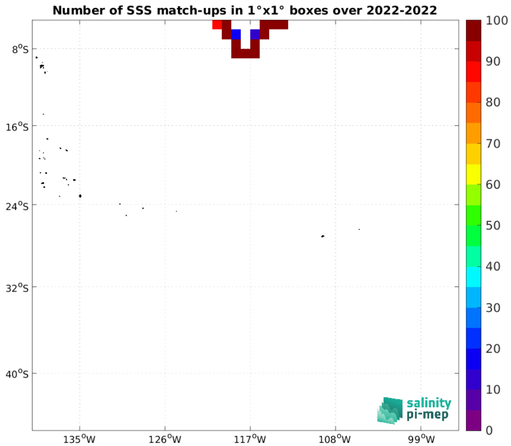
Figure 5: Number of SSS match-ups between Saildrone SSS and the SMAP SSS L2 v6 - 40 km (RSS) SSS product for the OTT zone Pi-MEP region over 1°x1° boxes and for the full satellite product period.
