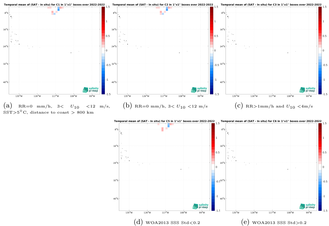
Figure 14: Temporal mean gridded over spatial boxes of size 1^\circ \times 1^\circ of \Delta SSS (SMAP SSS L2 v6 - 40 km (RSS) - Sairdrone) for 5 different subdatasets corresponding to:RR=0 mm/h, 3 < U_{10} < 12 m/s, SST >5^\circ\text{C} , distance to coast > 800 km (a), RR=0 mm/h, 3 < U_{10} < 12 m/s (b), RR >1 mm/h and U_{10} < 4 m/s (c), WOA2013 SSS Std <0.2 (d), WOA2013 SSS Std >0.2 (e).
