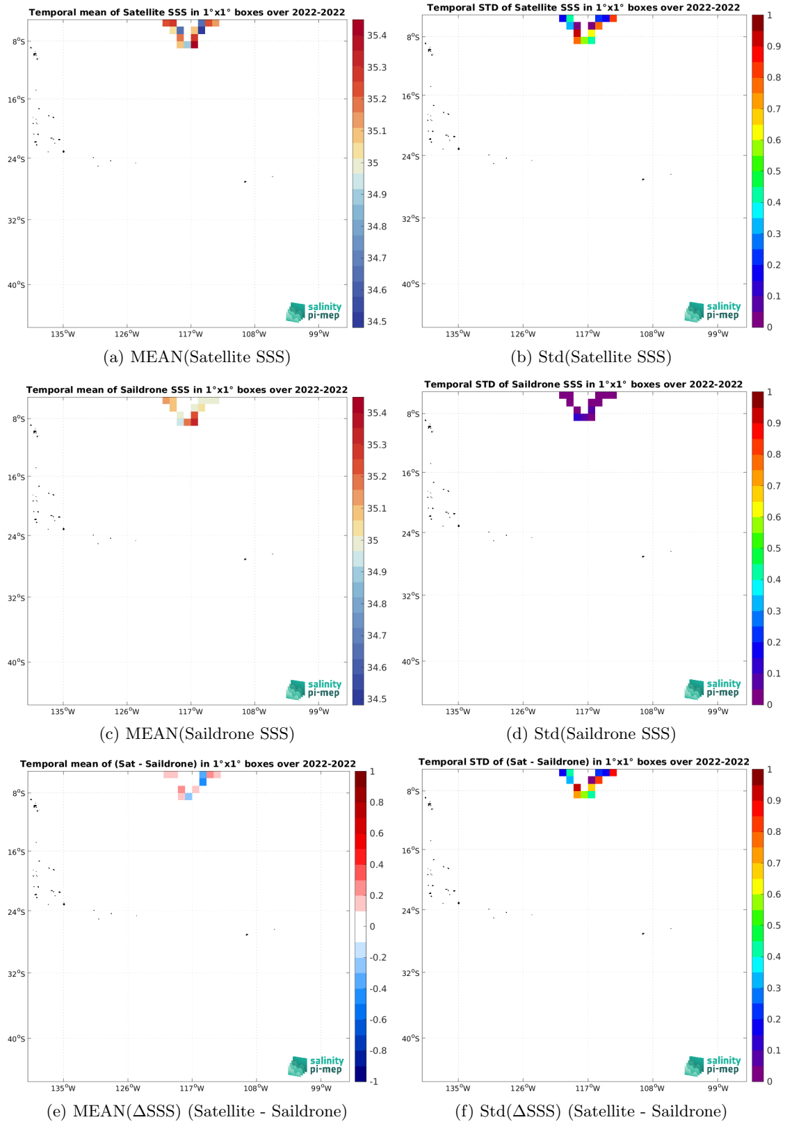
Figure 7: Temporal mean (left) and Std (right) of SSS from SMAP SSS L2 v6 - 40 km (RSS) (top), Saildrone (middle), and of \Delta SSS (Satellite - Saildrone). Only match-up pairs are used to generate these maps.
