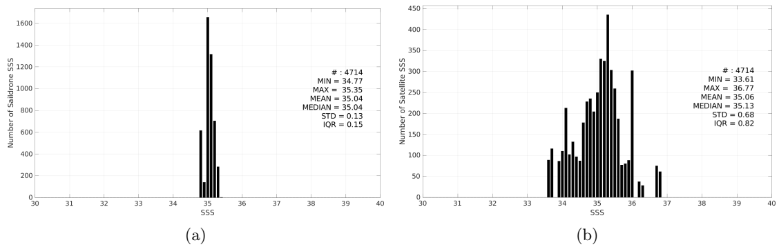
Figure 3: Histograms of SSS from Saildrone (a) and SMAP SSS L2 v6 - 40 km (RSS) (b) considering all match-up pairs per bins of 0.1 over the OTT zone Pi-MEP region and for the full satellite product period.
