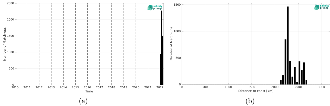
Figure 2: Number of match-ups between Saildrone and SMAP SSS L2 v6 - 40 km (RSS) SSS as a function of time (a) and as function of the distance to coast (b) over the OTT zone Pi-MEP region and for the full satellite product period.
