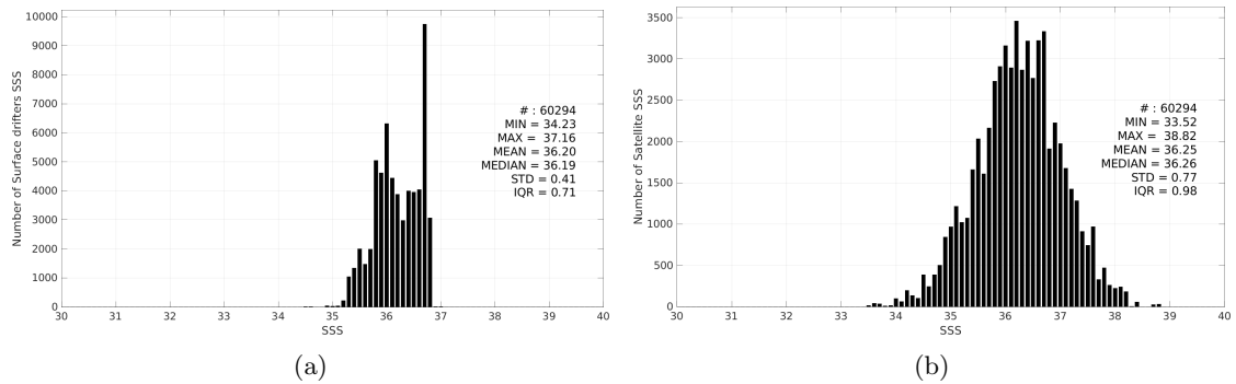
Figure 3: Histograms of SSS from Surface drifters (a) and SMAP SSS L2 v6 - 40 km (RSS) (b) considering all match-up pairs per bins of 0.1 over the OTT zone Pi-MEP region and for the full satellite product period.
