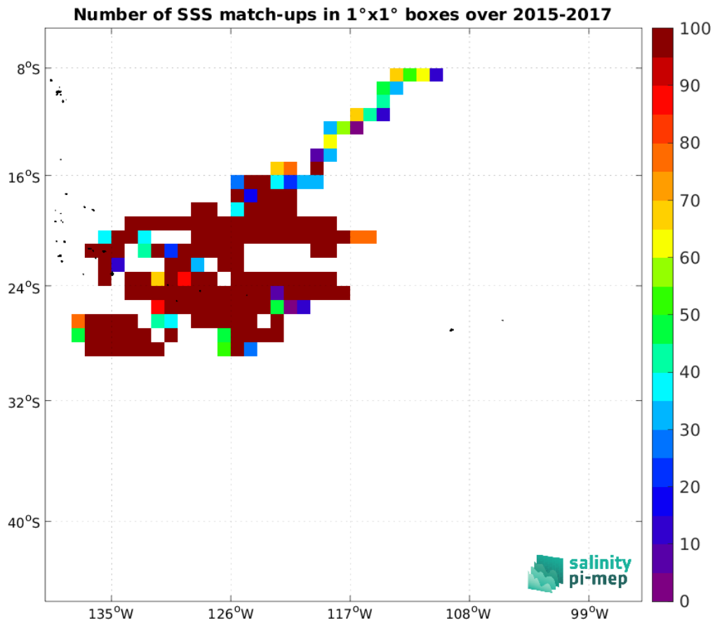
Figure 4: Number of SSS match-ups between Surface drifters SSS and the SMAP SSS L2 v6 - 40 km (RSS) SSS product for the OTT zone Pi-MEP region over 1°x1° boxes and for the full satellite product period.
