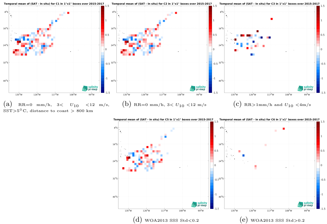
Figure 13: Temporal mean gridded over spatial boxes of size 1^\circ \times 1^\circ of \Delta SSS (SMAP SSS L2 v6 - 40 km (RSS) - Surface drifters) for 5 different subdatasets corresponding to:RR=0 mm/h, 3 < U_{10} < 12 m/s, SST >5^\circ C, distance to coast > 800 km (a), RR=0 mm/h, 3 < U_{10} < 12 m/s (b), RR >1 mm/h and U_{10} < 4 m/s (c), WOA2013 SSS Std <0.2 (d), WOA2013 SSS Std >0.2 (e).
