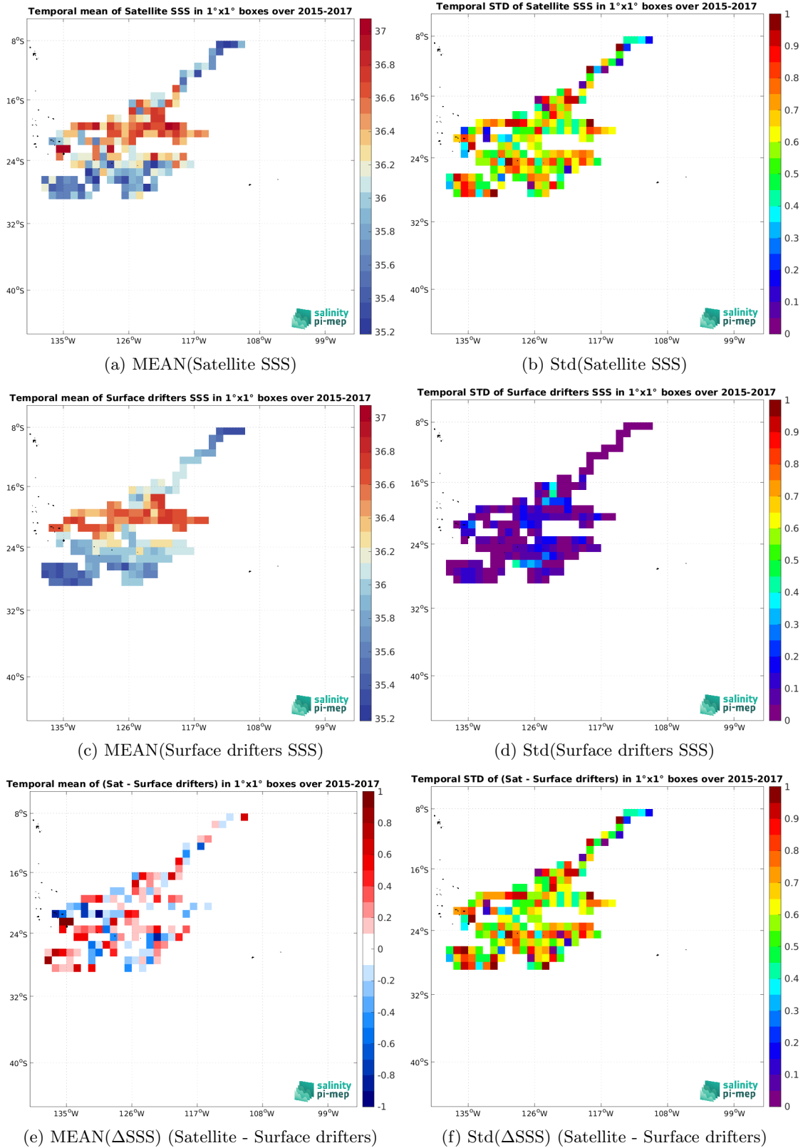
Figure 6: Temporal mean (left) and Std (right) of SSS from SMAP SSS L2 v6 - 40 km (RSS) (top), Surface drifters (middle), and of \Delta SSS (Satellite - Surface drifters). Only match-up pairs are used to generate these maps.
