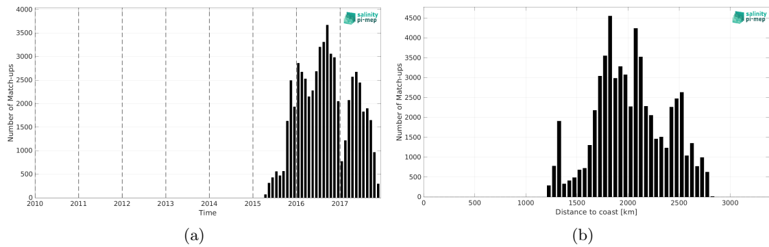
Figure 2: Number of match-ups between Surface drifters and SMAP SSS L2 v6 - 40 km (RSS) SSS as a function of time (a) and as function of the distance to coast (b) over the OTT zone Pi-MEP region and for the full satellite product period.
