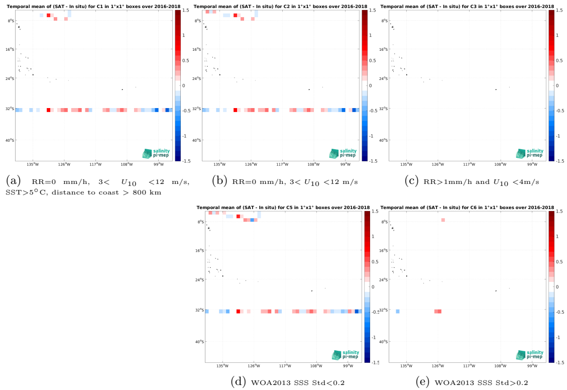
Figure 12: Temporal mean gridded over spatial boxes of size 1^\circ \times 1^\circ of \Delta SSS (SMAP SSS L2 v5 (RSS) - TSG (SAMOS)) for 5 different subdatasets corresponding to: RR=0 mm/h, 3 < U_{10} < 12 m/s, SST > 5^\circ C , distance to coast > 800 km (a), RR=0 mm/h, 3 < U_{10} < 12 m/s (b), RR > 1 mm/h and U_{10} < 4 m/s (c), WOA2013 SSS Std < 0.2 (d), WOA2013 SSS Std > 0.2 (e).
