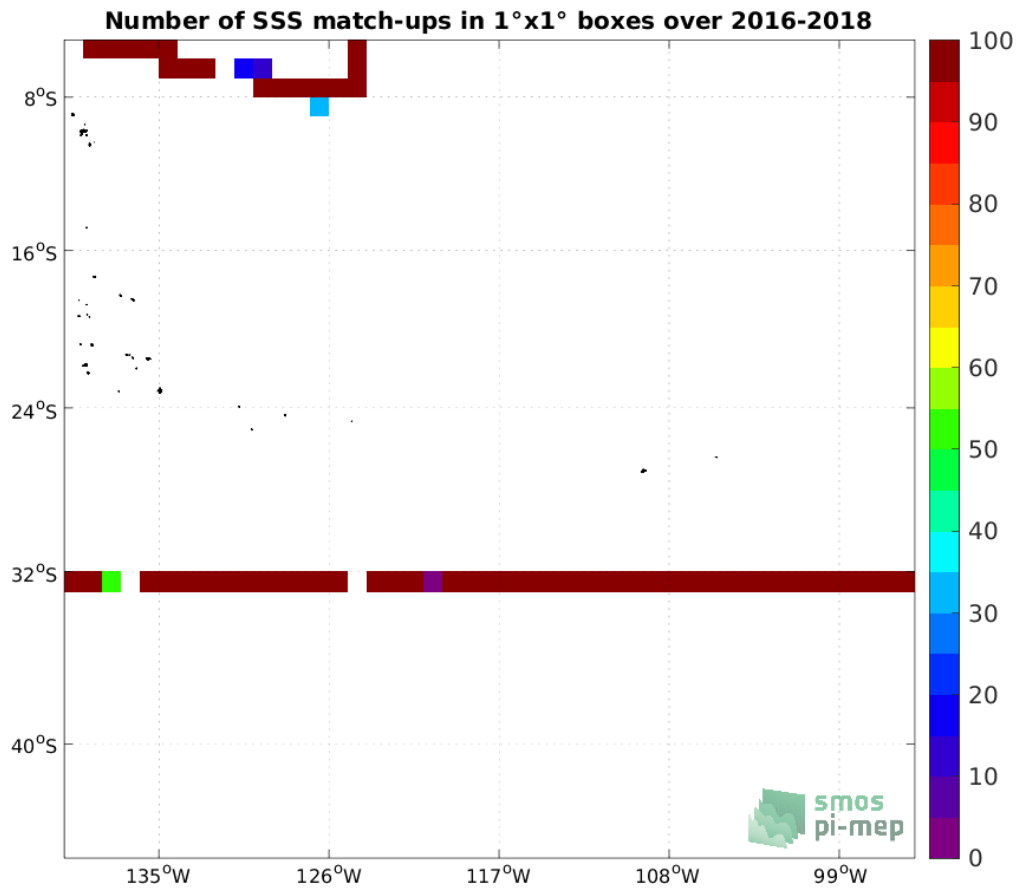
Figure 4: Number of SSS match-ups between TSG (SAMOS) SSS and the SMAP SSS L2 v5 (RSS) SSS product for the OTT zone Pi-MEP region over 1^\circ \times 1^\circ boxes and for the full satellite product period.
