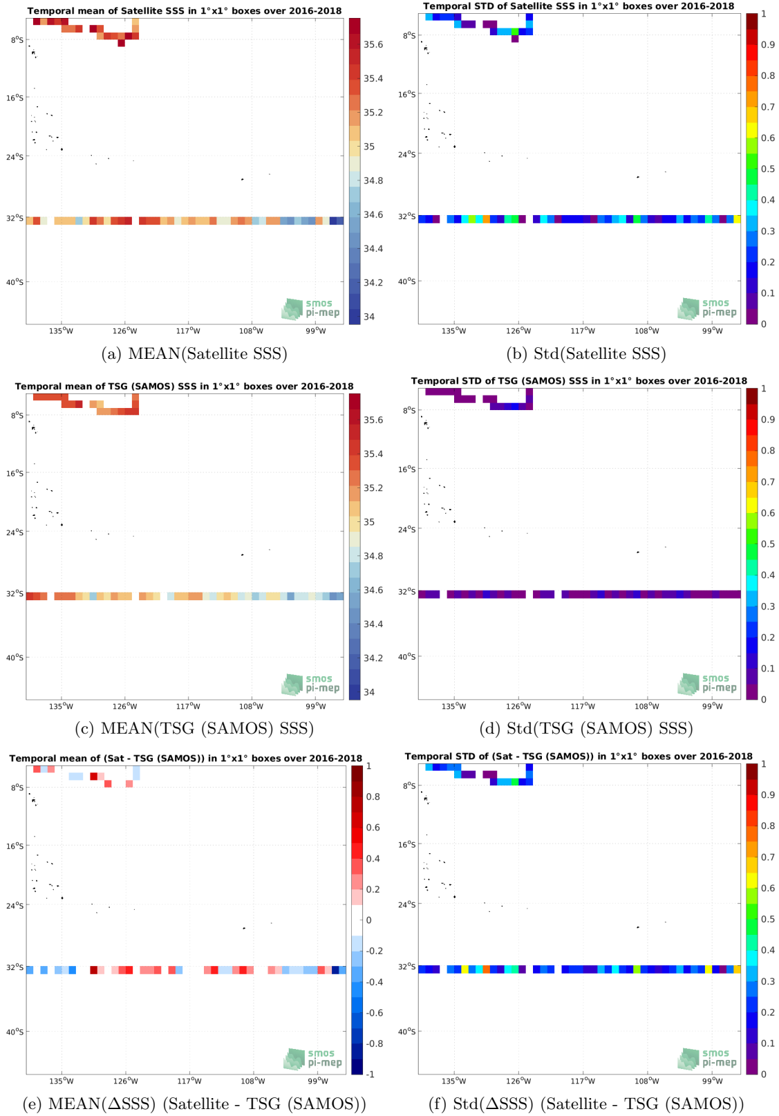
Figure 6: Temporal mean (left) and Std (right) of SSS from SMAP SSS L2 v5 (RSS) (top), TSG (SAMOS) (middle), and of \Delta SSS (Satellite - TSG (SAMOS)). Only match-up pairs are used to generate these maps.
