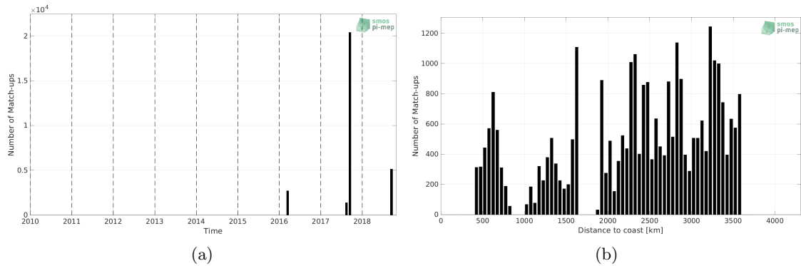
Figure 1: Number of match-ups between TSG (SAMOS) and SMAP SSS L2 v5 (RSS) SSS as a function of time (a) and as function of the distance to coast (b) over the OTT zone Pi-MEP region and for the full satellite product period.
