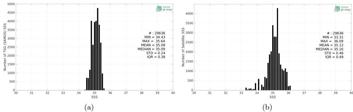
Figure 2: Histograms of SSS from TSG (SAMOS) (a) and SMAP SSS L2 v5 (RSS) (b) considering all match-up pairs per bins of 0.1 over the OTT zone Pi-MEP region and for the full satellite product period.
