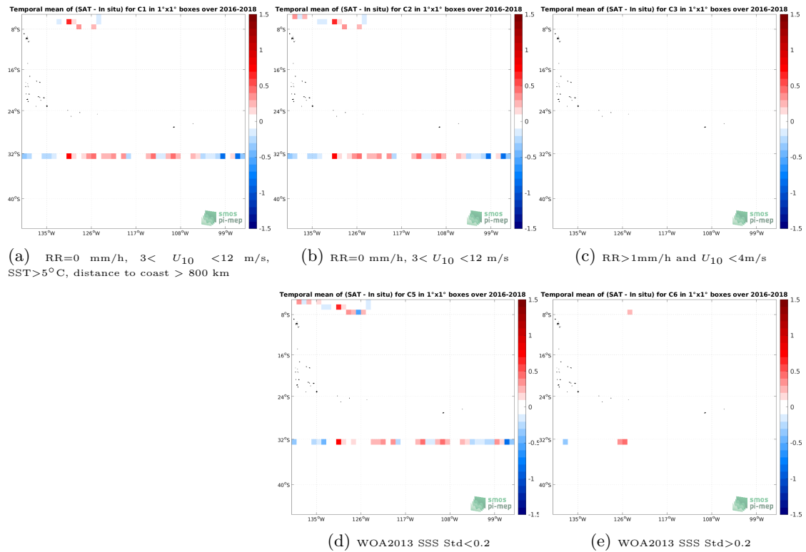
Figure 12: Temporal mean gridded over spatial boxes of size 1^\circ \times 1^\circ of \Delta SSS (SMAP SSS L2 v5 (RSS) - TSG (SAMOS)) for 5 different subdatasets corresponding to: RR=0 mm/h, 3 < U_{10} < 12 m/s, SST > 5^\circ C , distance to coast > 800 km (a), RR=0 mm/h, 3 < U_{10} < 12 m/s (b), RR > 1 mm/h and U_{10} < 4 m/s (c), WOA2013 SSS Std < 0.2 (d), WOA2013 SSS Std > 0.2 (e).
