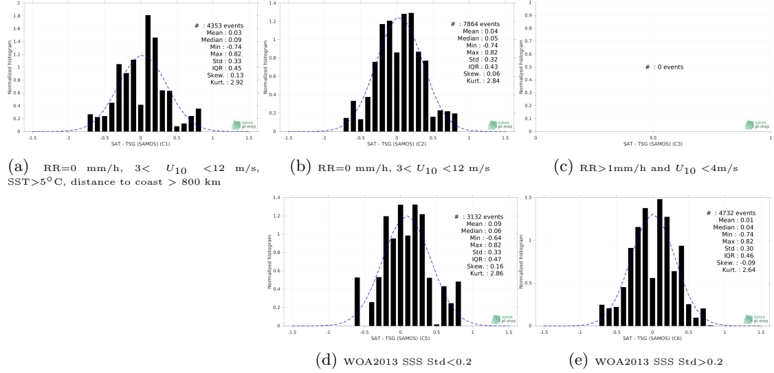
Figure 13: Normalized histogram of \Delta SSS (SMAP SSS L2 v5 (RSS) - TSG (SAMOS)) for 5 different subdatasets corresponding to: RR=0 mm/h, 3 < U_{10} < 12 m/s, SST > 5°C, distance to coast > 800 km (a), RR=0 mm/h, 3 < U_{10} < 12 m/s (b), RR > 1mm/h and U_{10} < 4 m/s (c), WOA2013 SSS Std < 0.2 (d), WOA2013 SSS Std > 0.2 (e).
