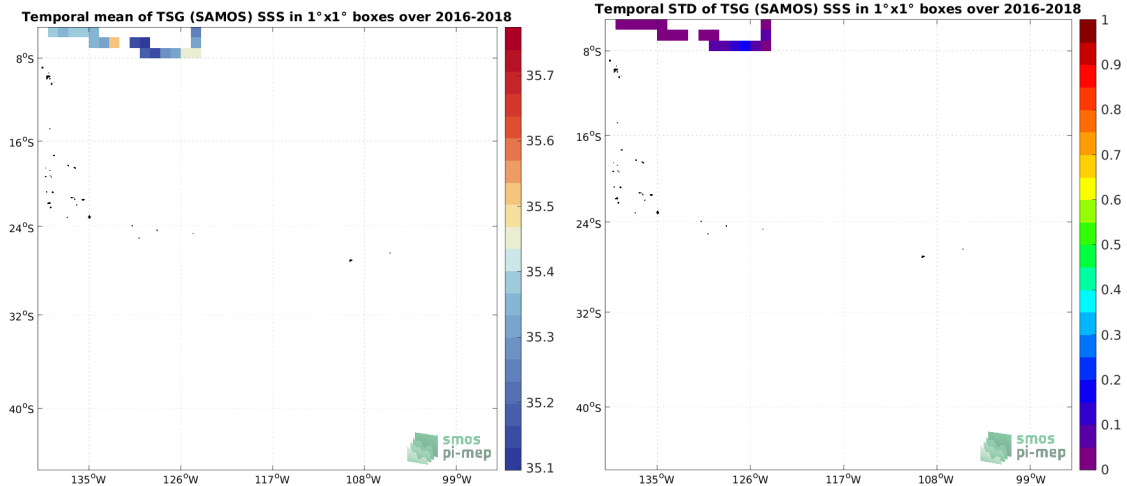
(c) MEAN(TSG (SAMOS) SSS)
