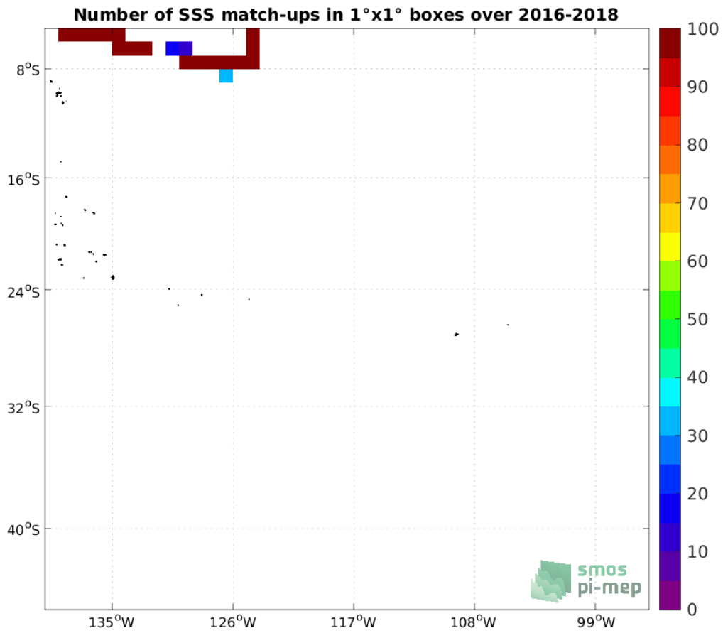
Figure 4: Number of SSS match-ups between TSG (SAMOS) SSS and the SMAP SSS L2 v5 (RSS) SSS product for the OTT zone Pi-MEP region over 1°x1° boxes and for the full satellite product period.
