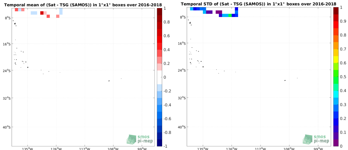
(e) MEAN( \Delta SSS) (Satellite - TSG (SAMOS))
