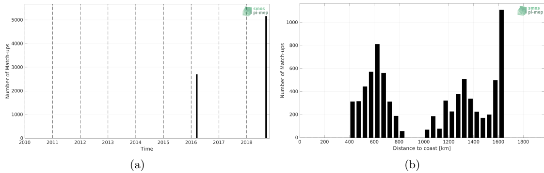
Figure 1: Number of match-ups between TSG (SAMOS) and SMAP SSS L2 v5 (RSS) SSS as a function of time (a) and as function of the distance to coast (b) over the OTT zone Pi-MEP region and for the full satellite product period.
