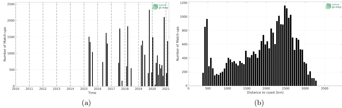
Figure 1: Number of match-ups between TSG (LEGOS-DM) and SMAP SSS L2 v5 (RSS) SSS as a function of time (a) and as function of the distance to coast (b) over the OTT zone Pi-MEP region and for the full satellite product period.
