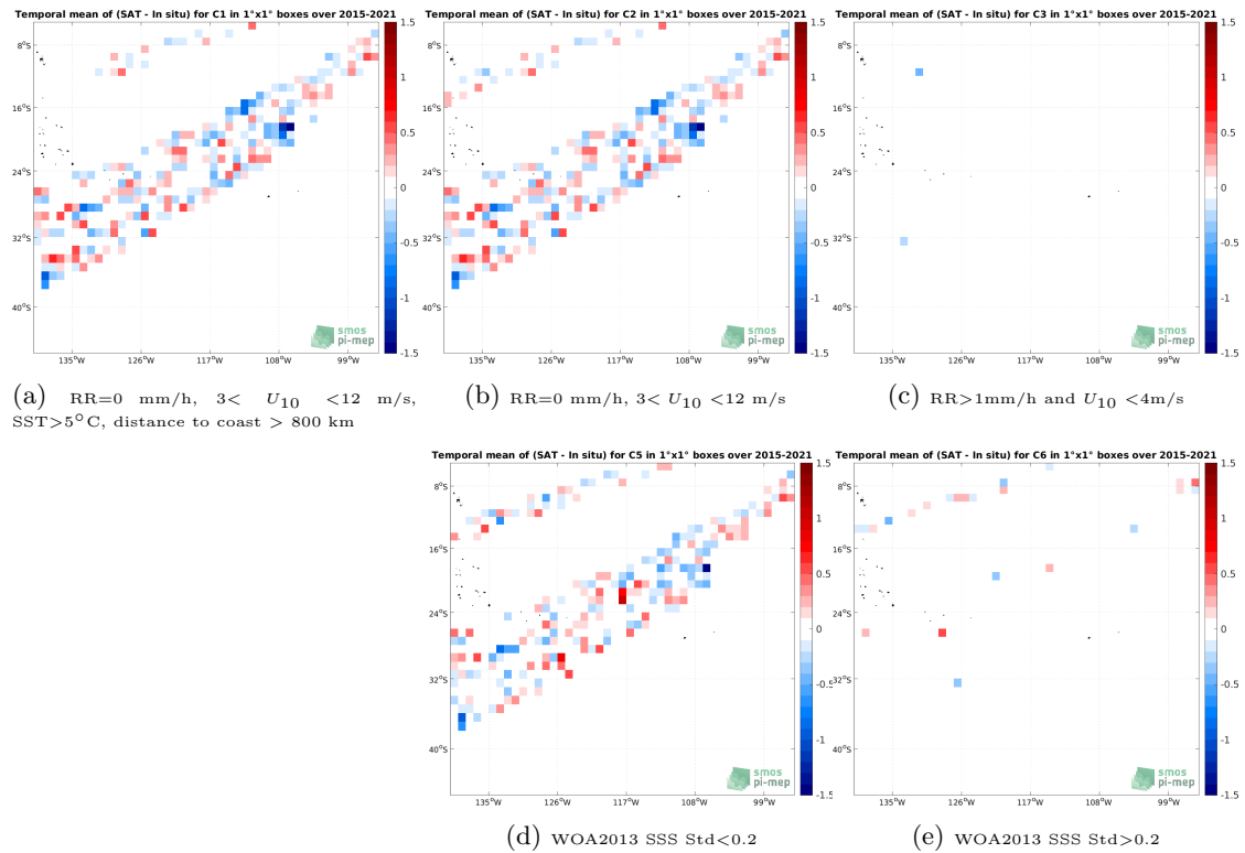
Figure 12: Temporal mean gridded over spatial boxes of size 1^\circ \times 1^\circ of \Delta SSS (SMAP SSS L2 v5 (RSS) - TSG (LEGOS-DM)) for 5 different subdatasets corresponding to: RR=0 mm/h, 3 < U_{10} < 12 m/s, SST > 5^\circ C , distance to coast > 800 km (a), RR=0 mm/h, 3 < U_{10} < 12 m/s (b), RR > 1 mm/h and U_{10} < 4 m/s (c), WOA2013 SSS Std < 0.2 (d), WOA2013 SSS Std > 0.2 (e).
