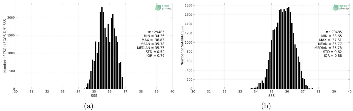
Figure 2: Histograms of SSS from TSG (LEGOS-DM) (a) and SMAP SSS L2 v5 (RSS) (b) considering all match-up pairs per bins of 0.1 over the OTT zone Pi-MEP region and for the full satellite product period.
