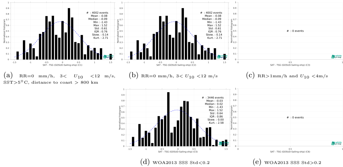
Figure 13: Normalized histogram of \Delta\text{SSS} (SMAP SSS L2 v5 (RSS) - TSG (GOSUD-Sailing-ship)) for 5 different subdatasets corresponding to: RR=0 mm/h, 3 < U_{10} < 12 m/s, SST > 5^\circ\text{C} , distance to coast > 800 km (a), RR=0 mm/h, 3 < U_{10} < 12 m/s (b), RR > 1\text{mm/h} and U_{10} < 4\text{m/s} (c), WOA2013 SSS \text{Std} < 0.2 (d), WOA2013 SSS \text{Std} > 0.2 (e).
