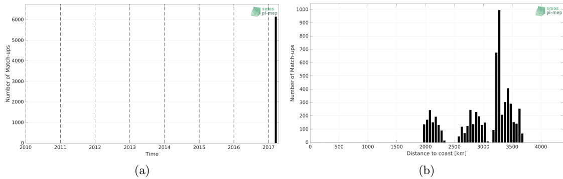
Figure 1: Number of match-ups between TSG (GOSUD-Sailing-ship) and SMAP SSS L2 v5 (RSS) SSS as a function of time (a) and as function of the distance to coast (b) over the OTT zone Pi-MEP region and for the full satellite product period.
