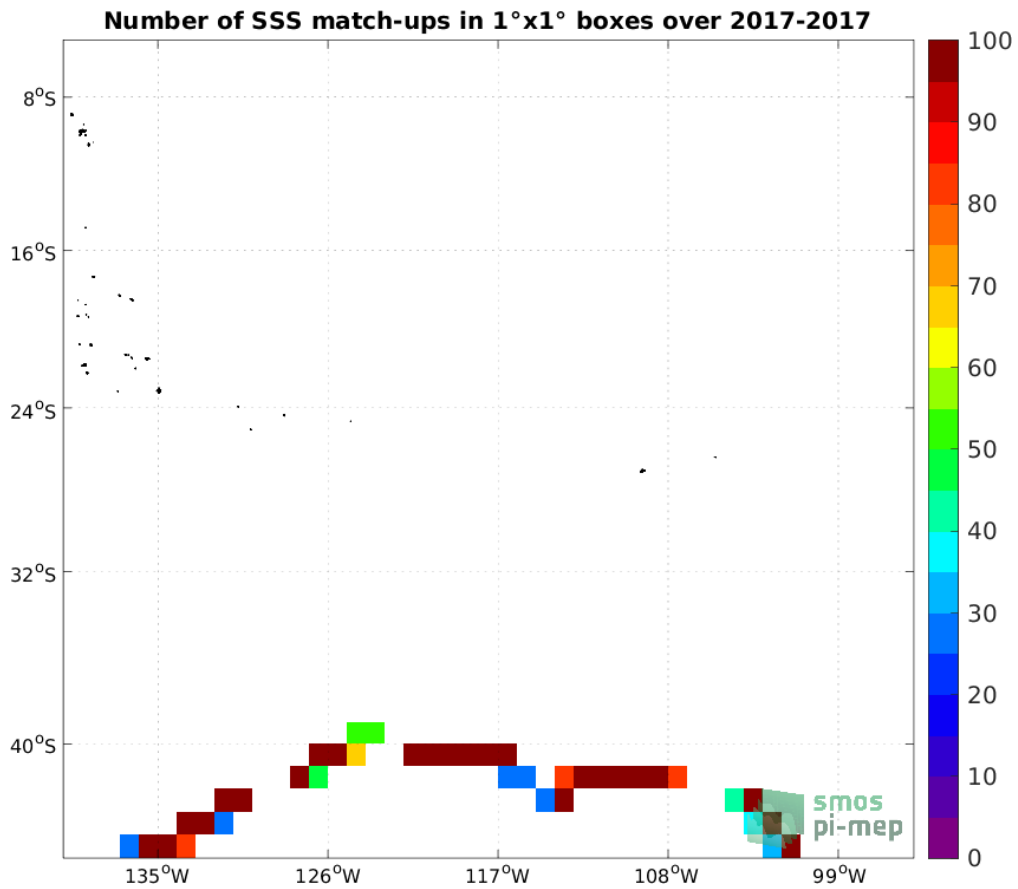
Figure 4: Number of SSS match-ups between TSG (GOSUD-Sailing-ship) SSS and the SMAP SSS L2 v5 (RSS) SSS product for the OTT zone Pi-MEP region over 1°×1° boxes and for the full satellite product period.
