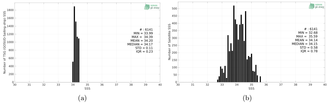
Figure 2: Histograms of SSS from TSG (GOSUD-Sailing-ship) (a) and SMAP SSS L2 v5 (RSS) (b) considering all match-up pairs per bins of 0.1 over the OTT zone Pi-MEP region and for the full satellite product period.
