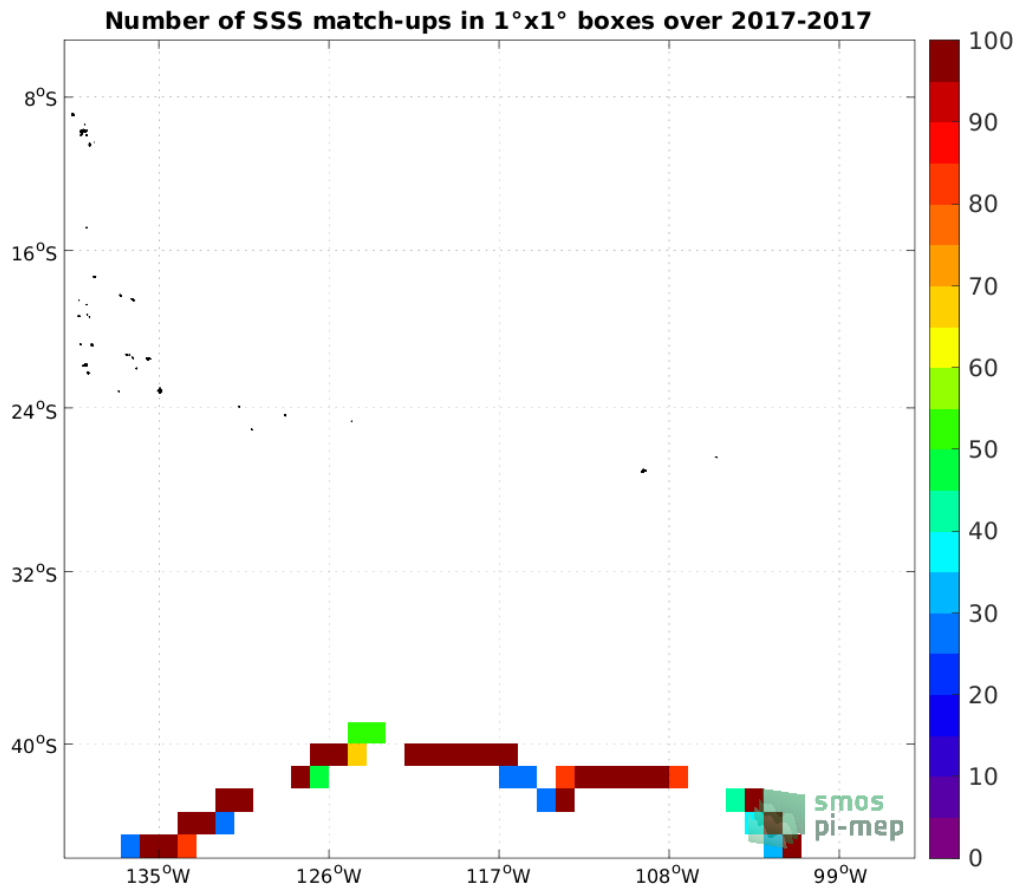
Figure 4: Number of SSS match-ups between TSG (GOSUD-Sailing-ship) SSS and the SMAP SSS L2 v5 (RSS) SSS product for the OTT zone Pi-MEP region over 1^\circ \times 1^\circ boxes and for the full satellite product period.
