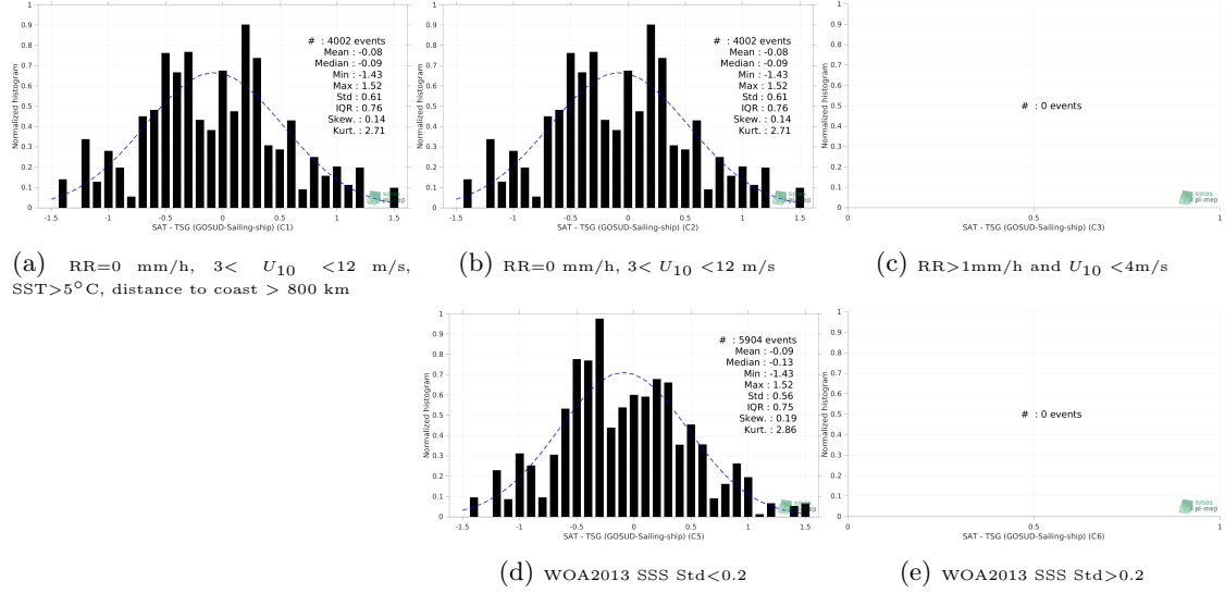
Figure 13: Normalized histogram of \Delta SSS (SMAP SSS L2 v5 (RSS) - TSG (GOSUD-Sailing-ship)) for 5 different subdatasets corresponding to: RR=0 mm/h, 3 < U_{10} < 12 m/s, SST>5°C, distance to coast > 800 km (a), RR=0 mm/h, 3 < U_{10} < 12 m/s (b), RR>1mm/h and U_{10} < 4 m/s (c), WOA2013 SSS Std<0.2 (d), WOA2013 SSS Std>0.2 (e).
