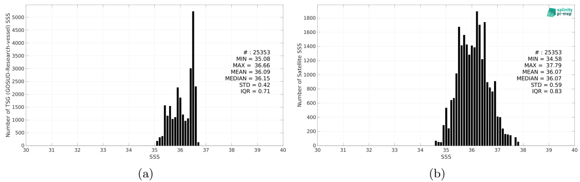
Figure 2: Histograms of SSS from TSG (GOSUD-Research-vessel) (a) and SMAP SSS L2 v5 (RSS) (b) considering all match-up pairs per bins of 0.1 over the OTT zone Pi-MEP region and for the full satellite product period.
