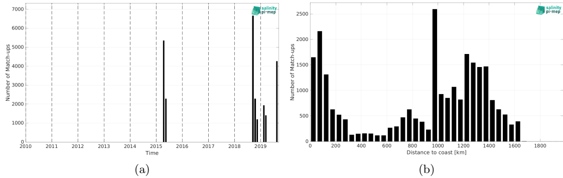
Figure 1: Number of match-ups between TSG (GOSUD-Research-vessel) and SMAP SSS L2 v5 (RSS) SSS as a function of time (a) and as function of the distance to coast (b) over the OTT zone Pi-MEP region and for the full satellite product period.
