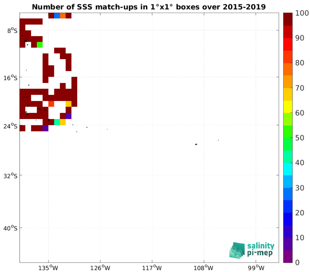
Figure 4: Number of SSS match-ups between TSG (GOSUD-Research-vessel) SSS and the SMAP SSS L2 v5 (RSS) SSS product for the OTT zone Pi-MEP region over 1°×1° boxes and for the full satellite product period.
