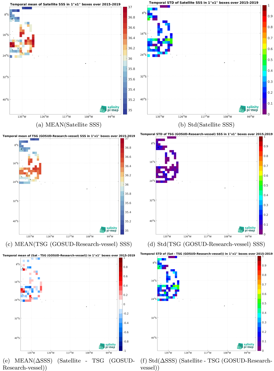
Figure 6: Temporal mean (left) and Std (right) of SSS from SMAP SSS L2 v5 (RSS) (top), TSG (GOSUD-Research-vessel) (middle), and of \Delta SSS (Satellite - TSG (GOSUD-Research-vessel)). Only match-up pairs are used to generate these maps.
