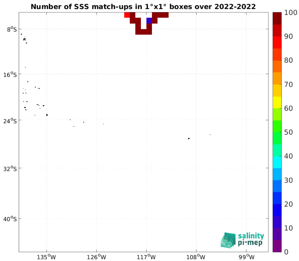
Figure 4: Number of SSS match-ups between Saildrone SSS and the SMAP SSS L2 v5 (RSS) SSS product for the OTT zone Pi-MEP region over 1°x1° boxes and for the full satellite product period.
