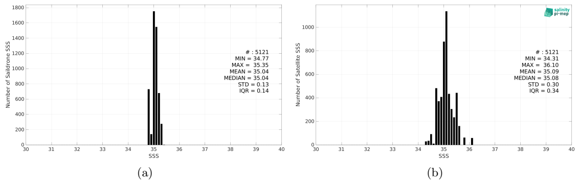
Figure 2: Histograms of SSS from Saildrone (a) and SMAP SSS L2 v5 (RSS) (b) considering all match-up pairs per bins of 0.1 over the OTT zone Pi-MEP region and for the full satellite product period.
