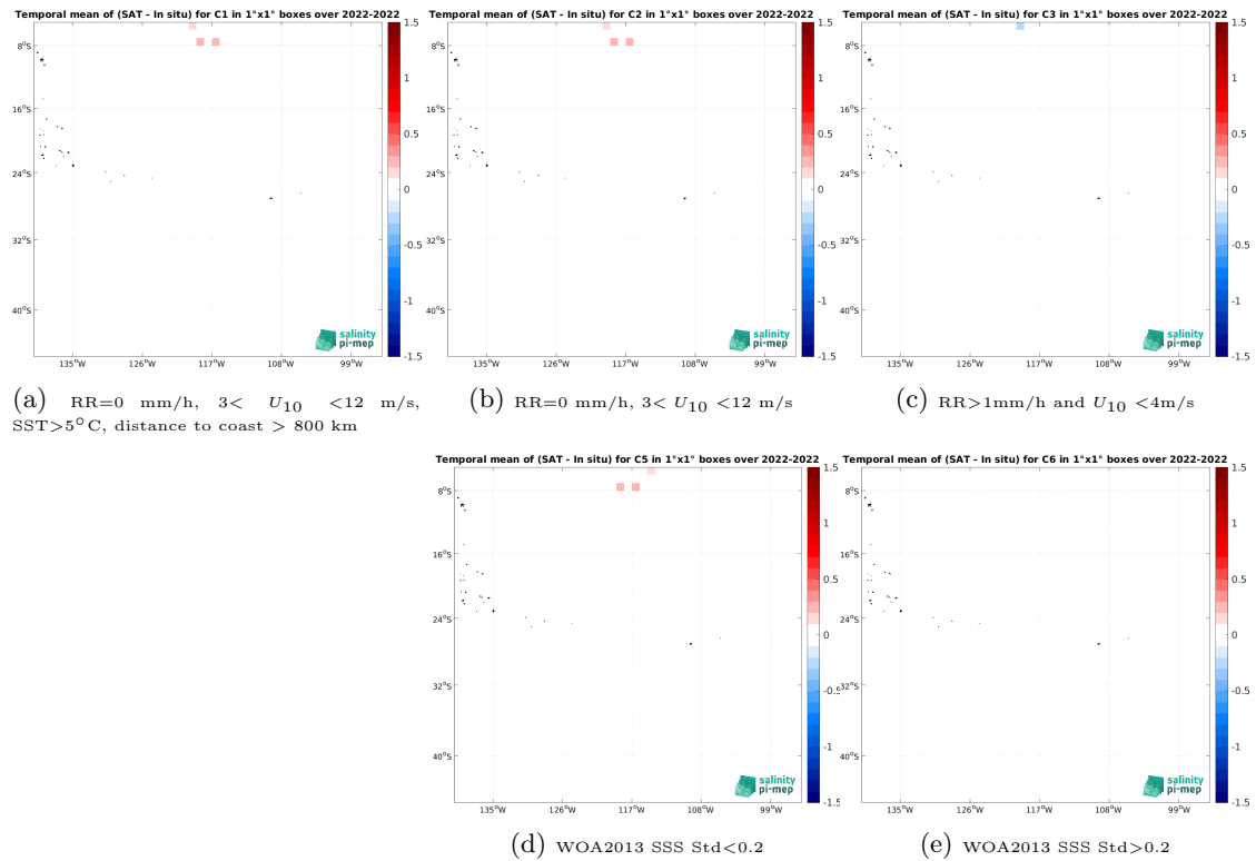
Figure 12: Temporal mean gridded over spatial boxes of size 1^\circ \times 1^\circ of \Delta SSS (SMAP SSS L2 v5 (RSS) - Saicdrone) for 5 different subdatasets corresponding to: RR=0 mm/h, 3 < U_{10} < 12 m/s, SST > 5^\circ C , distance to coast > 800 km (a), RR=0 mm/h, 3 < U_{10} < 12 m/s (b), RR > 1 mm/h and U_{10} < 4 m/s (c), WOA2013 SSS Std < 0.2 (d), WOA2013 SSS Std > 0.2 (e).
