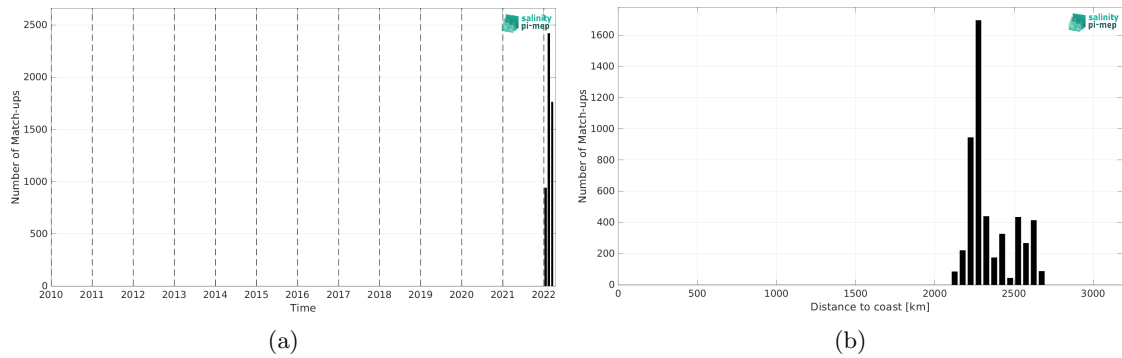
Figure 1: Number of match-ups between Saildrone and SMAP SSS L2 v5 (RSS) SSS as a function of time (a) and as function of the distance to coast (b) over the OTT zone Pi-MEP region and for the full satellite product period.
