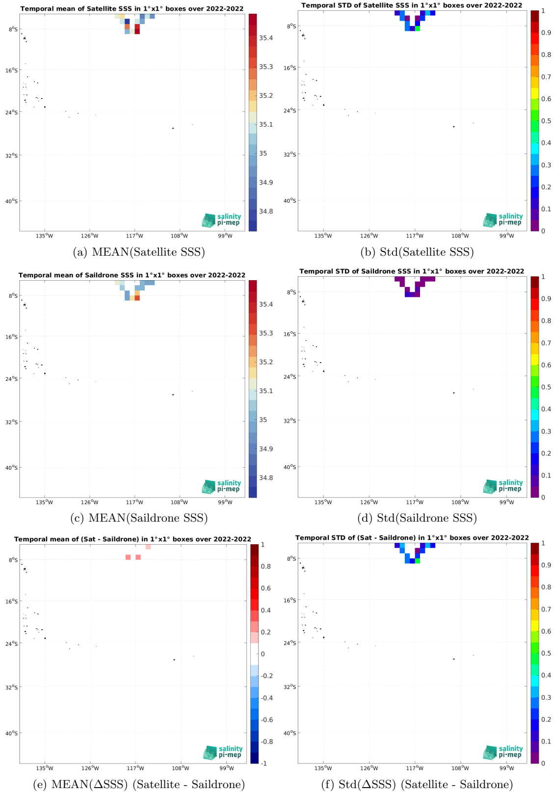
Figure 6: Temporal mean (left) and Std (right) of SSS from SMAP SSS L2 v5 (RSS) (top), Saildrone (middle), and of \Delta SSS (Satellite - Saildrone). Only match-up pairs are used to generate these maps.
