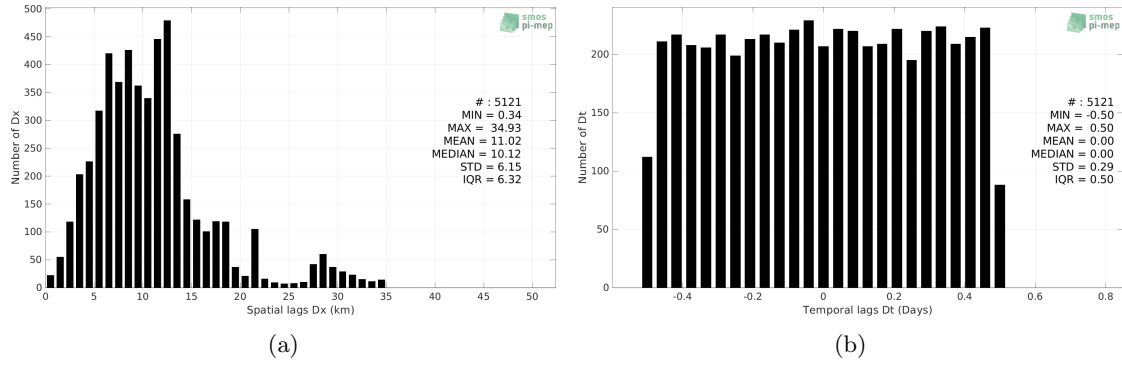
Figure 5: Histograms of the spatial (a) and temporal (b) lags between the location/time of the Sailldrone measurement and the date of the corresponding SMAP SSS L2 v5 (RSS) SSS pixel.
