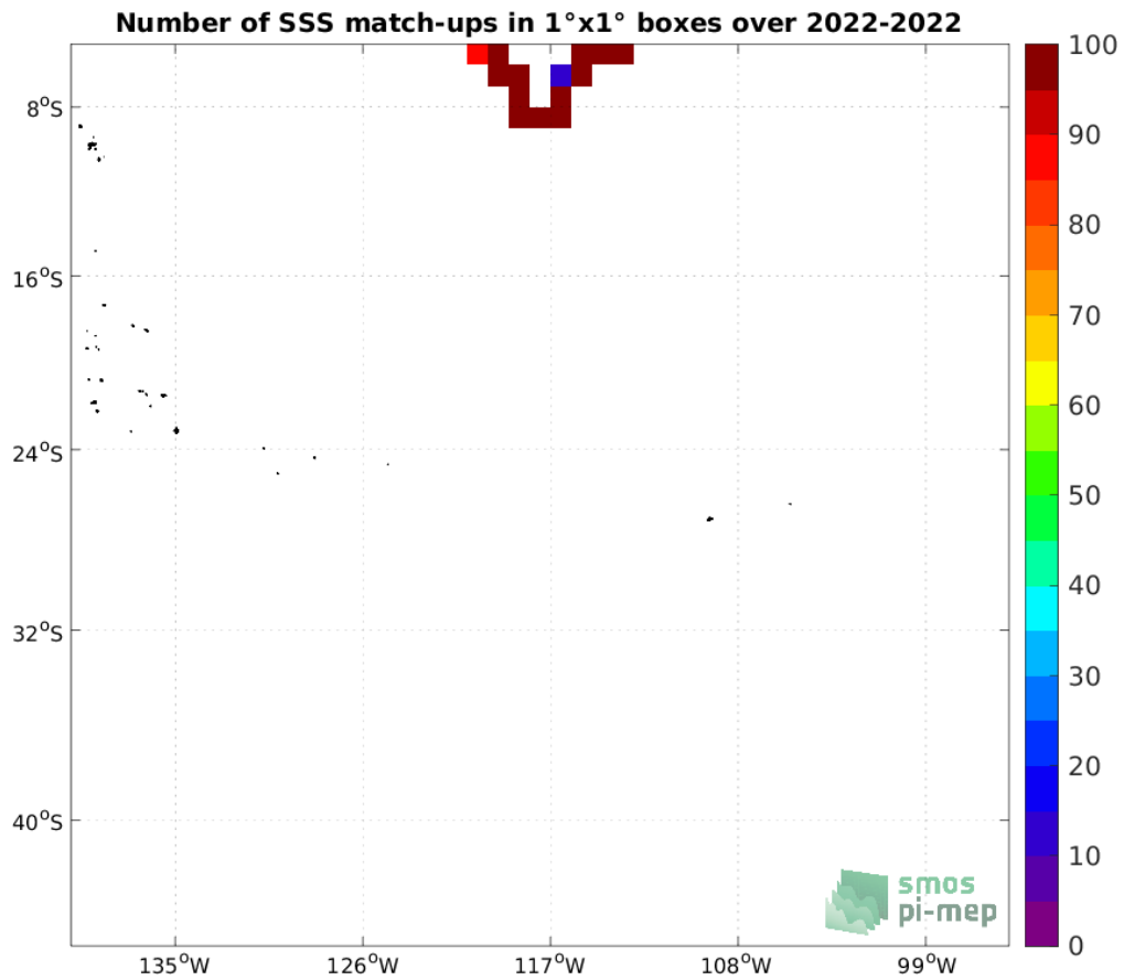
Figure 4: Number of SSS match-ups between Saildrone SSS and the SMAP SSS L2 v5 (RSS) SSS product for the OTT zone Pi-MEP region over 1^\circ \times 1^\circ boxes and for the full satellite product period.
