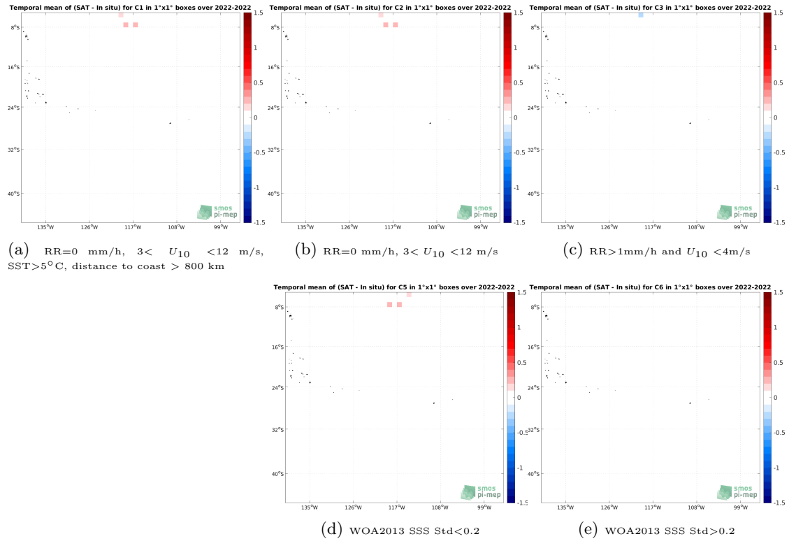
Figure 12: Temporal mean gridded over spatial boxes of size 1^\circ \times 1^\circ of \Delta SSS (SMAP SSS L2 v5 (RSS) - Saifdrone) for 5 different subdatasets corresponding to:RR=0 mm/h, 3 < U_{10} < 12 m/s, SST >5^\circ C, distance to coast > 800 km (a), RR=0 mm/h, 3 < U_{10} < 12 m/s (b), RR >1 mm/h and U_{10} < 4 m/s (c), WOA2013 SSS Std <0.2 (d), WOA2013 SSS Std >0.2 (e).
