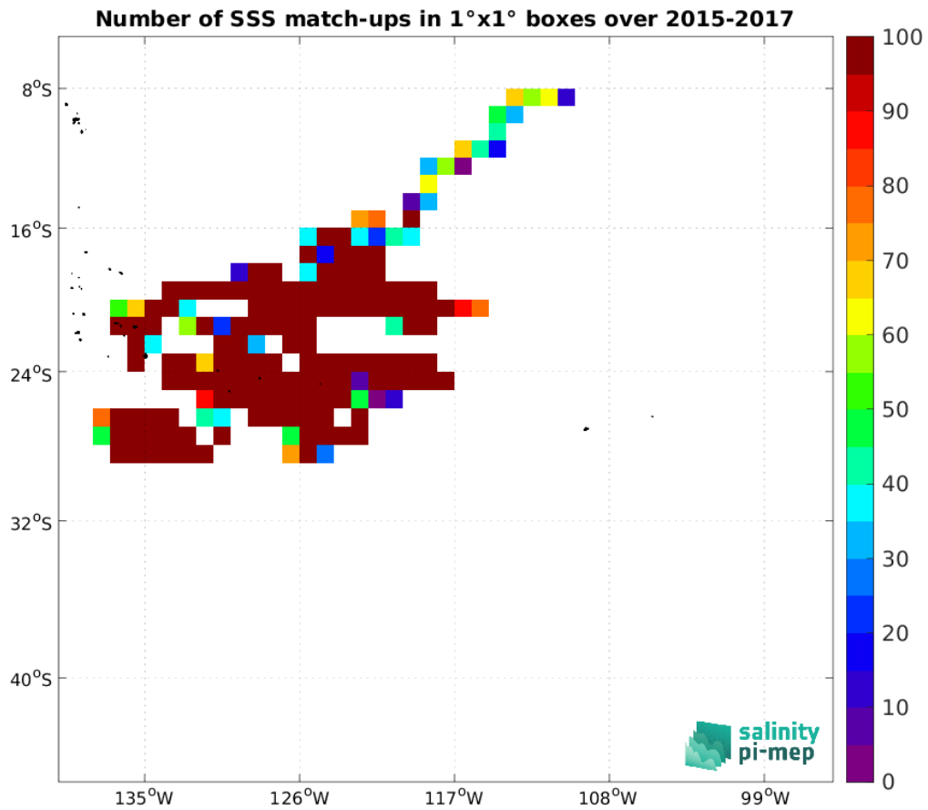
Figure 3: Number of SSS match-ups between Surface drifters SSS and the SMAP SSS L2 v5 (RSS) SSS product for the OTT zone Pi-MEP region over 1°x1° boxes and for the full satellite product period.
