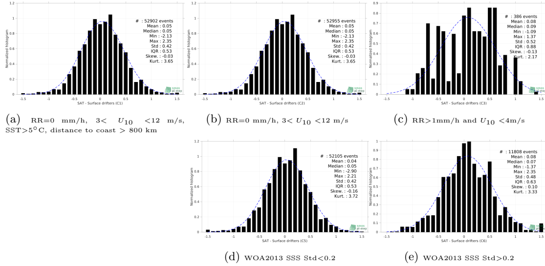
Figure 12: Normalized histogram of \Delta\text{SSS} (SMAP SSS L2 v5 (RSS) - Surface drifters) for 5 different subdatasets corresponding to: RR=0 mm/h, 3 < U_{10} < 12 m/s, SST>5°C, distance to coast > 800 km (a), RR=0 mm/h, 3 < U_{10} < 12 m/s (b), RR>1mm/h and U_{10} < 4 m/s (c), WOA2013 SSS Std<0.2 (d), WOA2013 SSS Std>0.2 (e).
