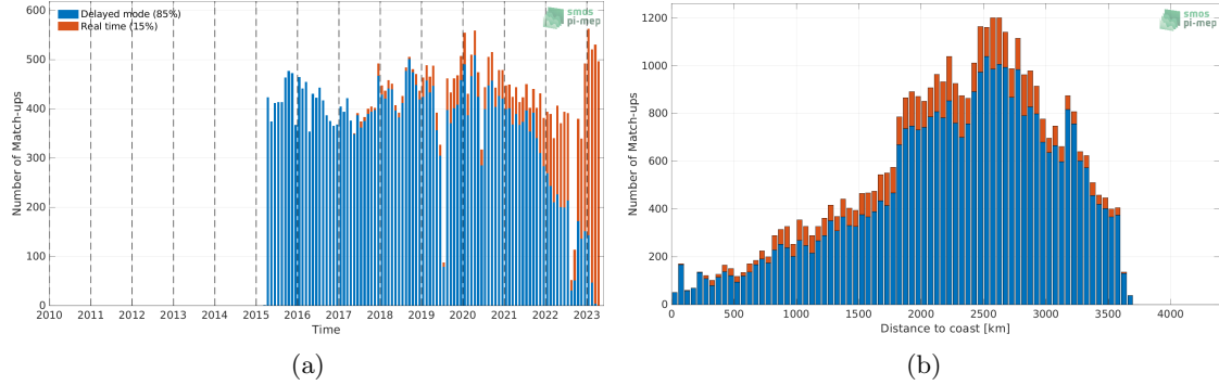
Figure 1: Number of match-ups between Argo and SMAP SSS L2 v5 (RSS) SSS as a function of time (a) and as function of the distance to coast (b) over the OTT zone Pi-MEP region and for the full satellite product period.
