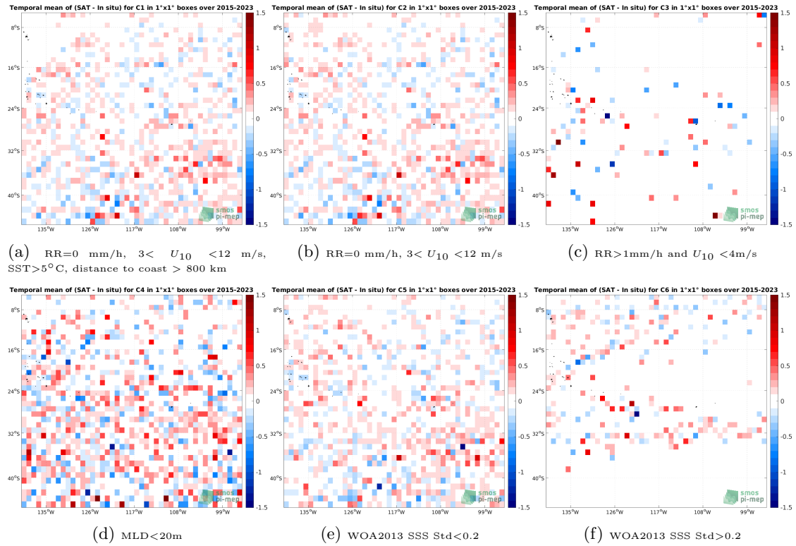
Figure 12: Temporal mean gridded over spatial boxes of size 1^\circ \times 1^\circ of \Delta SSS (SMAP SSS L2 v5 (RSS) - Argo) for 6 different subdatasets corresponding to:RR=0 mm/h, 3 < U_{10} < 12 m/s, SST >5^\circ C, distance to coast > 800 km (a), RR=0 mm/h, 3 < U_{10} < 12 m/s (b), RR >1 mm/h and U_{10} < 4 m/s (c),MLD <20 m (d),WOA2013 SSS Std <0.2 (e),WOA2013 SSS Std >0.2 (f).
