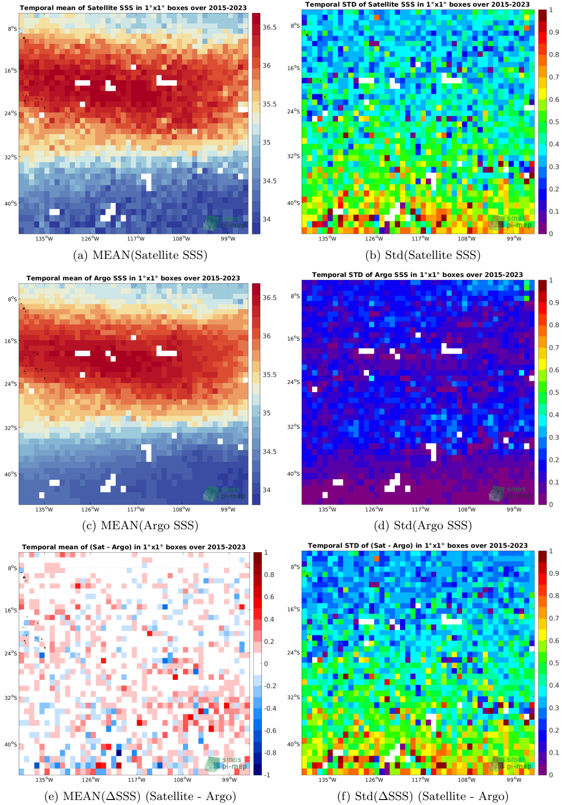
Figure 6: Temporal mean (left) and Std (right) of SSS from SMAP SSS L2 v5 (RSS) (top), Argo (middle), and of \Delta SSS (Satellite - Argo). Only match-up pairs are used to generate these maps.
