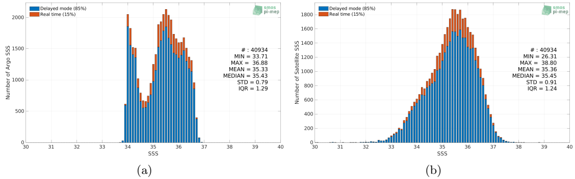
Figure 2: Histograms of SSS from Argo (a) and SMAP SSS L2 v5 (RSS) (b) considering all match-up pairs per bins of 0.1 over the OTT zone Pi-MEP region and for the full satellite product period.
