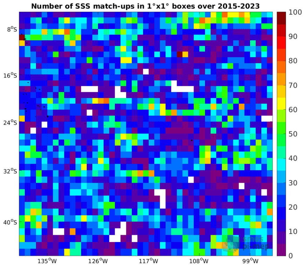
Figure 4: Number of SSS match-ups between Argo SSS and the SMAP SSS L2 v5 (RSS) SSS product for the OTT zone Pi-MEP region over 1°x1° boxes and for the full satellite product period.
