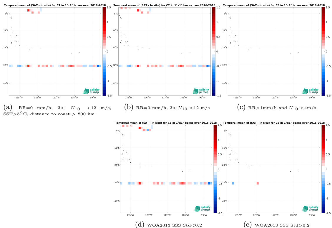
Figure 14: Temporal mean gridded over spatial boxes of size 1^\circ \times 1^\circ of \Delta\text{SSS} (SMAP SSS L2 v5.3 (RSS) - TSG (SAMOS)) for 5 different subdatasets corresponding to: \text{RR}=0 mm/h, 3 < U_{10} < 12 m/s, \text{SST} > 5^\circ\text{C} , distance to coast > 800 km (a), \text{RR}=0 mm/h, 3 < U_{10} < 12 m/s (b), \text{RR} > 1 mm/h and U_{10} < 4 m/s (c), WOA2013 SSS Std < 0.2 (d), WOA2013 SSS Std > 0.2 (e).
