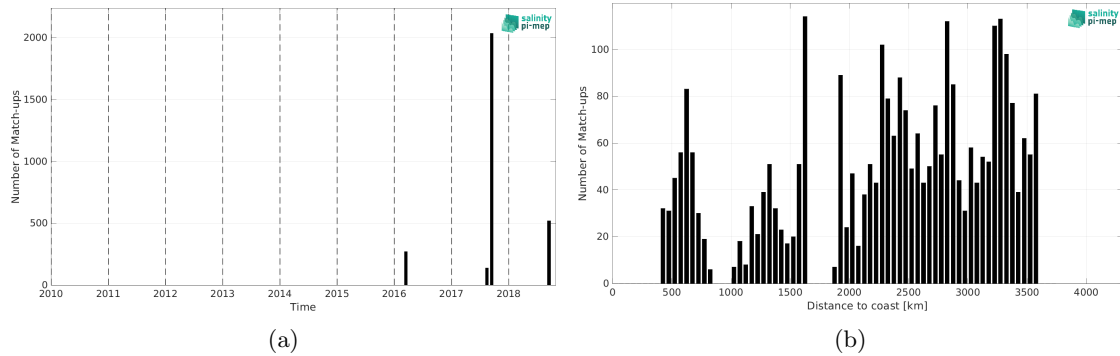
Figure 2: Number of match-ups between TSG (SAMOS) and SMAP SSS L2 v5.3 (RSS) SSS as a function of time (a) and as function of the distance to coast (b) over the OTT zone Pi-MEP region and for the full satellite product period.
