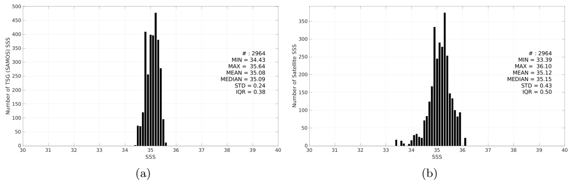
Figure 3: Histograms of SSS from TSG (SAMOS) (a) and SMAP SSS L2 v5.3 (RSS) (b) considering all match-up pairs per bins of 0.1 over the OTT zone Pi-MEP region and for the full satellite product period.
