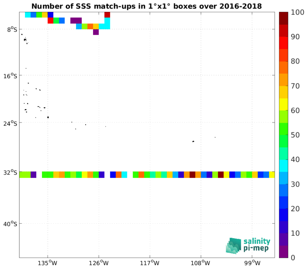
Figure 5: Number of SSS match-ups between TSG (SAMOS) SSS and the SMAP SSS L2 v5.3 (RSS) SSS product for the OTT zone Pi-MEP region over 1^\circ \times 1^\circ boxes and for the full satellite product period.
