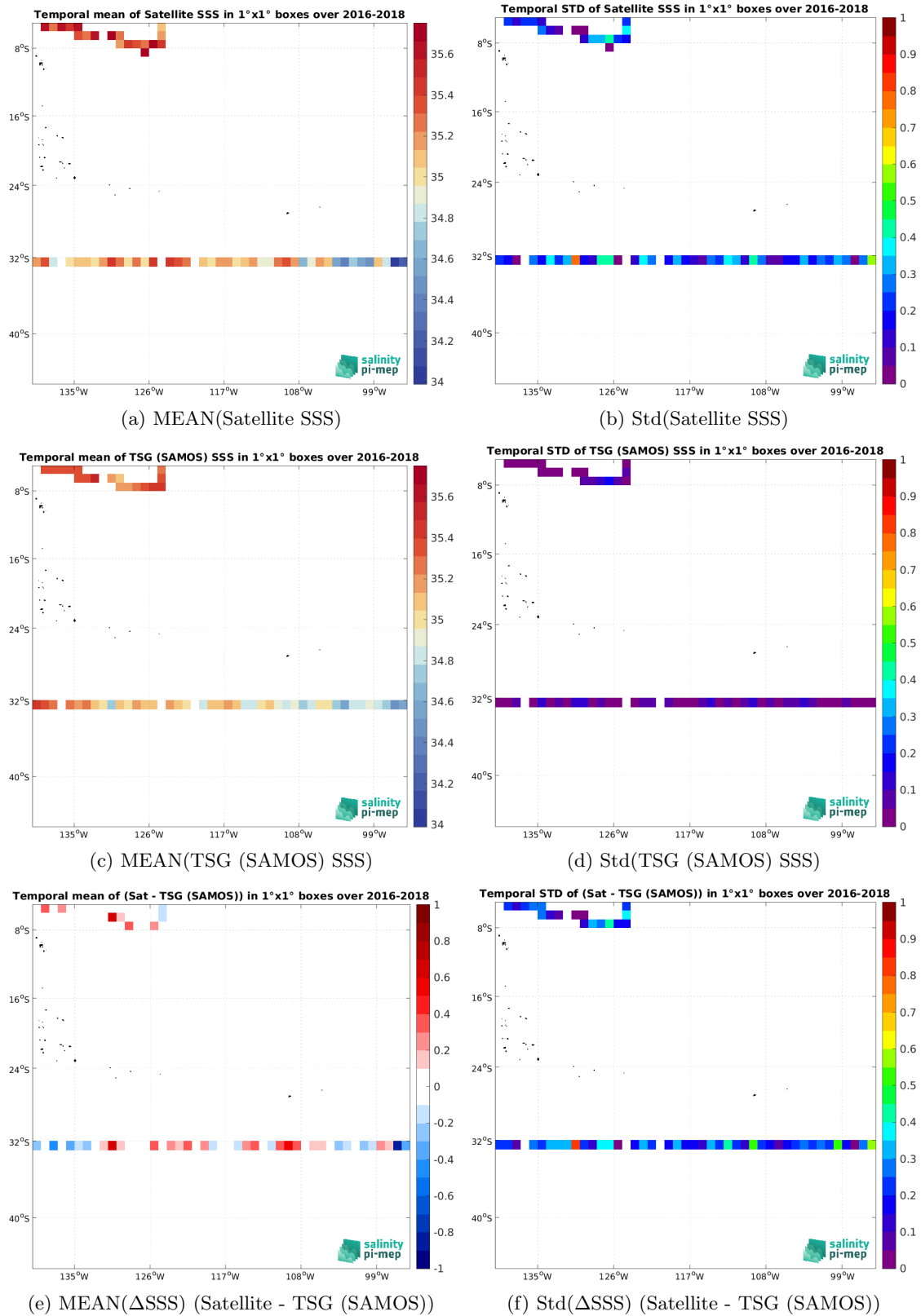
Figure 7: Temporal mean (left) and Std (right) of SSS from SMAP SSS L2 v5.3 (RSS) (top), TSG (SAMOS) (middle), and of \Delta SSS (Satellite - TSG (SAMOS)). Only match-up pairs are used to generate these maps.
