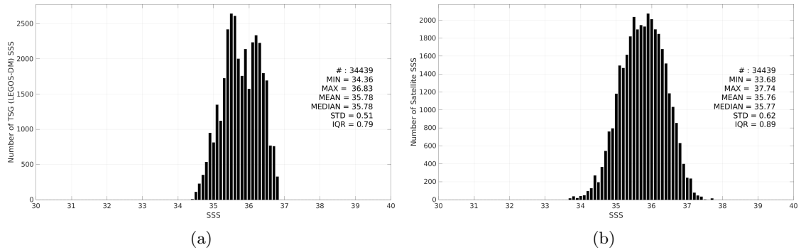
Figure 3: Histograms of SSS from TSG (LEGOS-DM) (a) and SMAP SSS L2 v5.3 (RSS) (b) considering all match-up pairs per bins of 0.1 over the OTT zone Pi-MEP region and for the full satellite product period.
