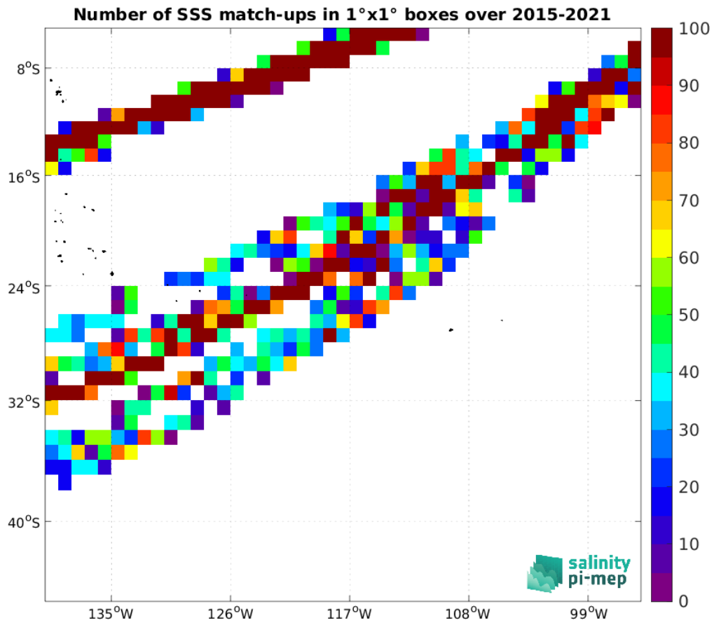
Figure 5: Number of SSS match-ups between TSG (LEGOS-DM) SSS and the SMAP SSS L2 v5.3 (RSS) SSS product for the OTT zone Pi-MEP region over 1^\circ \times 1^\circ boxes and for the full satellite product period.
