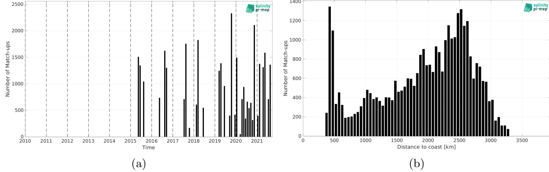
Figure 2: Number of match-ups between TSG (LEGOS-DM) and SMAP SSS L2 v5.3 (RSS) SSS as a function of time (a) and as function of the distance to coast (b) over the OTT zone Pi-MEP region and for the full satellite product period.
