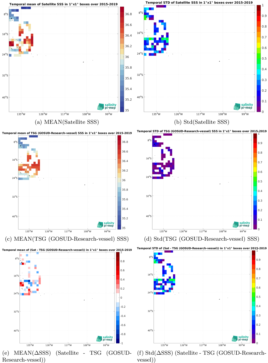
Figure 7: Temporal mean (left) and Std (right) of SSS from SMAP SSS L2 v5.3 (RSS) (top), TSG (GOSUD-Research-vessel) (middle), and of \Delta SSS (Satellite - TSG (GOSUD-Research-vessel)). Only match-up pairs are used to generate these maps.
