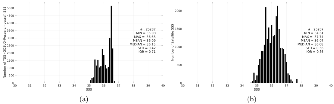
Figure 3: Histograms of SSS from TSG (GOSUD-Research-vessel) (a) and SMAP SSS L2 v5.3 (RSS) (b) considering all match-up pairs per bins of 0.1 over the OTT zone Pi-MEP region and for the full satellite product period.
